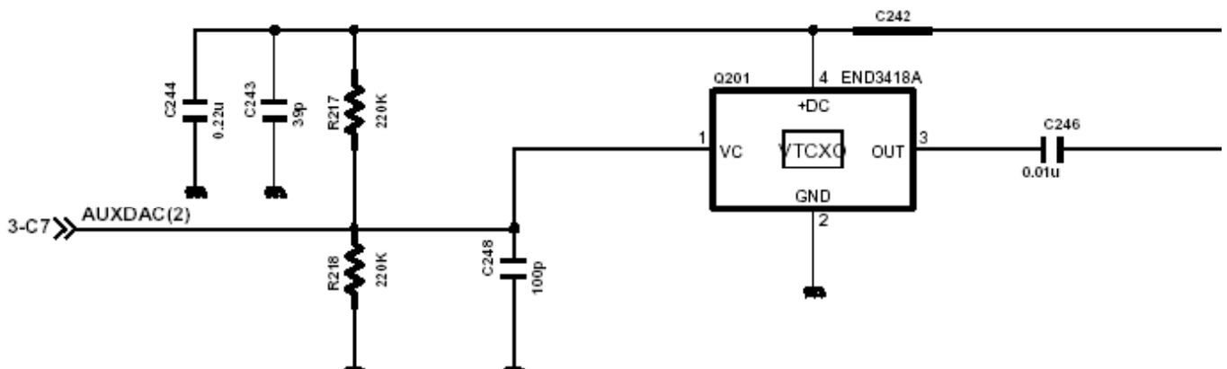
13M-crystal oscillator
