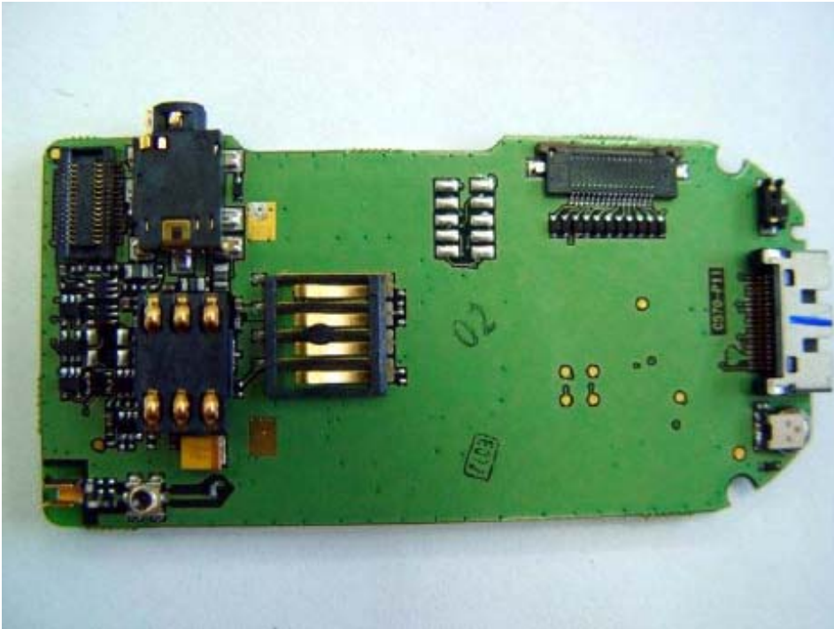
K570 – Solder View
