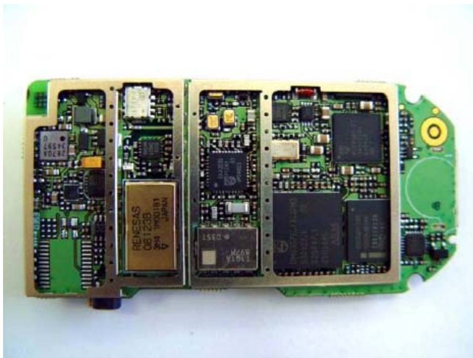
K570 – Component View
