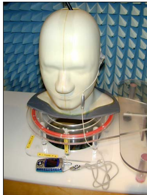
Figure 33. A Positional photograph of MX-C99 Handset Fitted Headset Fitted placed against LH Cheek
