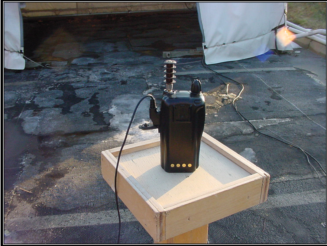
PHOTOGRAPH 3: RADIATED EMISSIONS BACK VIEW
