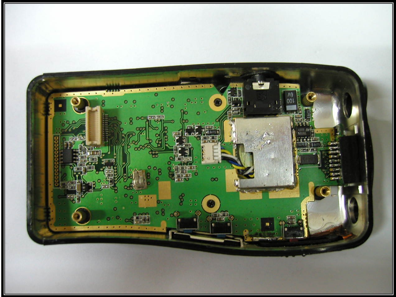
PHOTOGRAPH 12: DIGITAL PCB BACK VIEW
