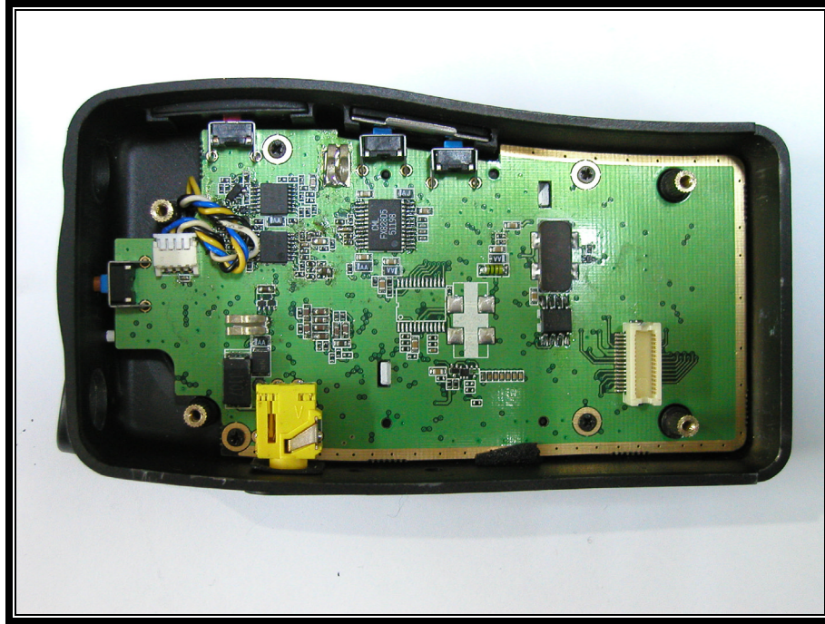
PHOTOGRAPH 10: DIGITAL PCB INSIDE BACK COVER
