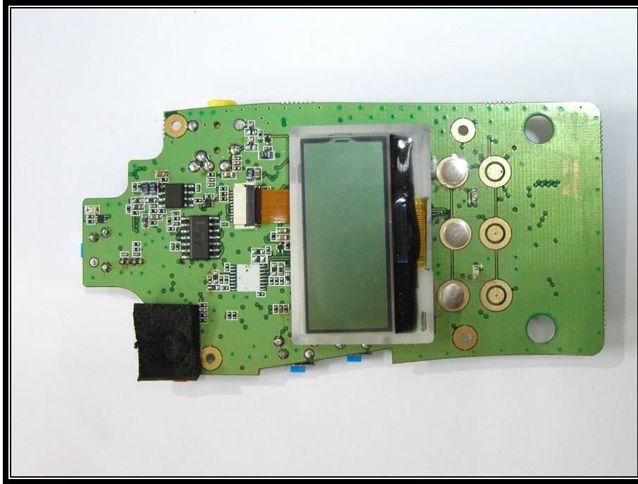
PHOTOGRAPH 11: PCB FRONT
