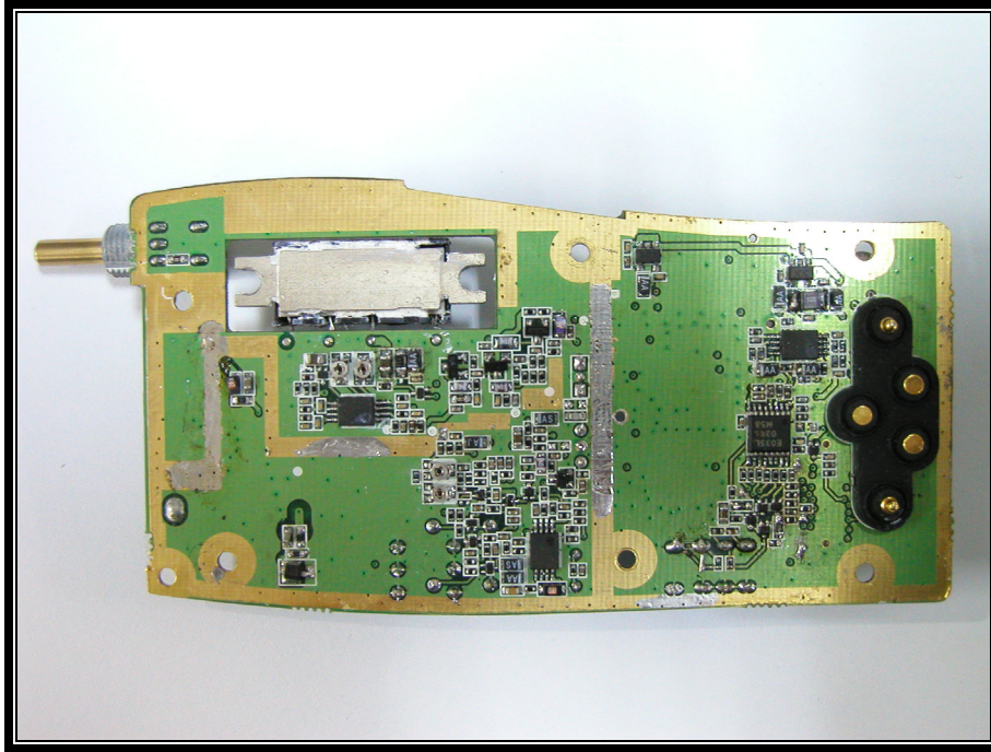
PHOTOGRAPH 12: RF PCB BACK SIDE
