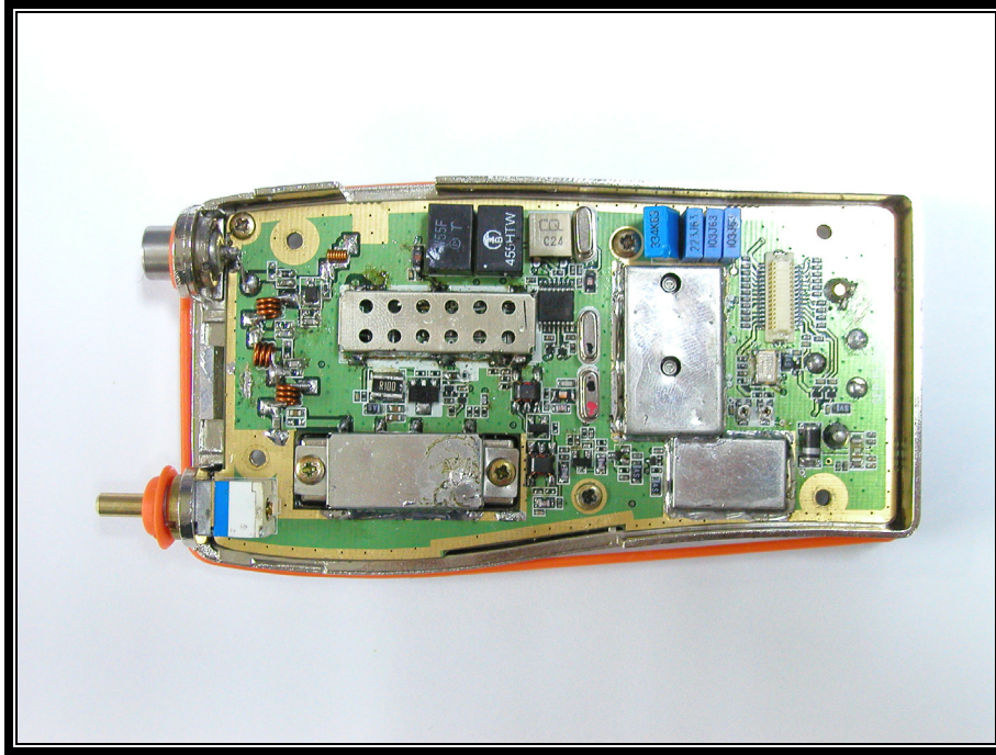
PHOTOGRAPH 13: RF PCB FRONT SIDE
