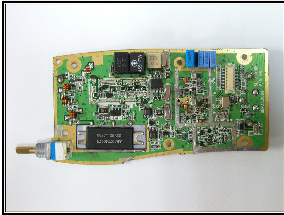
PHOTOGRAPH 14: RF PCB FRONT SIDE WITH SHIELDS REMOVED
