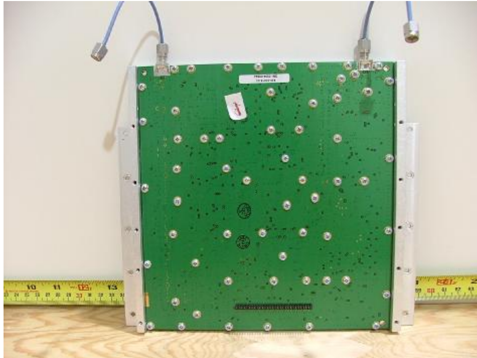
Top Heat Sink
