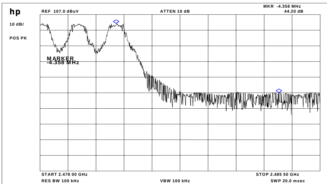
Plot 3: Marker-Delta Method (hopping)
