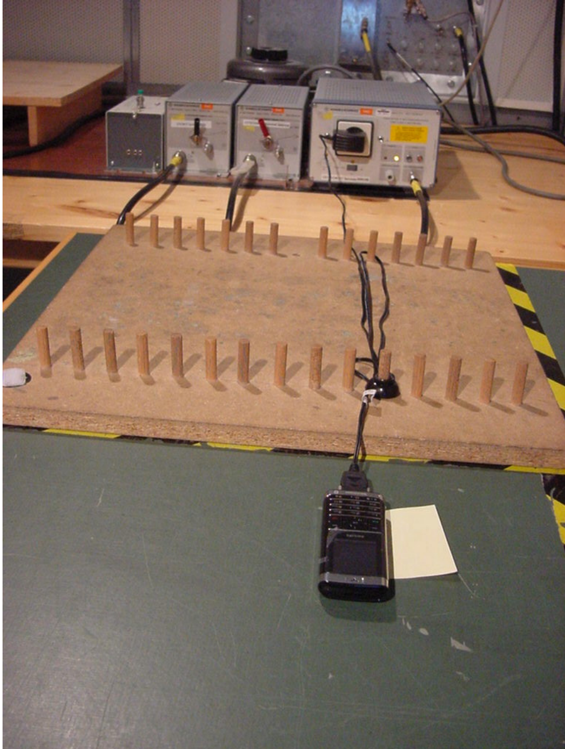
Photo 3: Conducted Emissions
