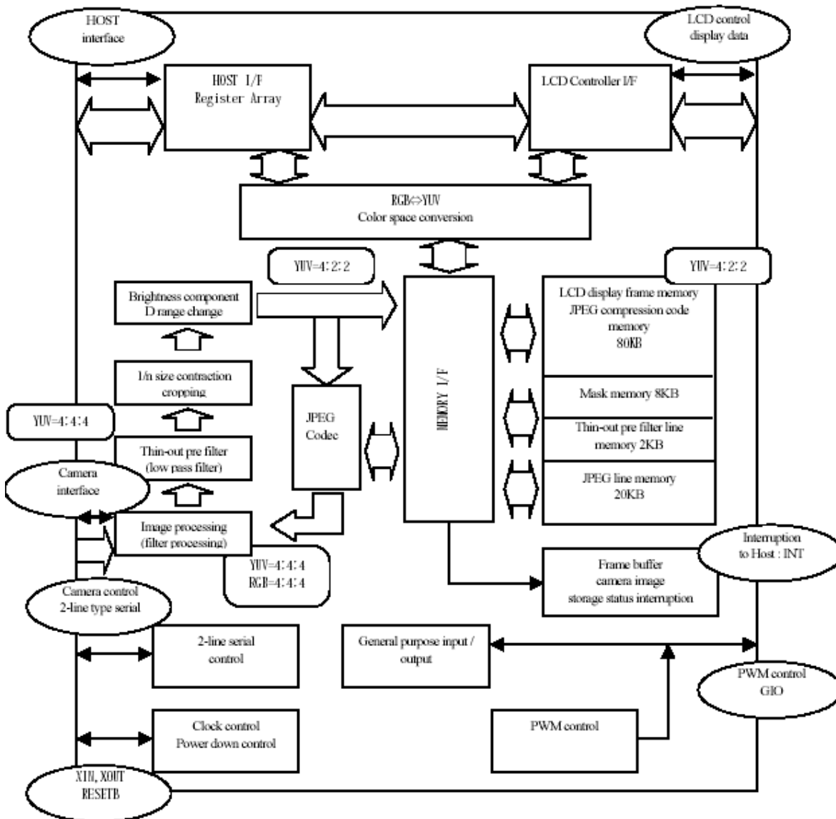
Fig.1.5-1. BU1594GS block diagram
