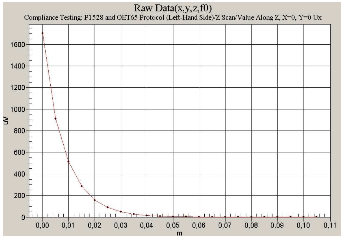
Z-scan Head 1900 MHz
