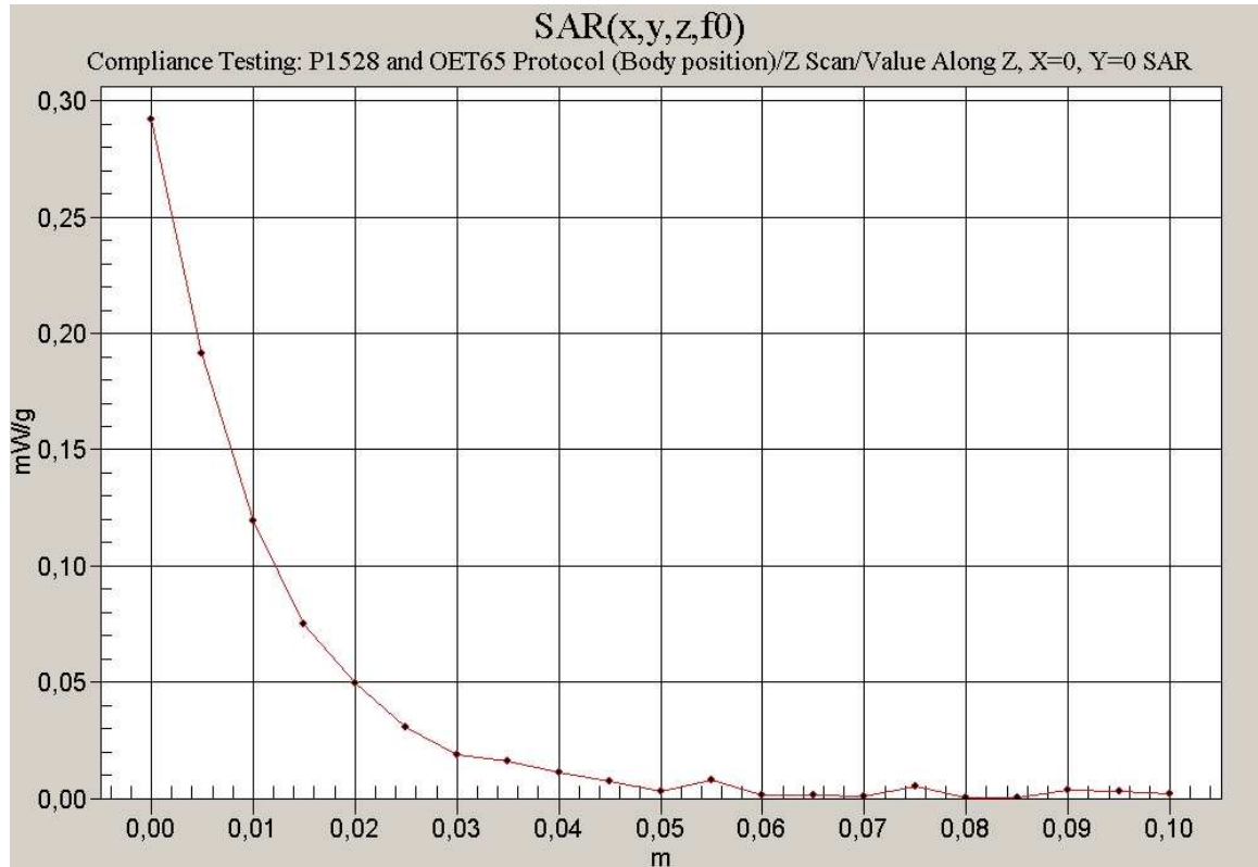
Z-scan Body 1900 MHz
