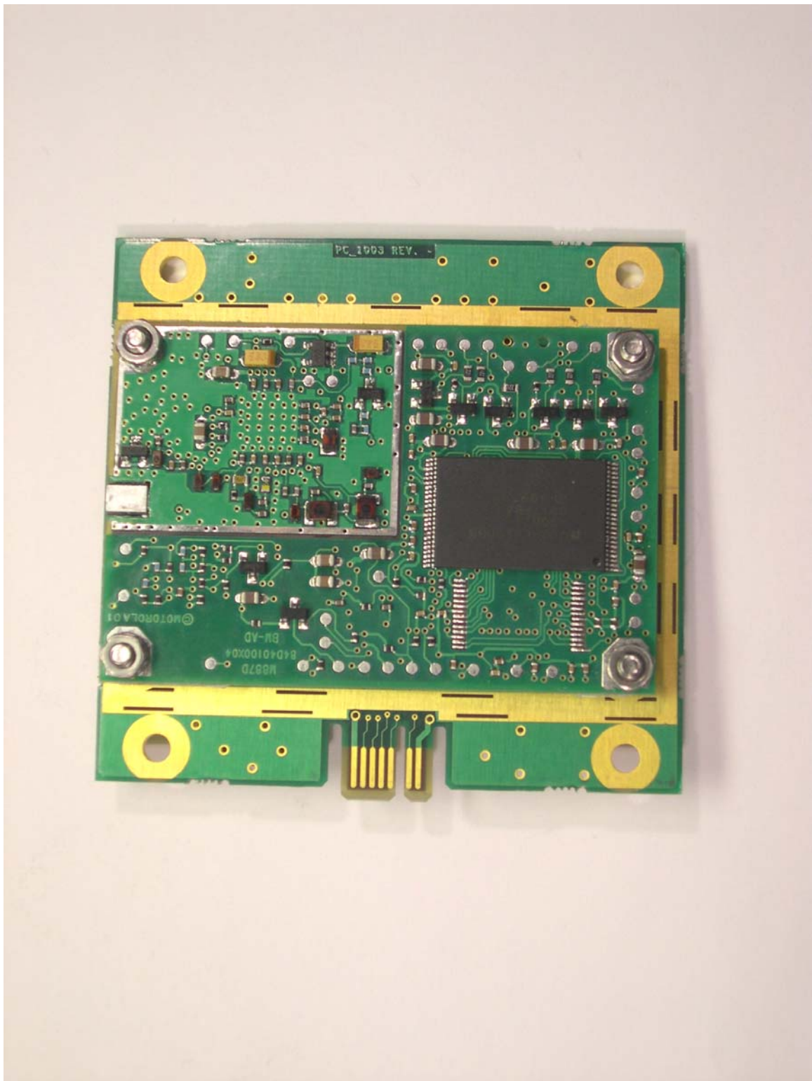
Flight Computer, Rear View with COTS GPS Receiver (Motorola M-12)
