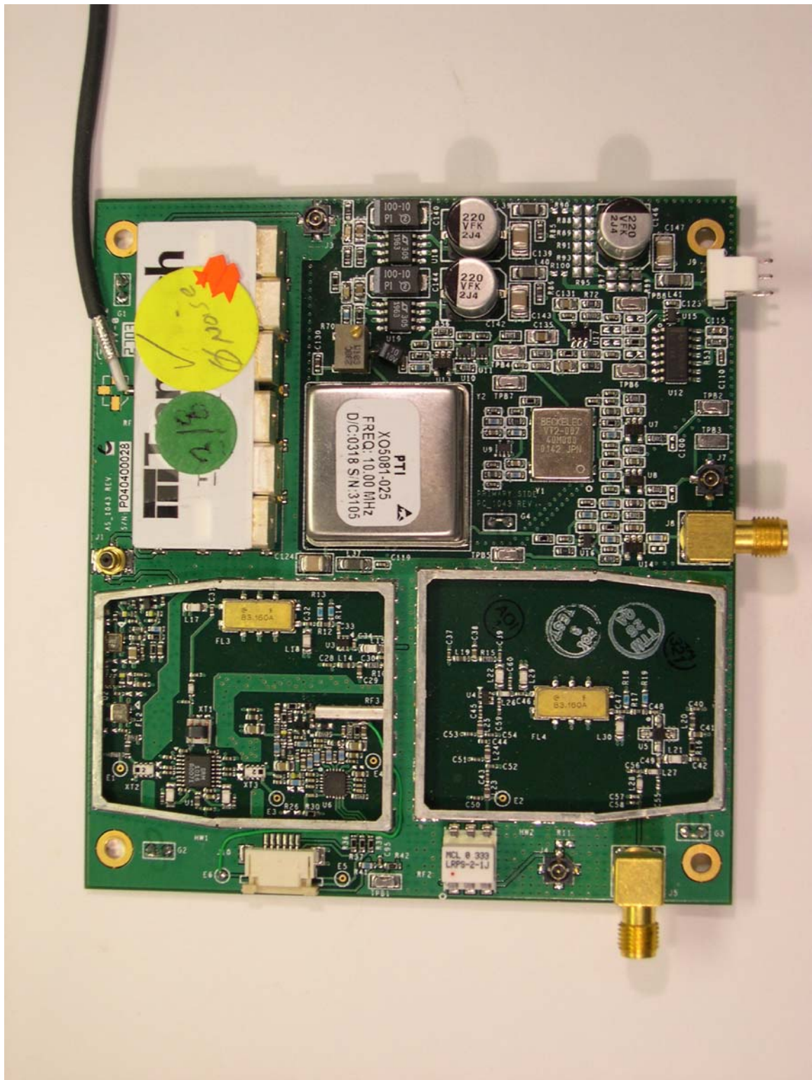
High Intercept Board, Front View
