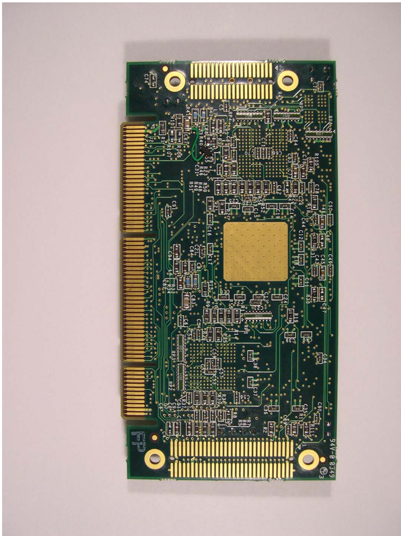
Baseband Processor – bottom view
