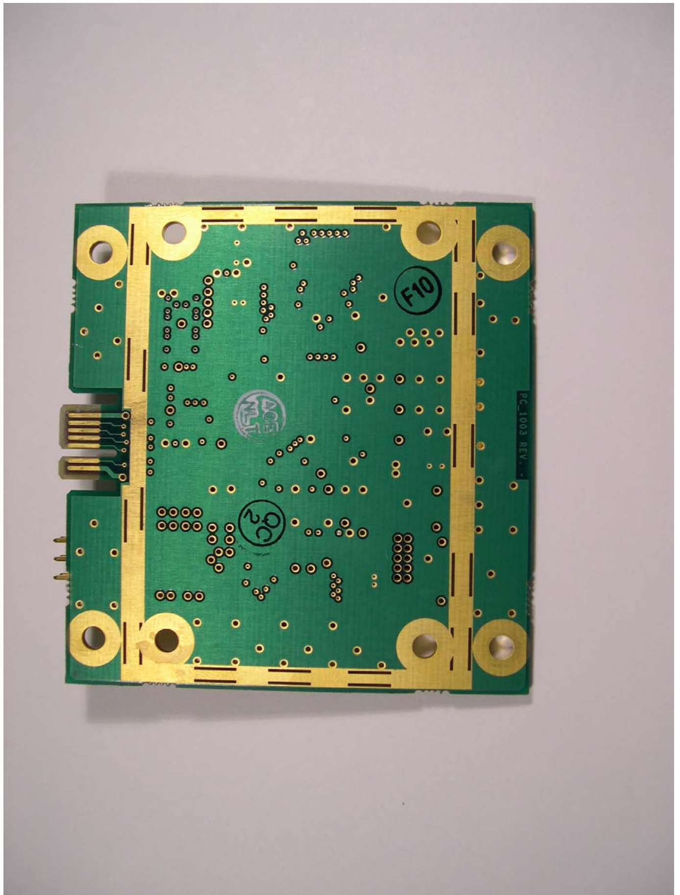
Flight computer - bottom
