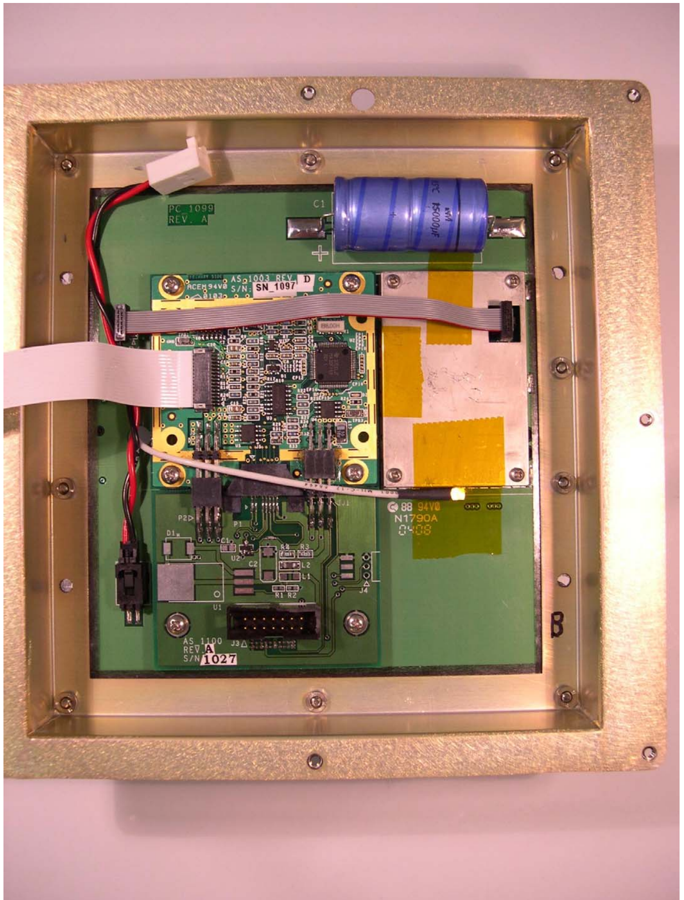
Battery Printed Circuit Board – bottom
