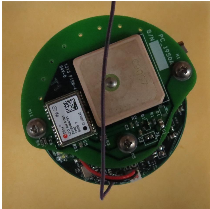
Top View without Radome
