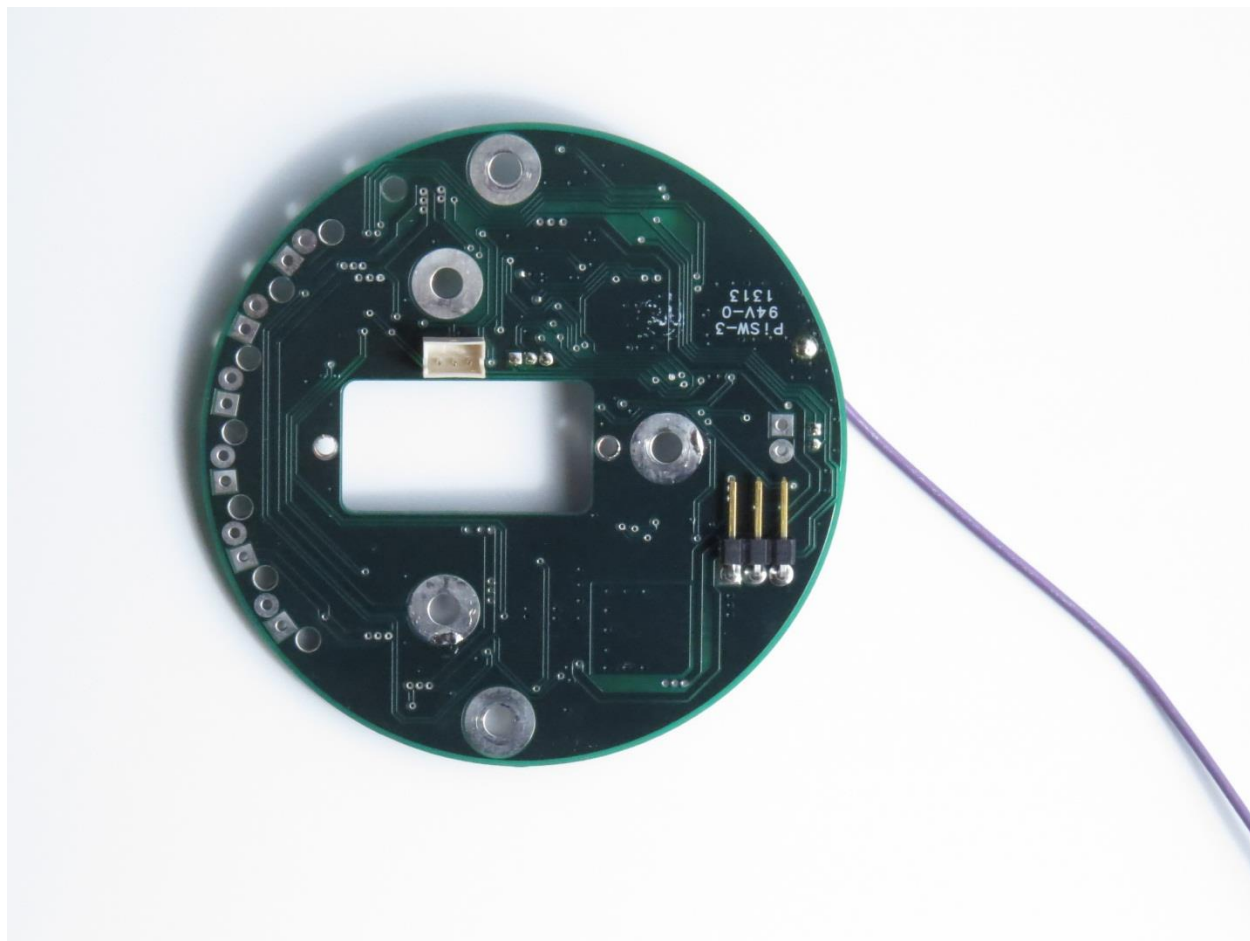
Line Cutter Board Bottom
