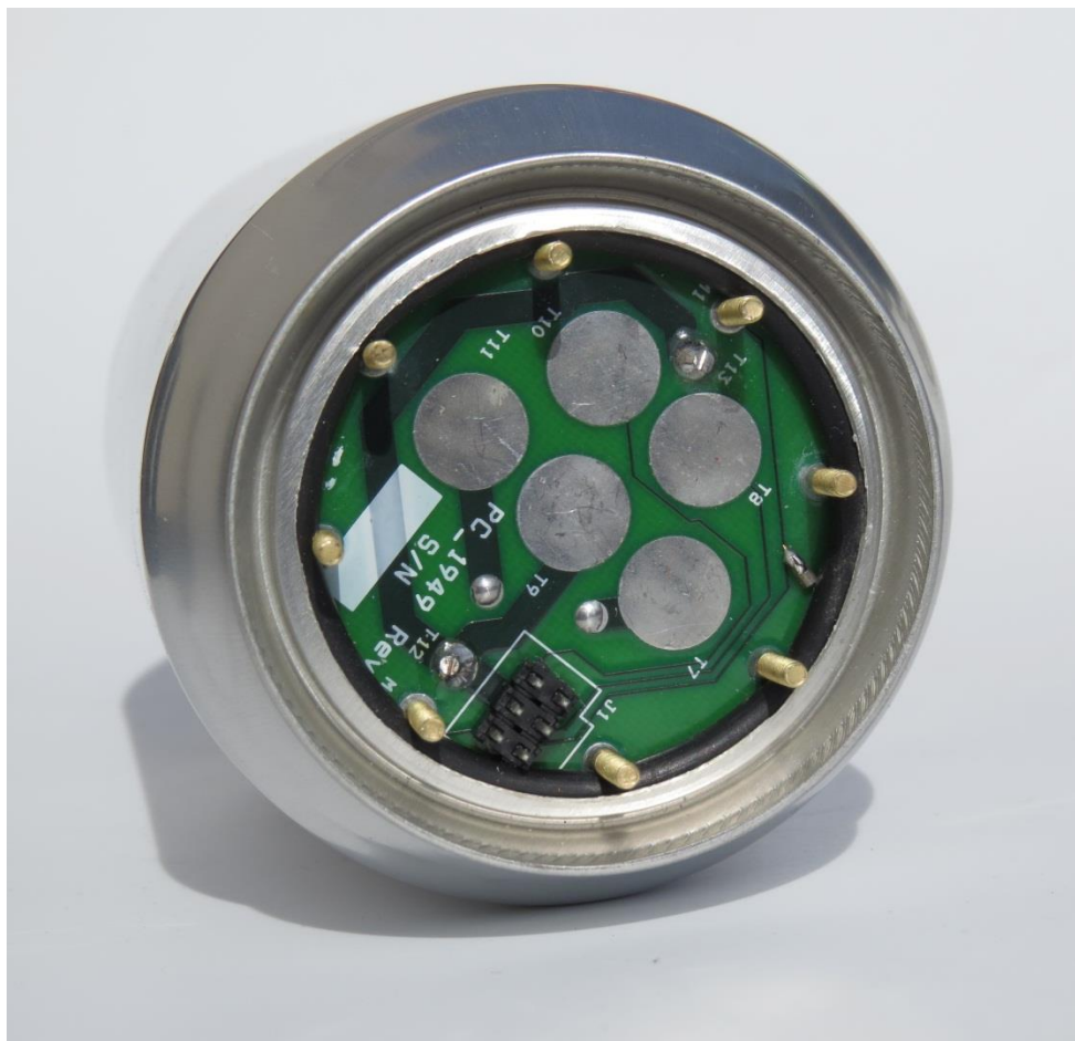
Radio Can after lid seaming TOP VIEW
