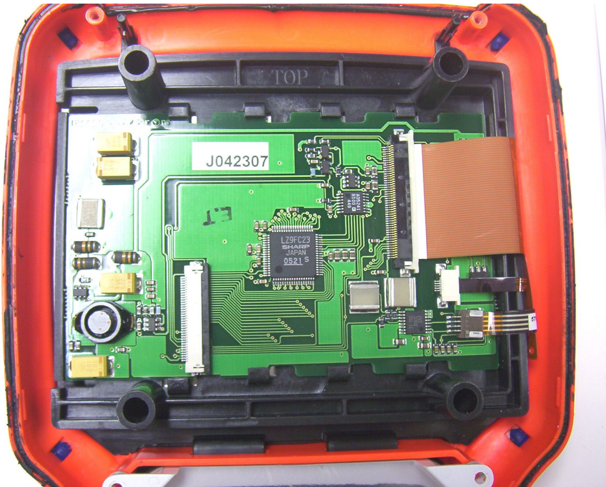
Photo 4: Sharp Display PCB View
