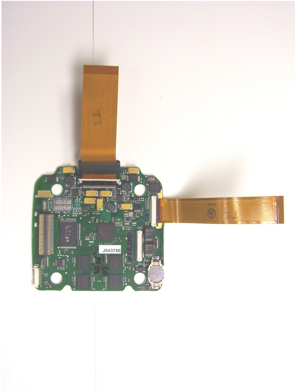
Photo 2: CPU PCB Top View
