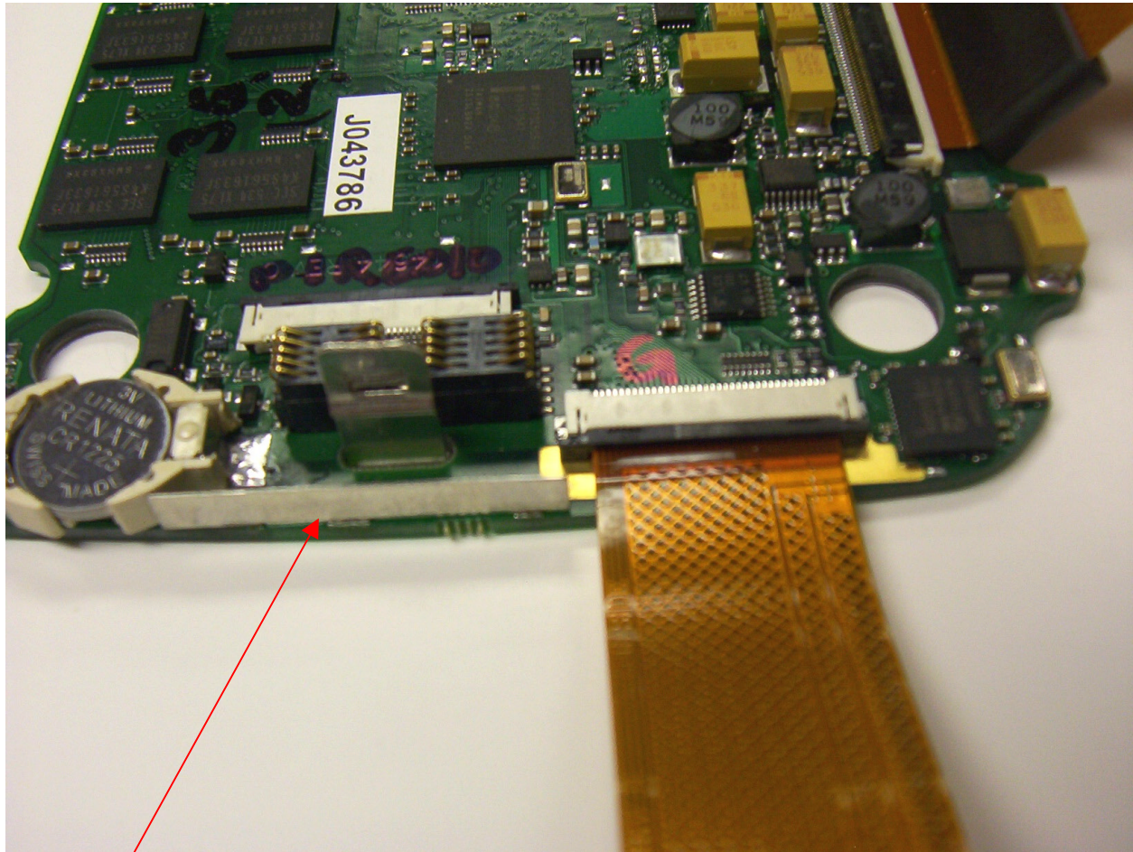
Transmitting Antenna
