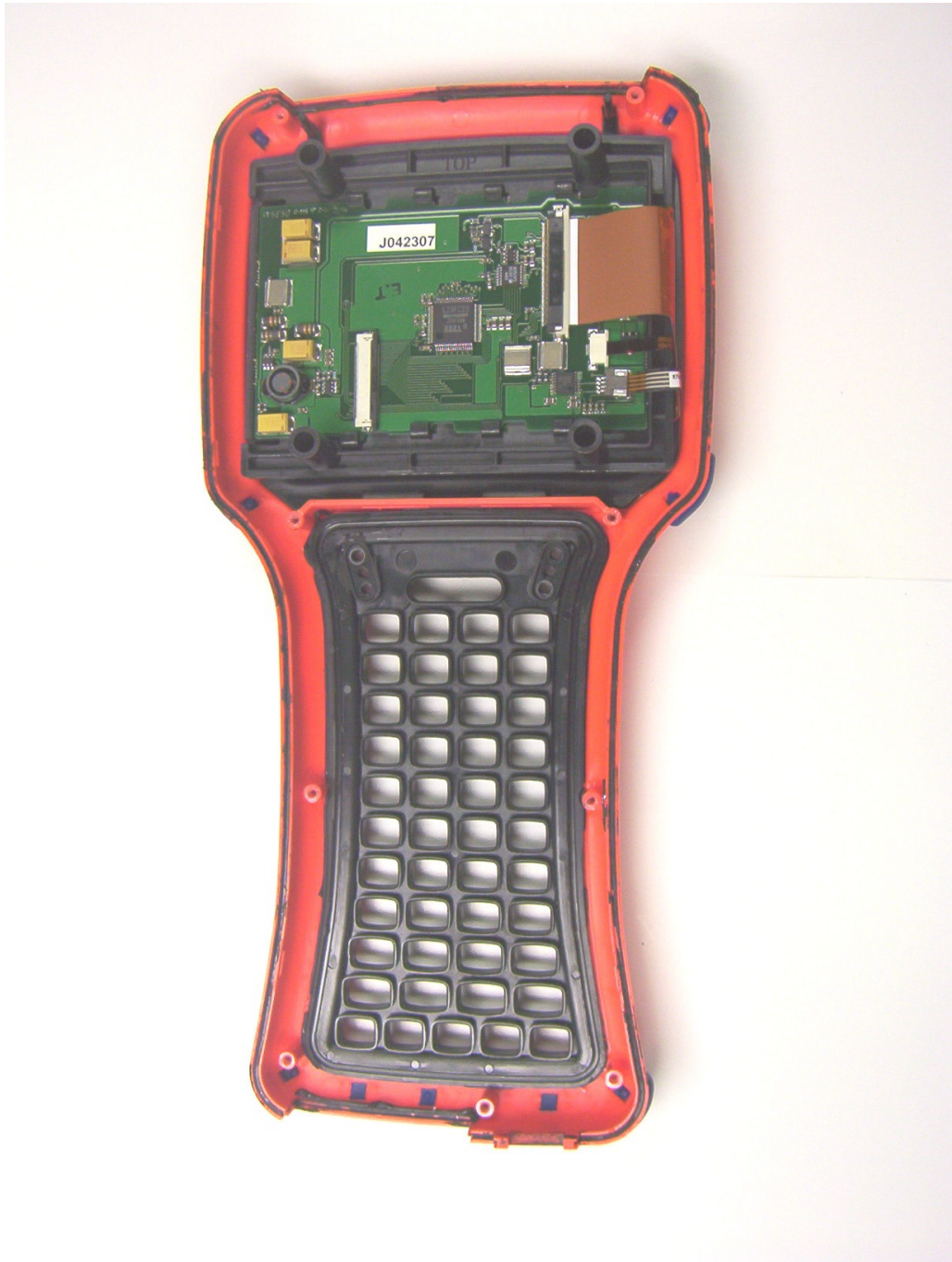
Photo 2: JETT.XL Top Half Close-up View
