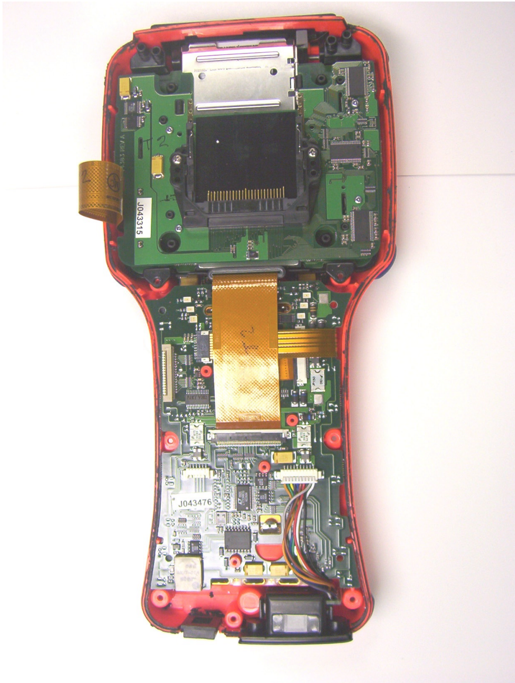
Photo 3: JETT.XL Bottom Half Close-up (Lower with KB Pad Removed) View
