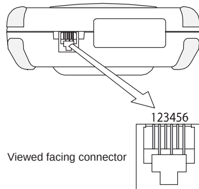
Figure 2-9: 6-Pin Modular Interface Connector
