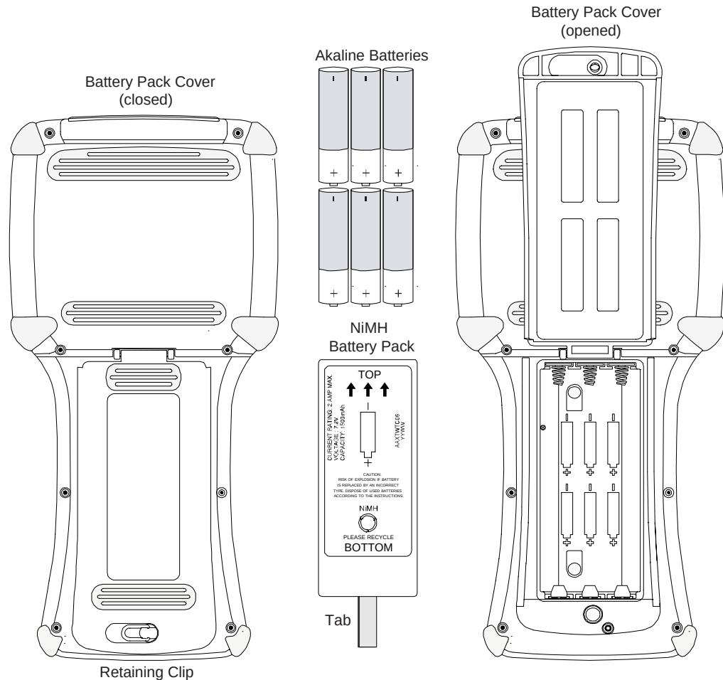
Figure 3-6: Changing Batteries
