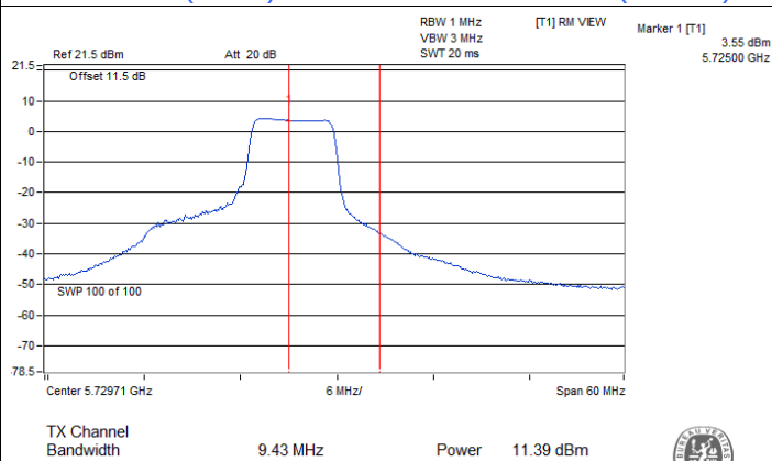
802.11ax (HE20) RU52 / Chain 1 : CH 144 (U-NII-3)
