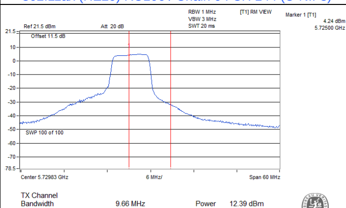
802.11ax (HE20) RU106 / Chain 0 : CH 144 (U-NII-3)
