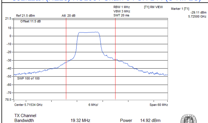
802.11ax (HE20) RU106 / Chain 0 : CH 144 (U-NII-2C)
