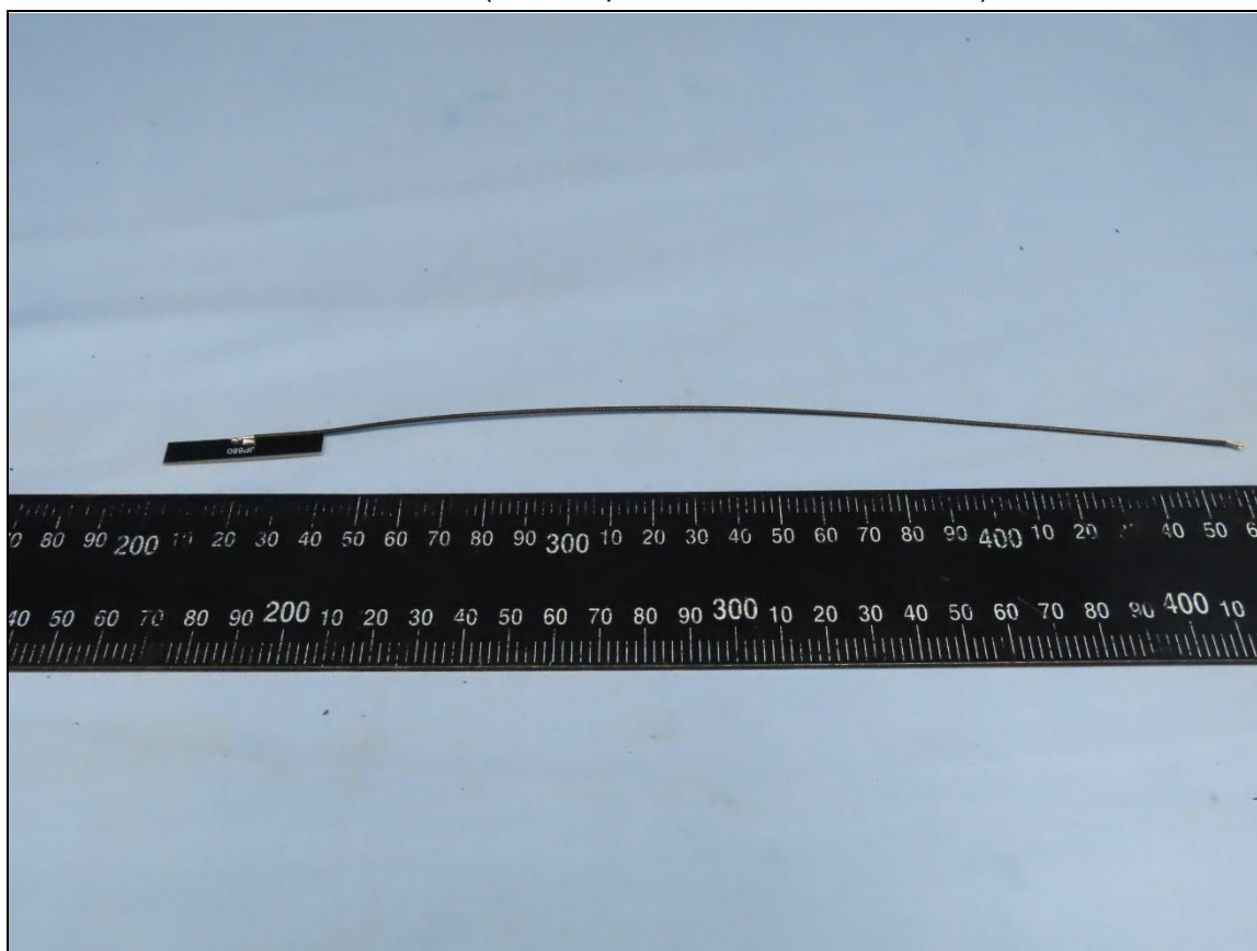
Antenna Set 7 (Brand: SparkLAN / Model: AD-516AX)
