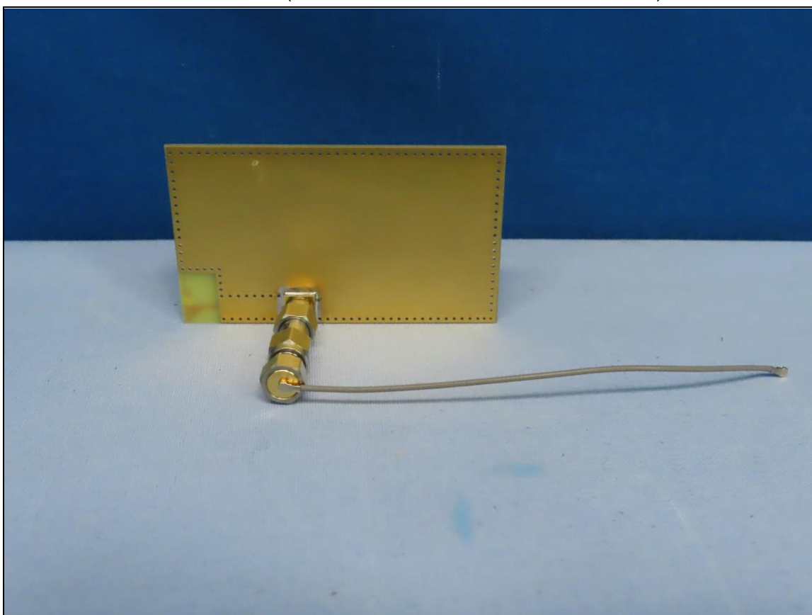
Antenna Set 8 (Brand: Johanson / Model: 2450AD18A6050)
