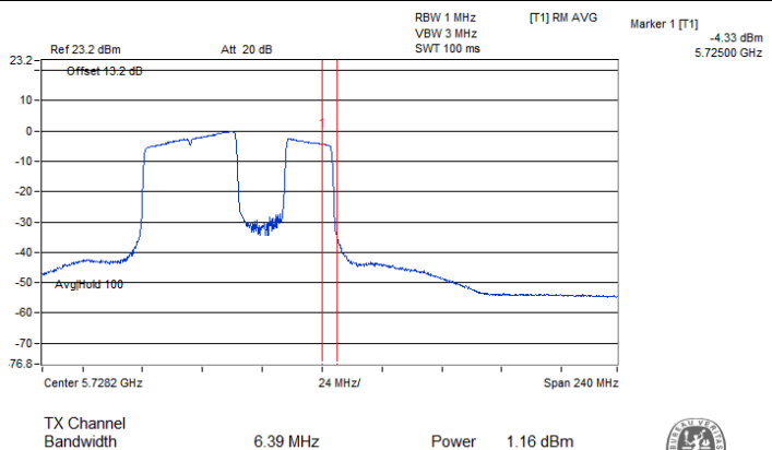
802.11be (EHT80) Punctured by 20 MHz / Chain 0 : CH 138 (U-NII-3)
