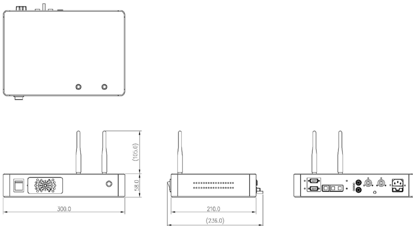
Figure 2.5 SCU Dimension
