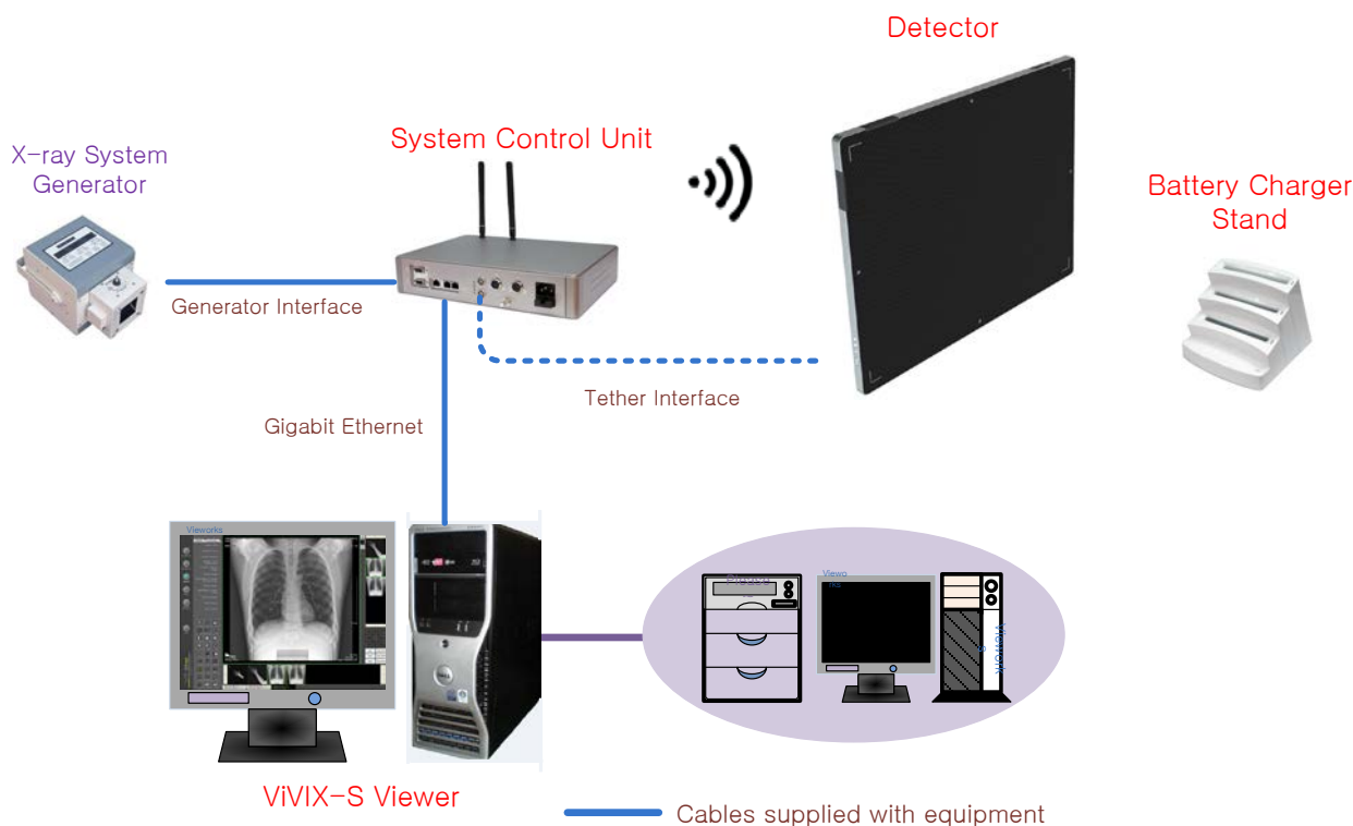
Figure 1.1 ViVIX-S Wireless System Configuration
