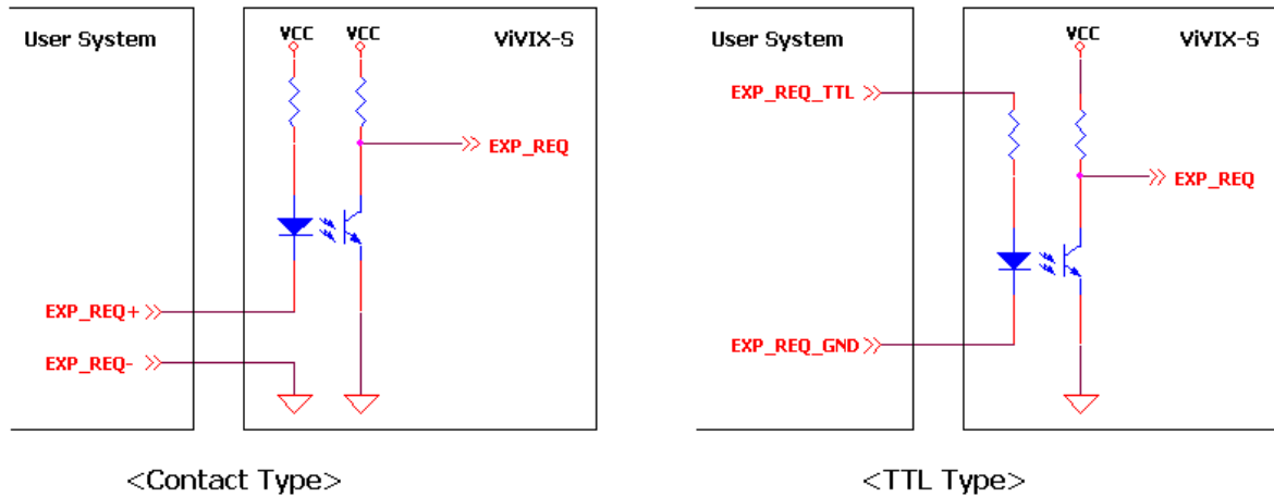
Figure 2.14 Exposure Request Input Circuit
