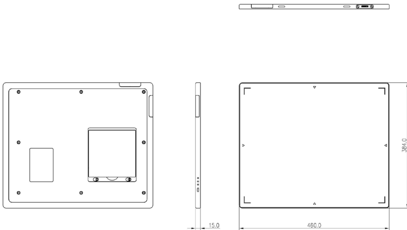
Figure 2.2 Detector Dimension
