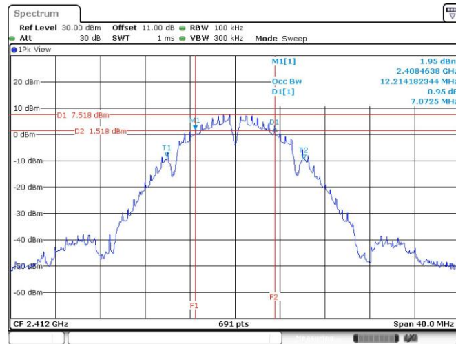
Worst Plot
