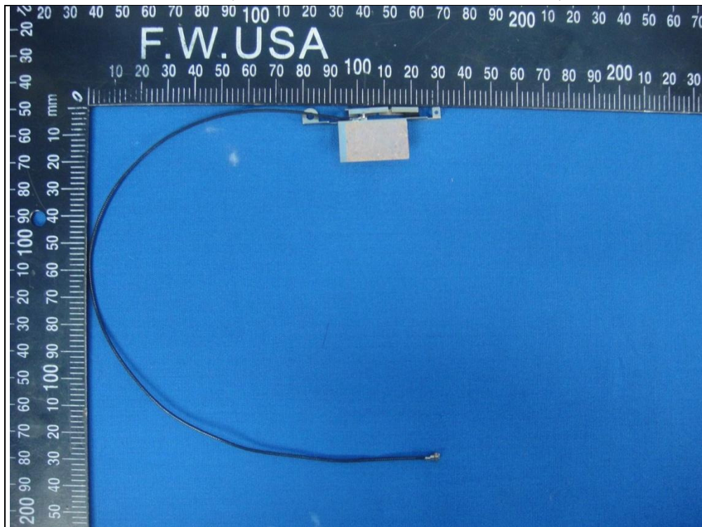
Antenna (Brand: WNC, Model: 81.EBJ15.005)
