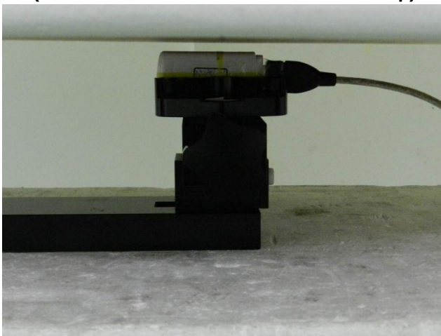
USB Cable Plug-in USB Configuration 4 (Vertical Back with Phantom 5 mm Gap)
