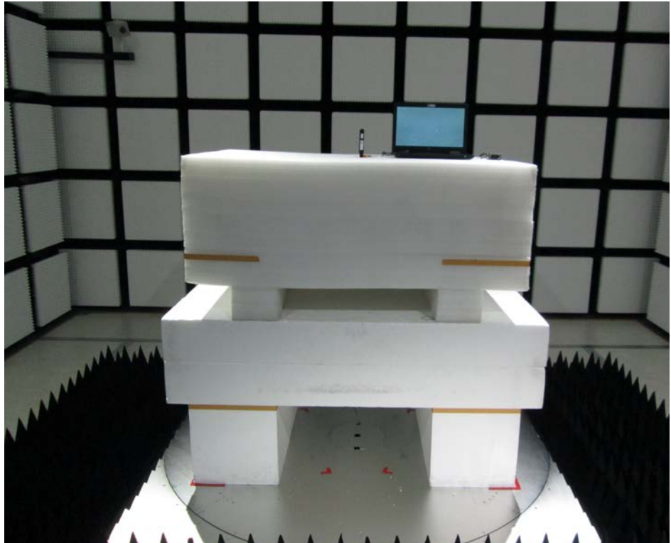
FRONT VIEW
