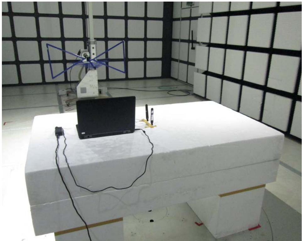
REAR VIEW
