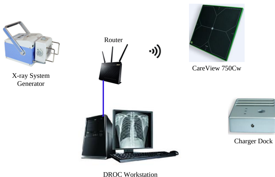
Figure 2 Wireless configuration
