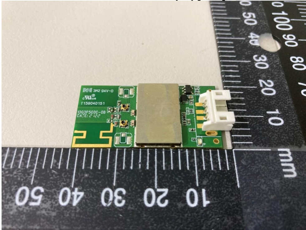
Outview: WUBT-239ACN(BT) [P4W] Pic 1
