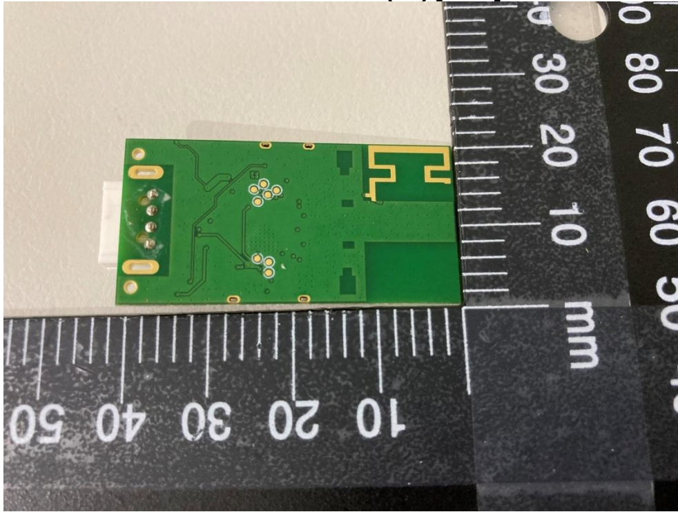
Outview: WUBT-239ACN(BT) [M4W] Pic 4
