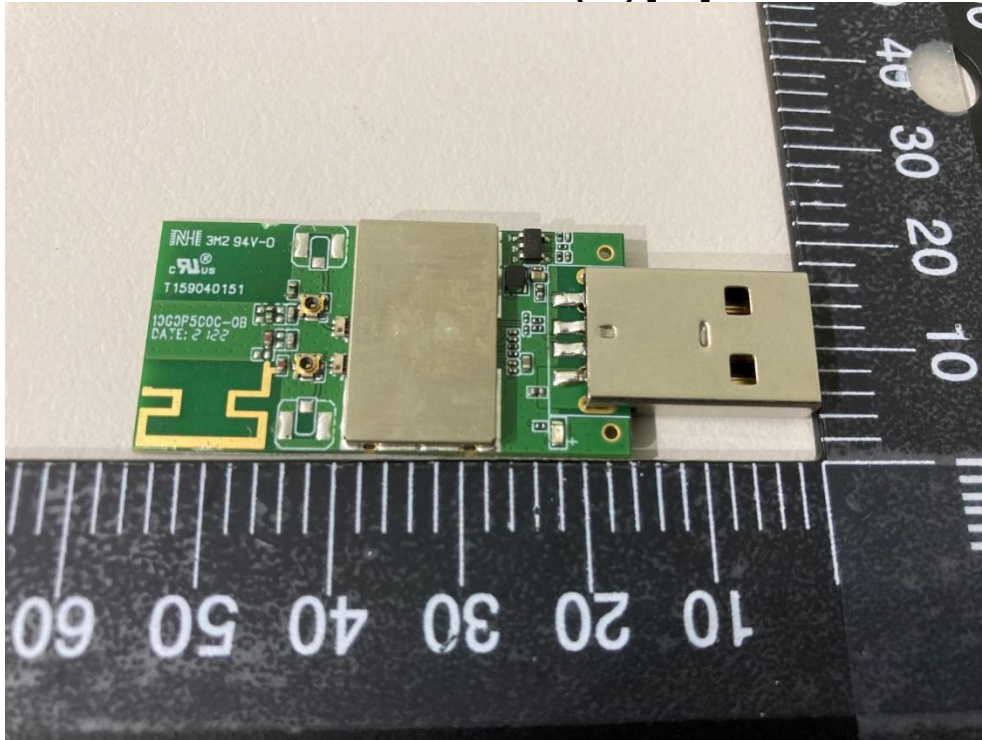
Outview: WUBT-239ACN(BT) [PU] Pic 1
