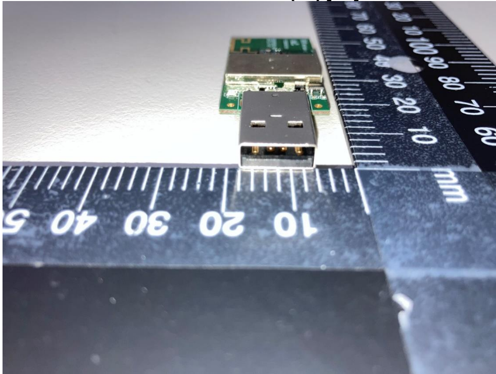
Outview: WUBT-239ACN(BT) [PU] Pic 3
