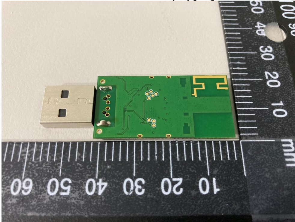
Outview: WUBT-239ACN(BT) [MU] Pic 3
