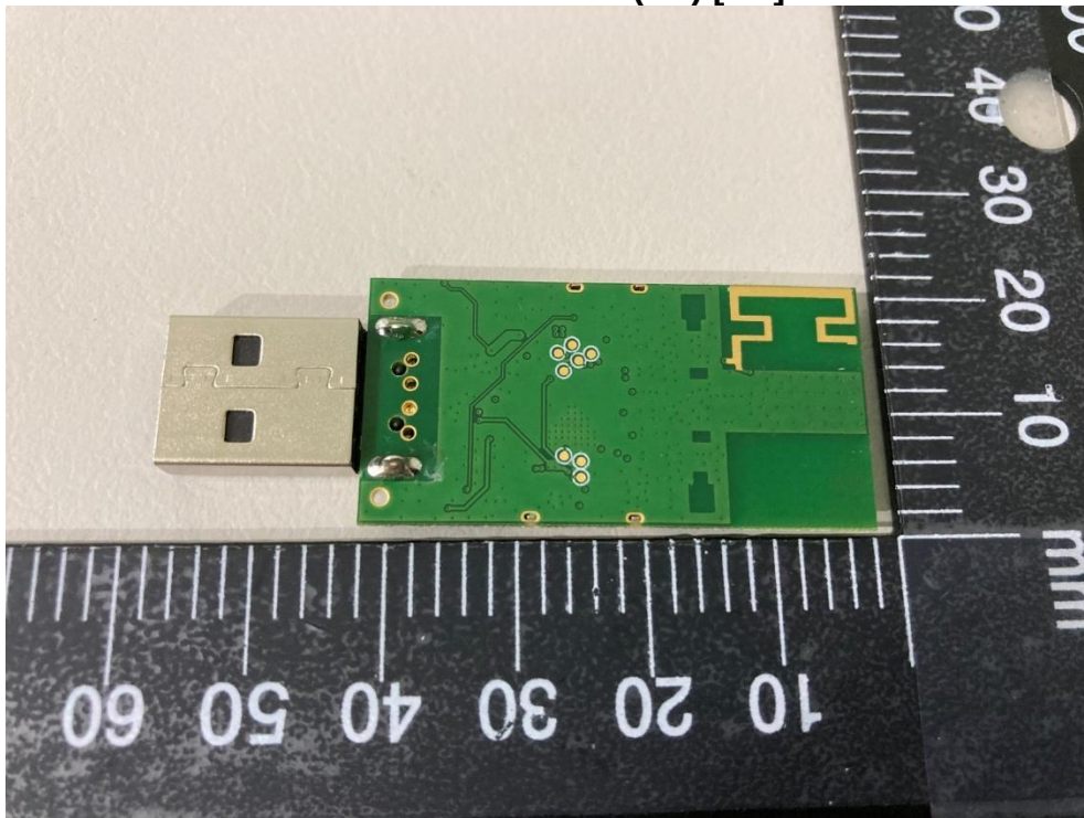
Outview: WUBT-239ACN(BT) [PU] Pic 2
