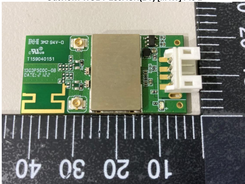
Outview: WUBT-239ACN(BT) [M4W] Pic 2
