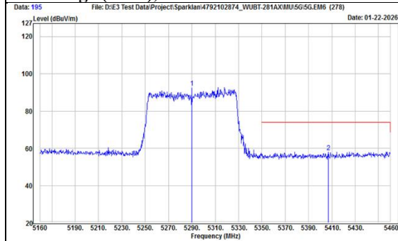
TX, 802.11ac(VHT80) (Ch 58) Band Edge (Peak), Horizontal
