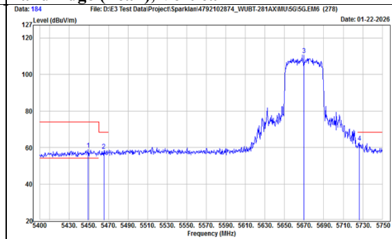
TX, 802.11ax(HE40) (Ch 134) Band Edge (Peak), Vertical
