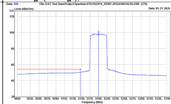
TX, 802.11ax(HE40) (Ch 38) Band Edge (Peak), Vertical
