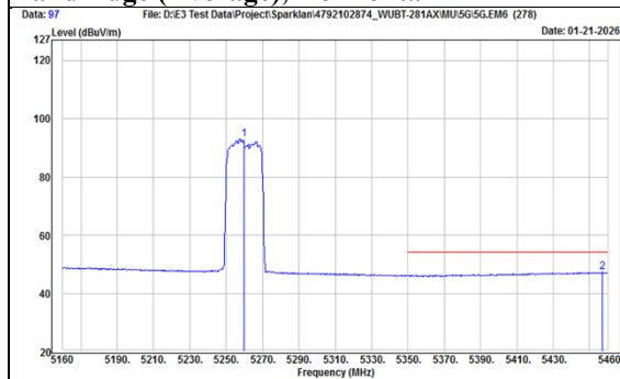
TX, 802.11ax(HE20) (Ch 52) Band Edge (Peak), Horizontal
