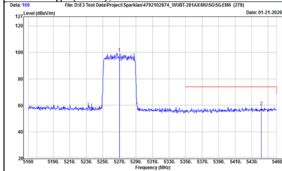
TX, 802.11ax(HE40) (Ch 54) Band Edge (Peak), Horizontal
