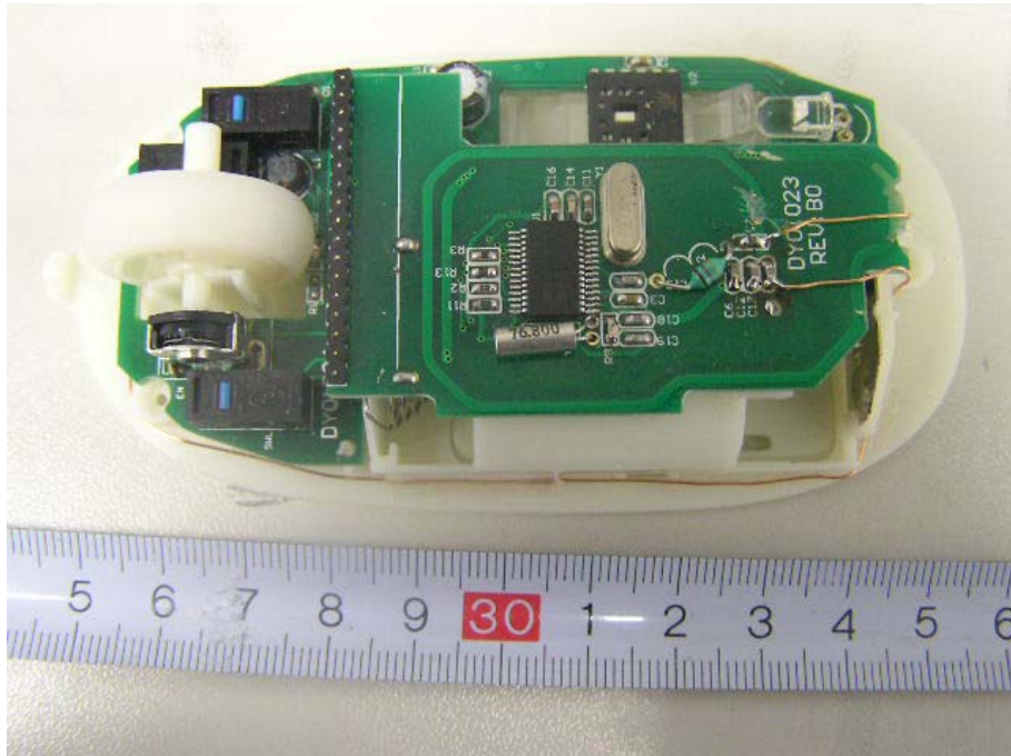
EUT-Uncover View
