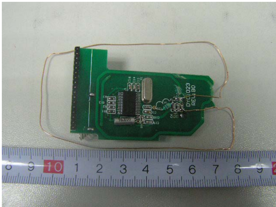
EUT- Top View of Antenna Board
