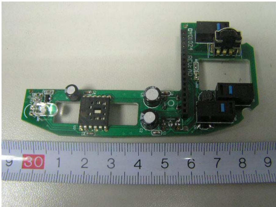
EUT-Top View of Main Board
