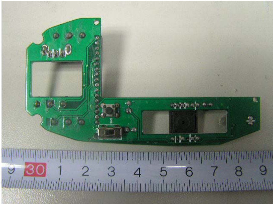
EUT- Bottom View of Main Board
