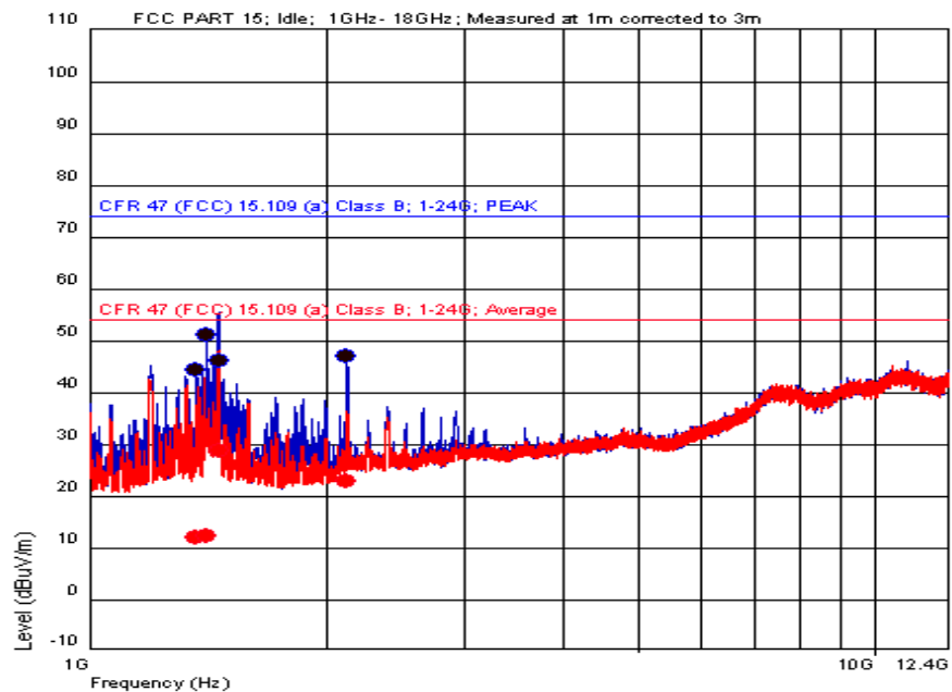
Picture 10: radiated emission results, 1 – 12.400 GHz, Red= horizontal polarization, blue = vertical polarization
