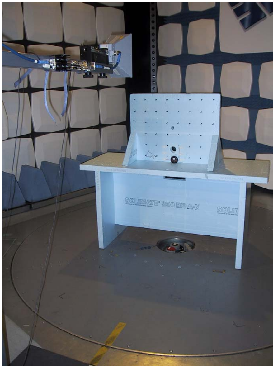
Picture 1: Spurious emission and field strength measurement setup
