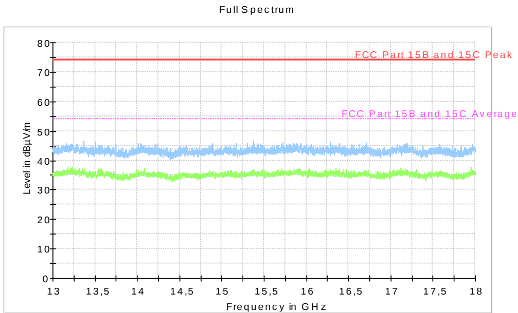
Diagram, Peak overview sweep, 13 – 18 GHz at 3 m distance. RX mid channel, EUT orientation Y.
