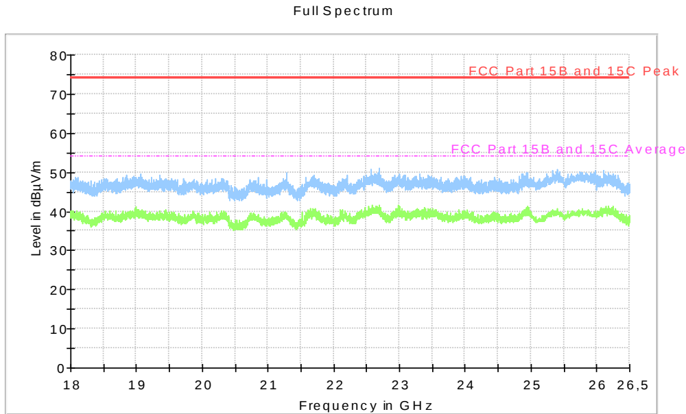
Diagram, Peak overview sweep, 18 – 26 GHz at 3 m distance. RX mid channel, EUT orientation X.
