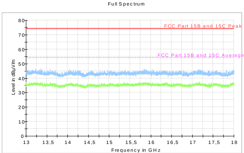
Diagram, Peak overview sweep, 13-18 GHz at 3 m distance, RX low channel, EUT orientation Y
