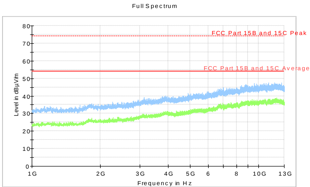
Diagram, Peak overview sweep, 1 – 13 GHz at 3 m distance. RX low channel, EUT orientation Y.
