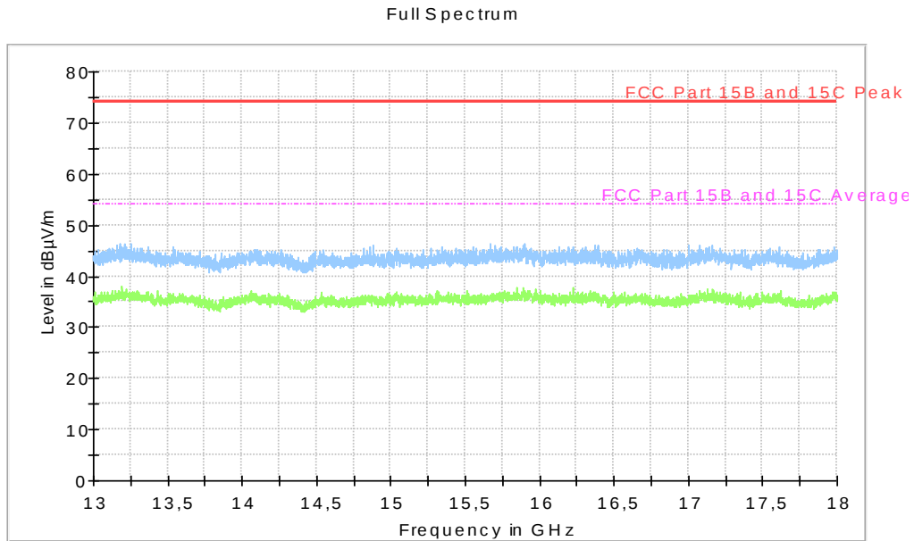
Diagram, Peak overview sweep, 13 – 18 GHz at 3 m distance. TX mid channel, EUT orientation Y.
