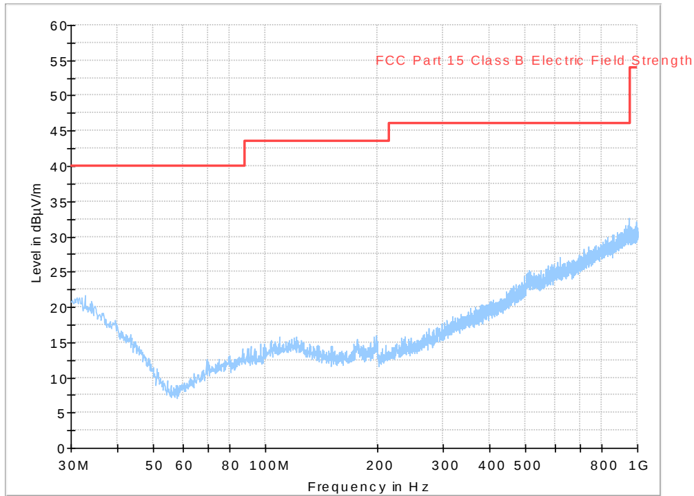
Diagram, Peak overview sweep, 30 – 1000 MHz at 3 m distance. RX mid channel, EUT orientation X.
