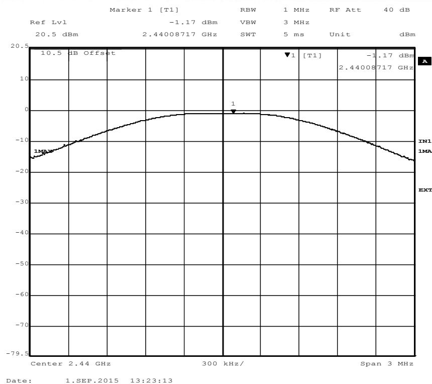
Diagram, maximum peak conducted output power, TX mid channel
