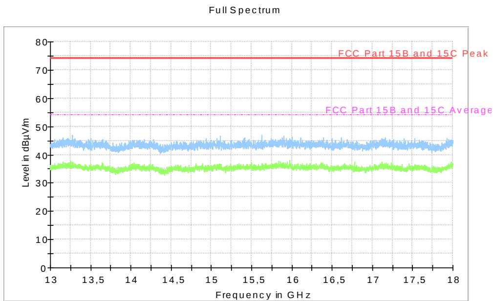
Diagram, Peak overview sweep, 13 – 18 GHz at 3 m distance. TX mid channel, EUT orientation Z.
