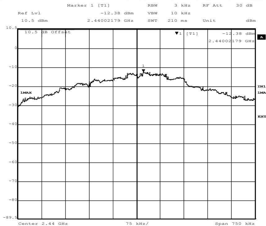
Diagram, peak power spectral density, TX mid channel
