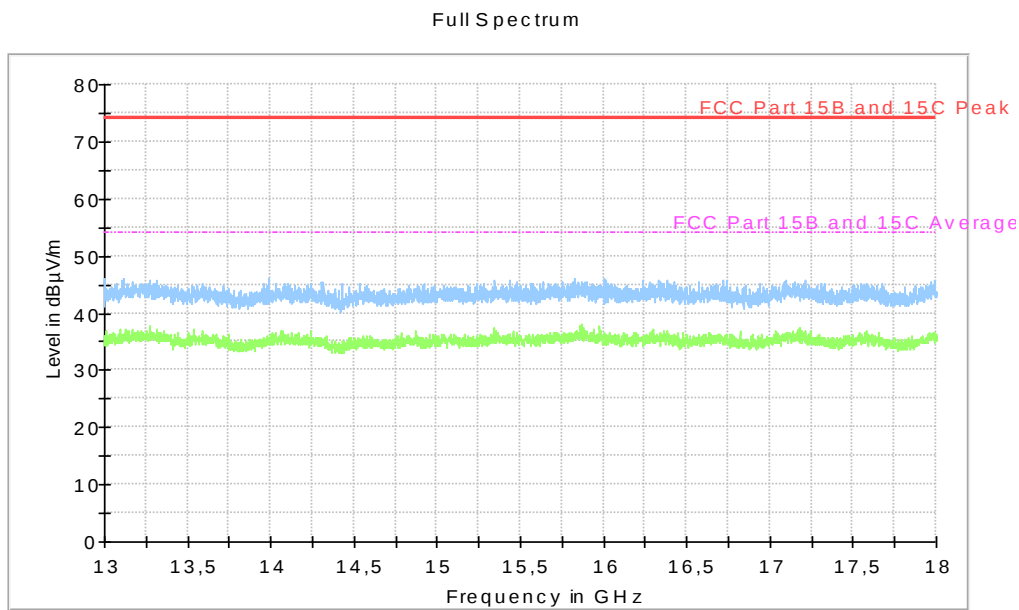
Diagram, Peak overview sweep, 13 – 18 GHz at 3 m distance. RX mid channel, EUT orientation X.
