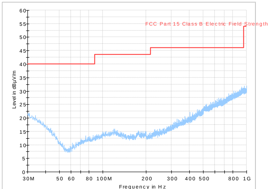
Diagram, Peak overview sweep, 30 – 1000 MHz at 3 m distance. RX low channel, EUT orientation Y.
