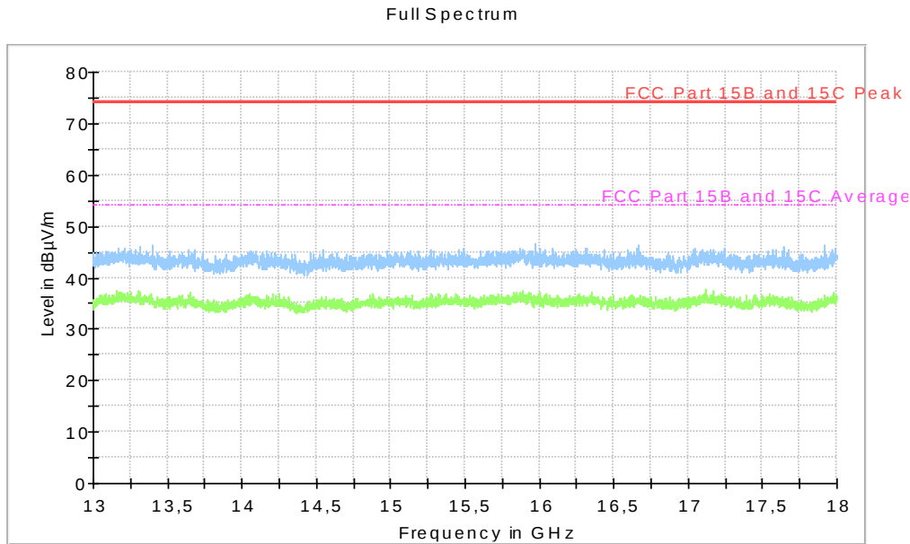
Diagram, Peak overview sweep, 13 – 18 GHz at 3 m distance. RX mid channel, EUT orientation Z.
