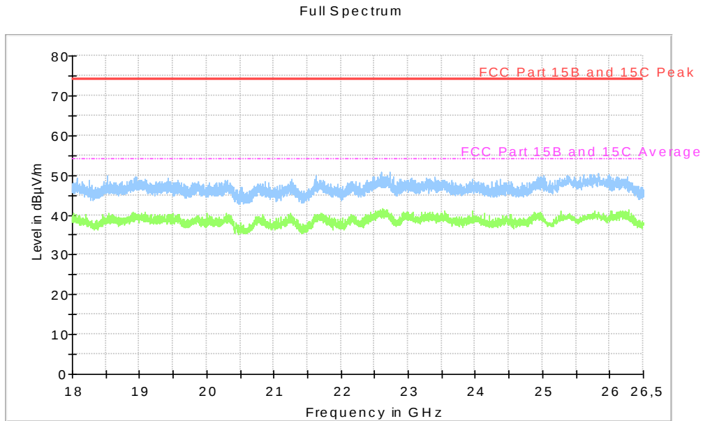
Diagram, Peak overview sweep, 18 – 26 GHz at 3 m distance. TX high channel, EUT orientation Y.
