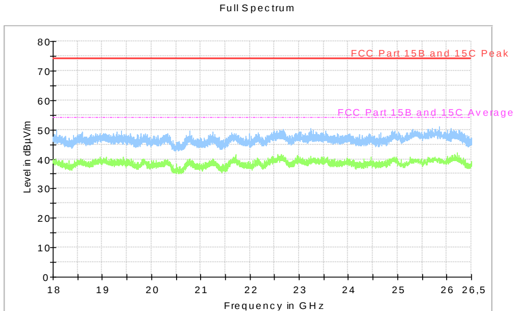
Diagram, Peak overview sweep, 18 – 26 GHz at 3 m distance. RX mid channel, EUT orientation Y.
