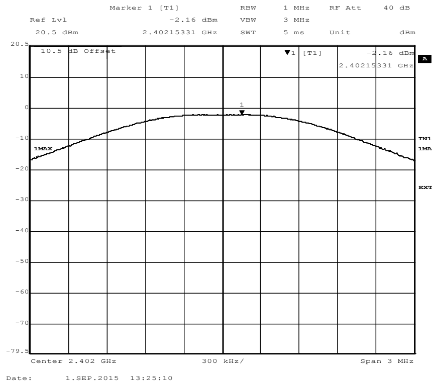
Diagram, maximum peak conducted output power, TX low channel
