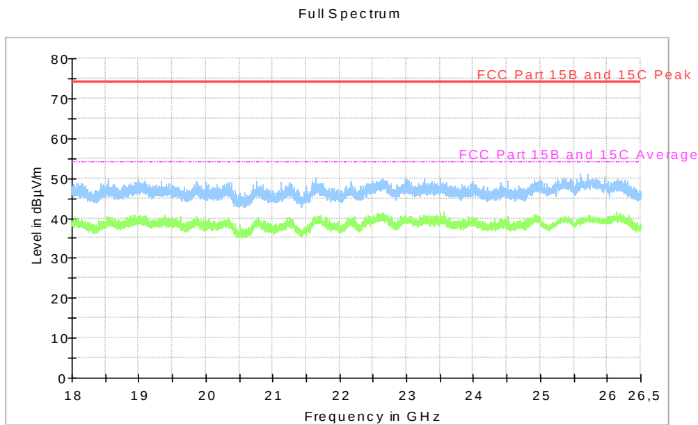
Diagram, Peak overview sweep, 18 – 26 GHz at 3 m distance. RX high channel, EUT orientation Y.
