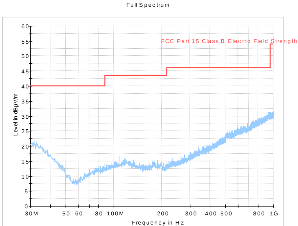
Diagram, Peak overview sweep, 30 – 1000 MHz at 3 m distance. TX low channel, EUT orientation Y.
