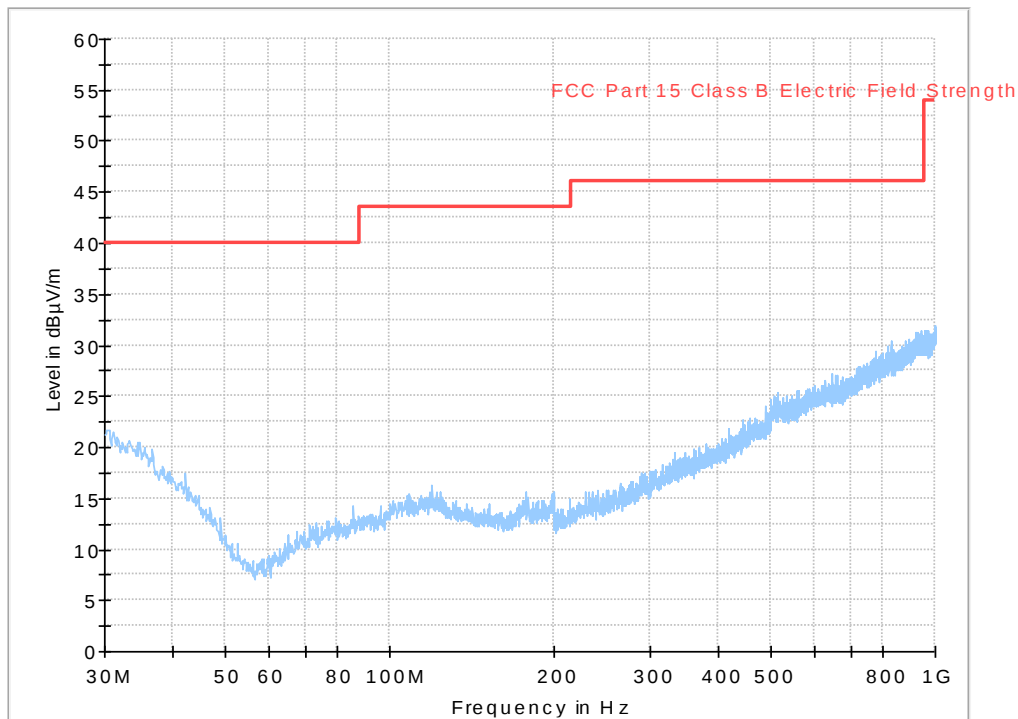
Diagram, Peak overview sweep, 30 – 1000 MHz at 3 m distance. RX high channel, EUT orientation Y.
