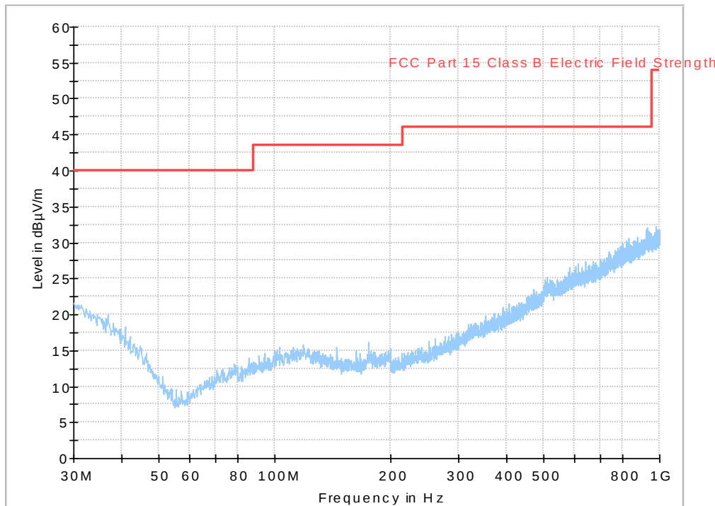
Diagram, Peak overview sweep, 30 – 1000 MHz at 3 m distance. RX mid channel, EUT orientation Y.
