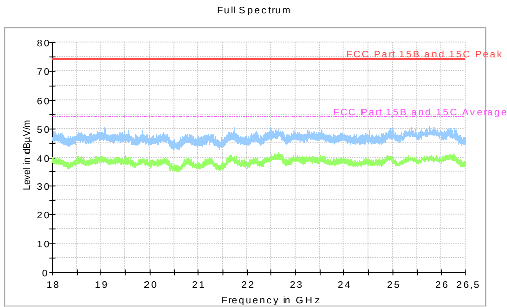
Diagram, Peak overview sweep, 18 – 26 GHz at 3 m distance. RX mid channel, EUT orientation Z.
