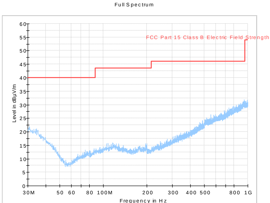
Diagram, Peak overview sweep, 30 – 1000 MHz at 3 m distance. TX mid channel, EUT orientation Y.
