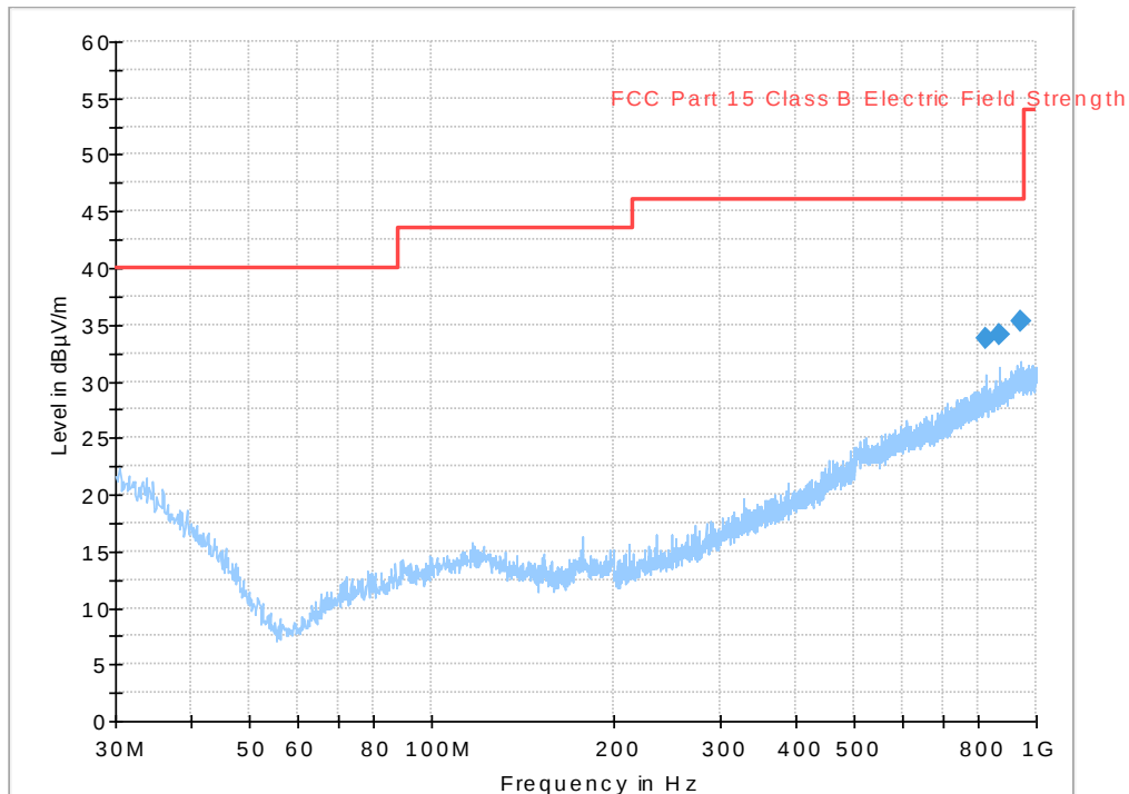
Diagram, Peak overview sweep, 30 – 1000 MHz at 3 m distance. RX mid channel, EUT orientation Z.
