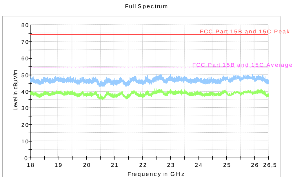
Diagram, Peak overview sweep, 18 – 26 GHz at 3 m distance. TX mid channel, EUT orientation X.
