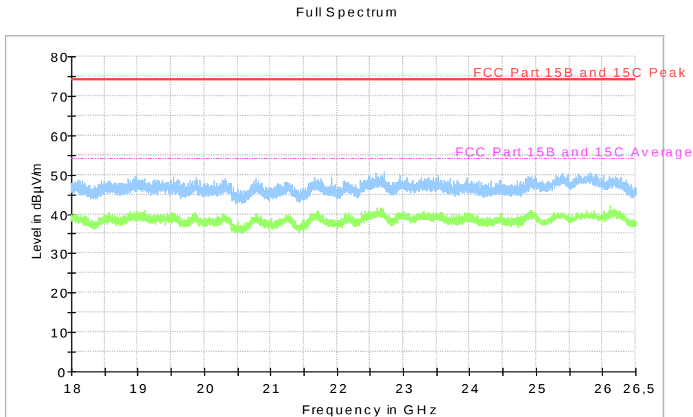
Diagram, Peak overview sweep, 18 – 26 GHz at 3 m distance. TX mid channel, EUT orientation Z.
