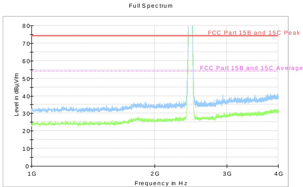
Diagram, Peak overview sweep, 1 – 4 GHz at 3 m distance. TX mid channel, EUT orientation Y.
