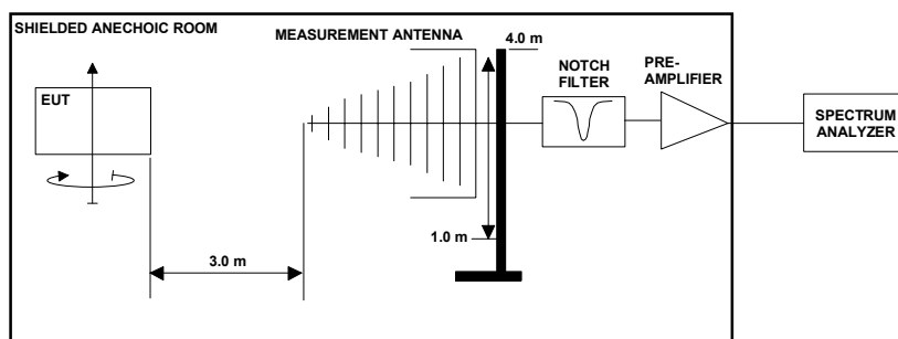
Picture 1: Test setup for radiated spurious emissions measurement 30 MHz - 3 GHz frequencies
