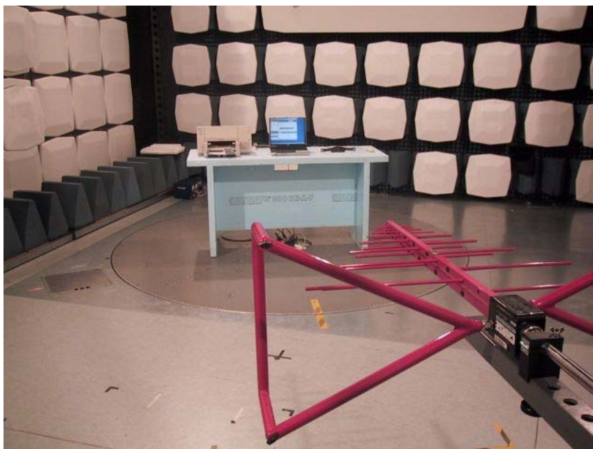
Picture 2: Radiated emission measurement setup
