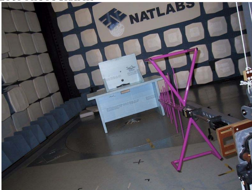
Picture 1: Spurious emission and field strength measurement setup
