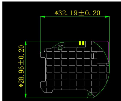
NFC Antenna Diagram
