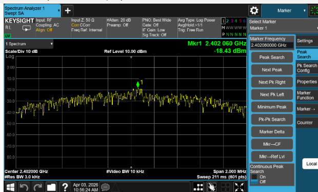
GFSK (BLE 2Mbps) LOW CHANNEL
