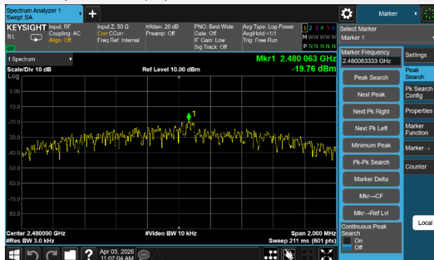
GFSK (BLE 2Mbps) HIGH CHANNEL
