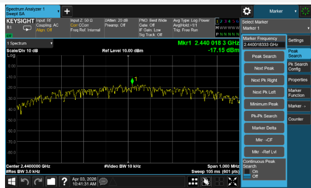
GFSK (BLE 1Mbps) MIDDLE CHANNEL
