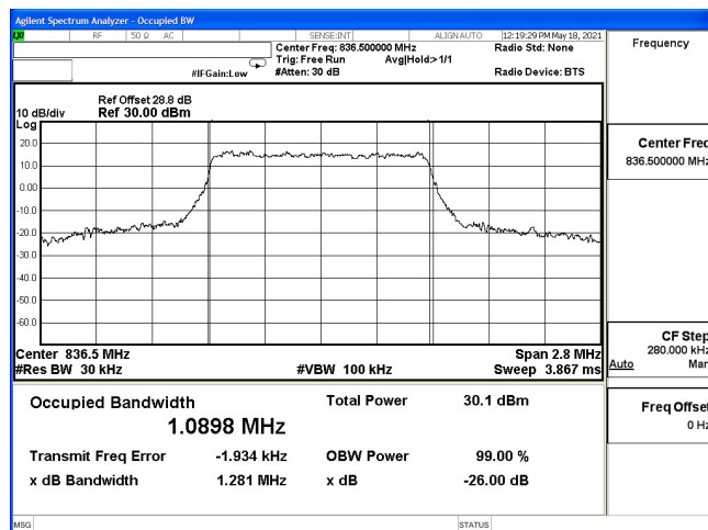
OCC-B5_1.4M-CH20525-16QAM
