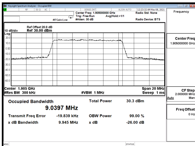
OCC-B2_10M-CH19150-16QAM
