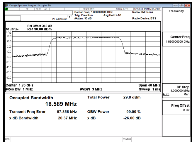
OCC-B2_20M-CH18700-QPSK
