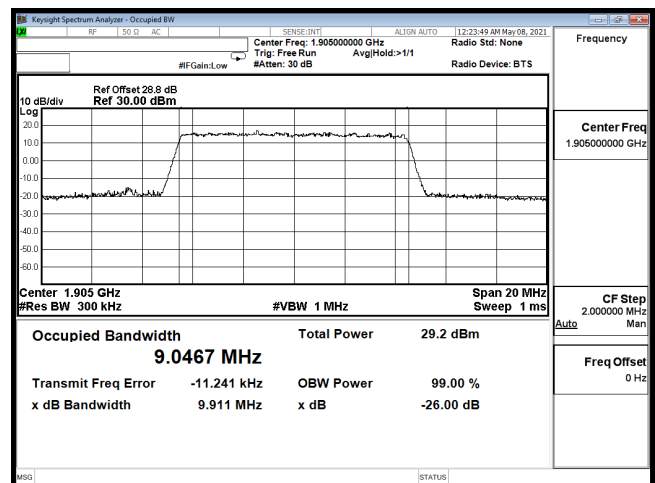
OCC-B2_10M-CH19150-64QAM
