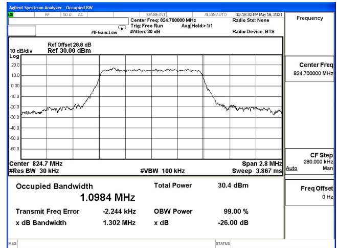
OCC-B5_1.4M-CH20407-16QAM
