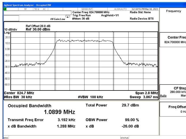
OCC-B5_1.4M-CH20407-64QAM
