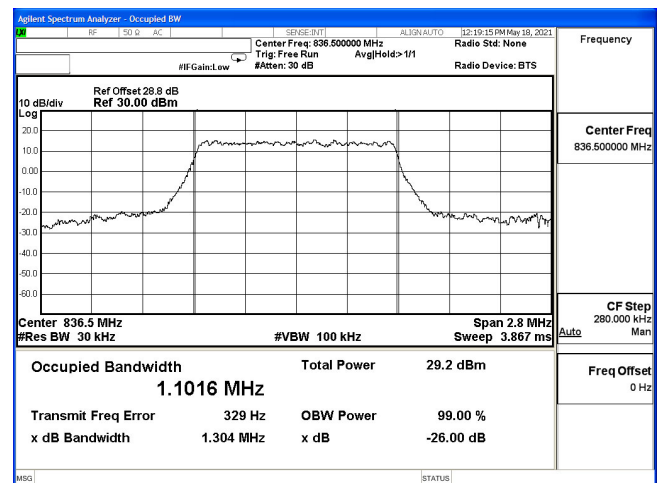
OCC-B5_1.4M-CH20525-64QAM
