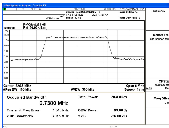
OCC-B5_3M-CH20415-64QAM
