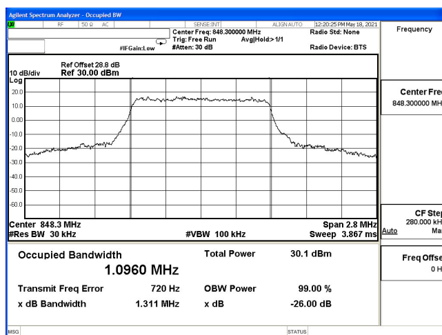
OCC-B5 1.4M-CH20643-16QAM
