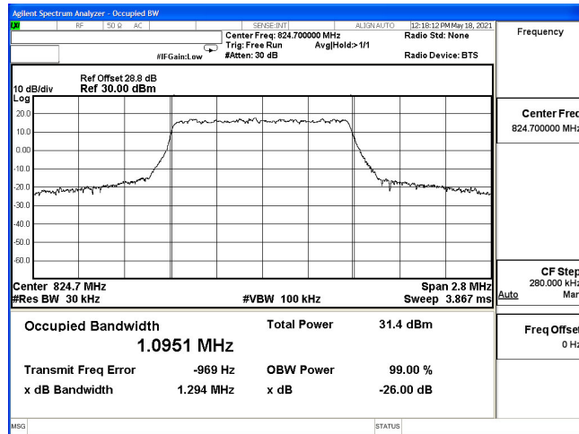
OCC-B5_1.4M-CH20407-QPSK
