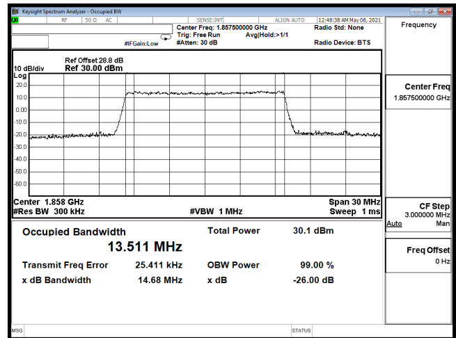
OCC-B2_15M-CH18675-16QAM
