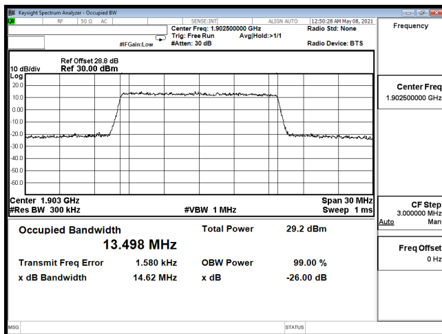
OCC-B2_15M-CH19125-64QAM
