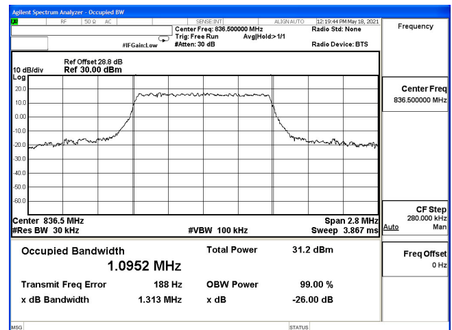
OCC-B5_1.4M-CH20525-QPSK
