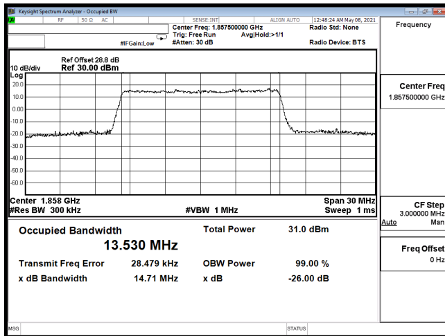
OCC-B2_15M-CH18675-QPSK
