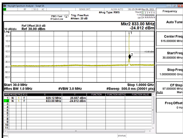
CSE-B5_10M-CH20450-16QAM(1,25)-30M-1G
