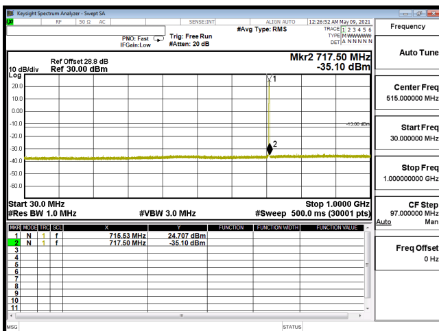
CSE-B12_1.4M-CH23173-64QAM(3,2)-30M-1G
