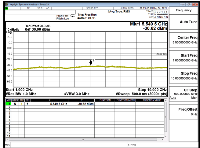
CSE-B12_1.4M-CH23173-QPSK(1,5)-1G-10G
