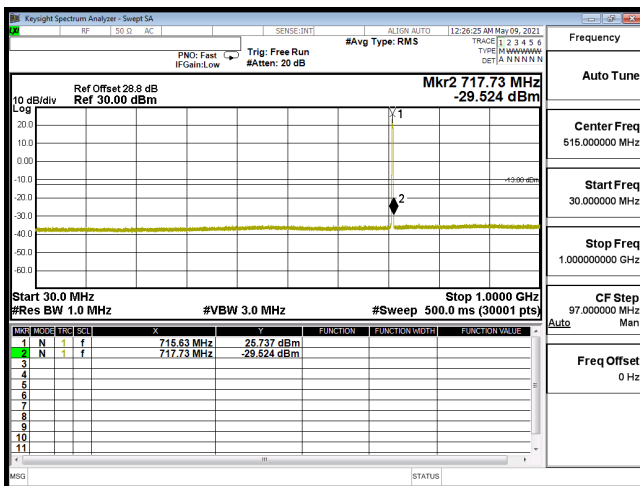
CSE-B12_1.4M-CH23173-16QAM(1,5)-30M-1G
