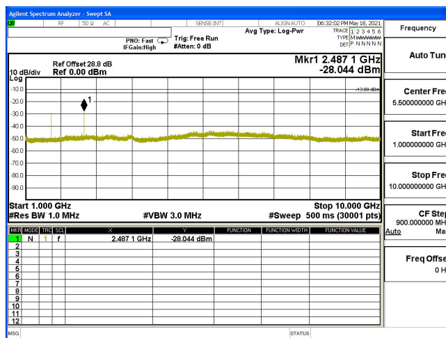
CSE-B5_10M-CH20450-16QAM(1,25)-1G-10G
