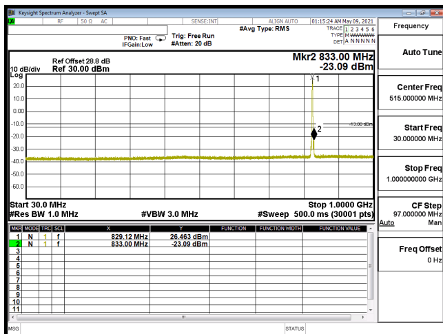
CSE-B5_10M-CH20450-QPSK(1,25)-30M-1G
