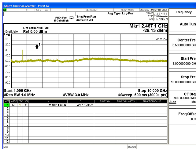
CSE-B5_10M-CH20450-QPSK(1,25)-1G-10G
