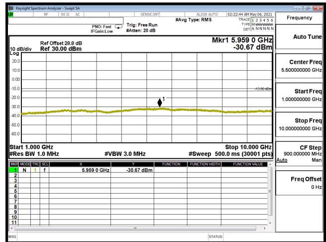
CSE-B12_1.4M-CH23095-QPSK(3,0)-1G-10G
