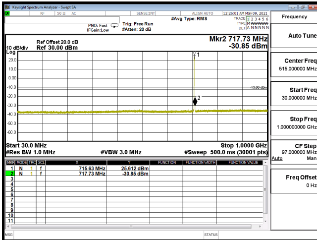
CSE-B12_1.4M-CH23173-QPSK(1,5)-30M-1G
