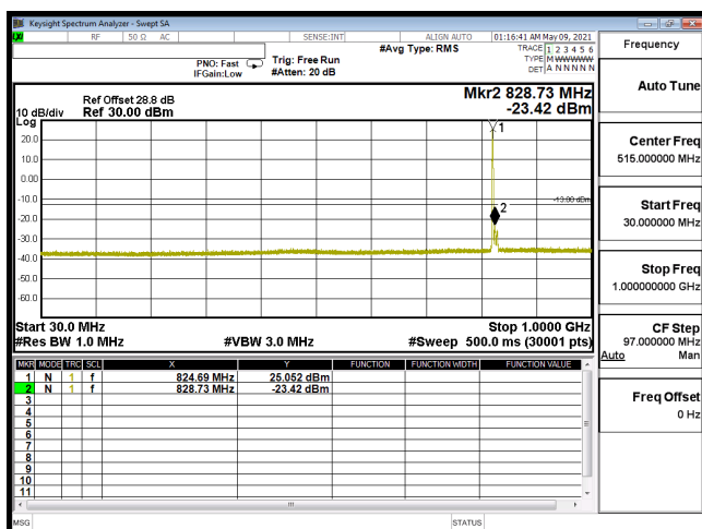
CSE-B5_10M-CH20450-64QAM(1,0)-30M-1G
