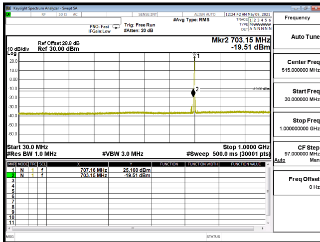
CSE-B12_1.4M-CH23095-QPSK(3,0)-30M-1G
