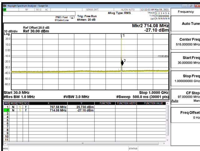
CSE-B12_3M-CH23095-16QAM(1,7)-30M-1G
