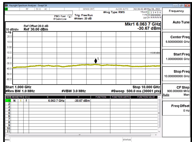
CSE-B12_3M-CH23095-16QAM(1,7)-1G-10G
