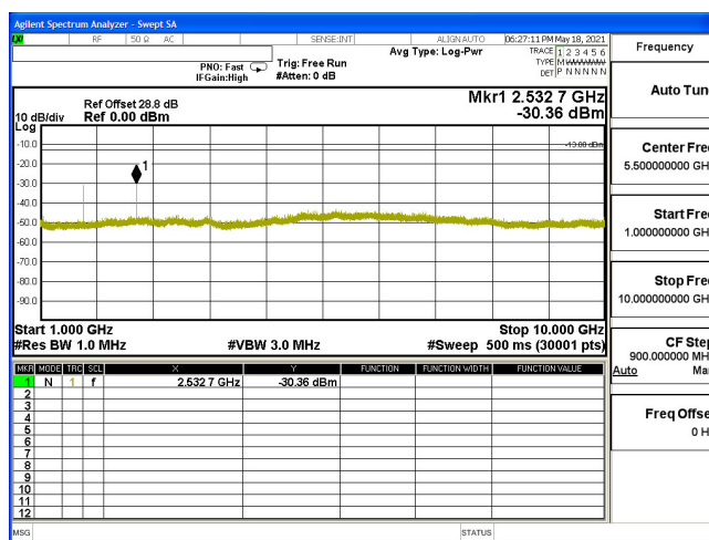
CSE-B5_5M-CH20625-16QAM(1,0)-1G-10G
