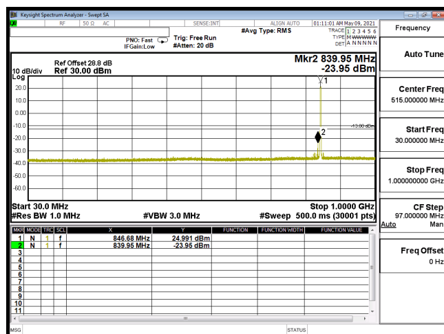
CSE-B5_5M-CH20625-QPSK(1,12)-30M-1G
