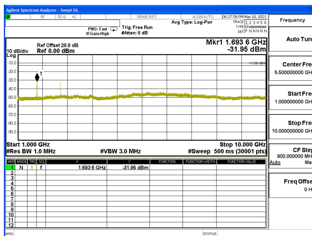
CSE-B5_5M-CH20625-64QAM(1,12)-1G-10G
