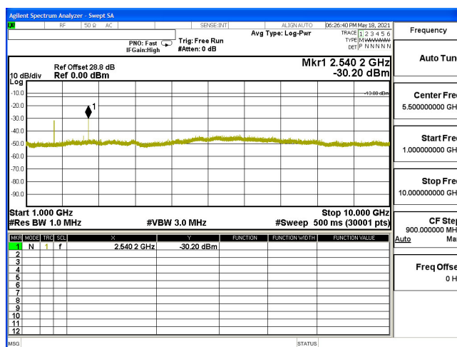
CSE-B5_5M-CH20625-QPSK(1,12)-1G-10G
