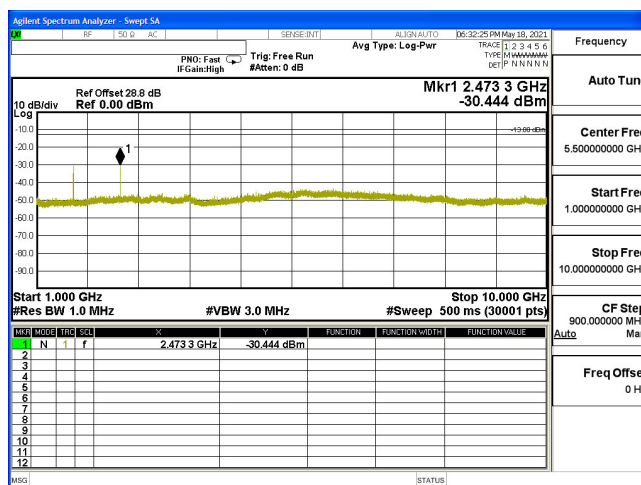
CSE-B5_10M-CH20450-64QAM(1,0)-1G-10G
