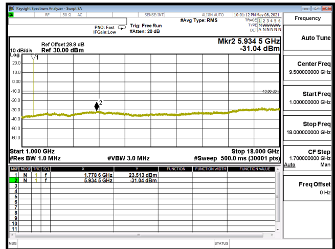
CSE-B66_3M-CH132657-QPSK(1,7)-1G-18G
