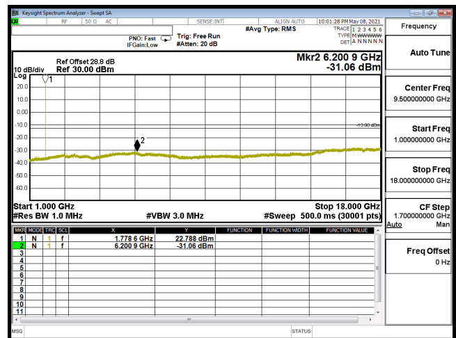
CSE-B66_3M-CH132657-16QAM(1,7)-1G-18G
