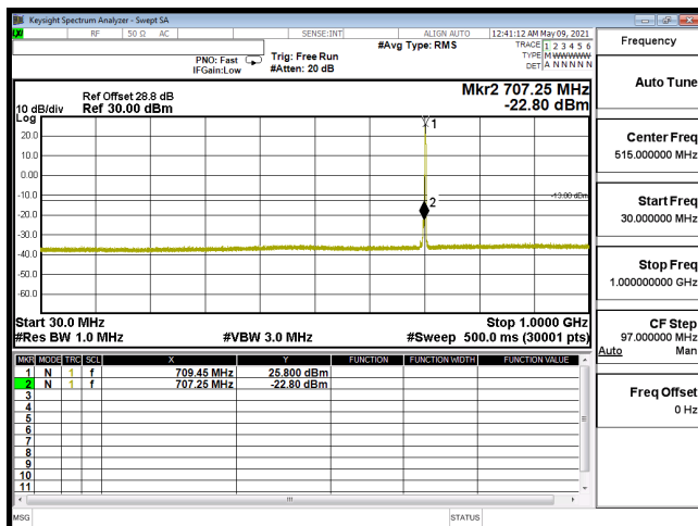
CSE-B12_5M-CH23095-16QAM(1,24)-30M-1G
