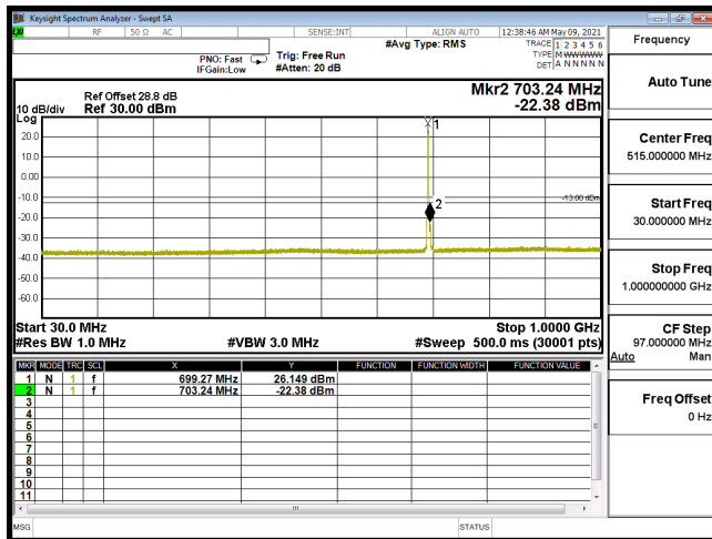
CSE-B12_5M-CH23035-QPSK(1,0)-30M-1G
