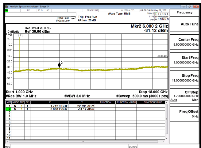
CSE-B66_3M-CH131987-64QAM(1,14)-1G-18G
