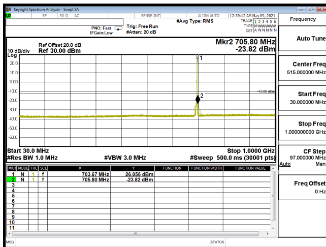
CSE-B12_5M-CH23035-16QAM(1,24)-30M-1G
