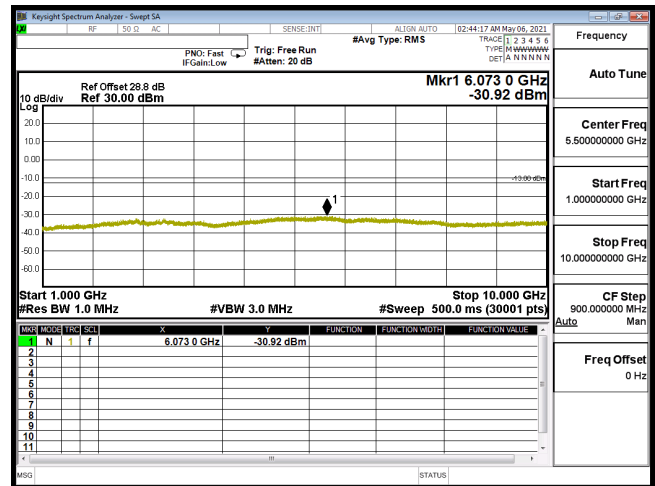
CSE-B12_5M-CH23095-QPSK(1,24)-1G-10G
