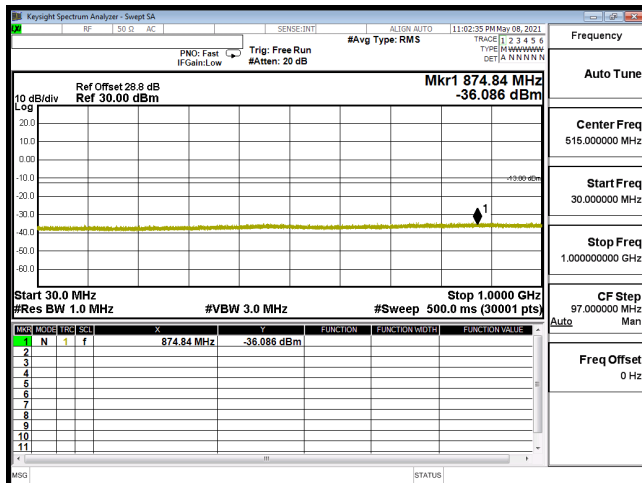
CSE-B66_3M-CH131987-QPSK(1,7)-30M-1G
