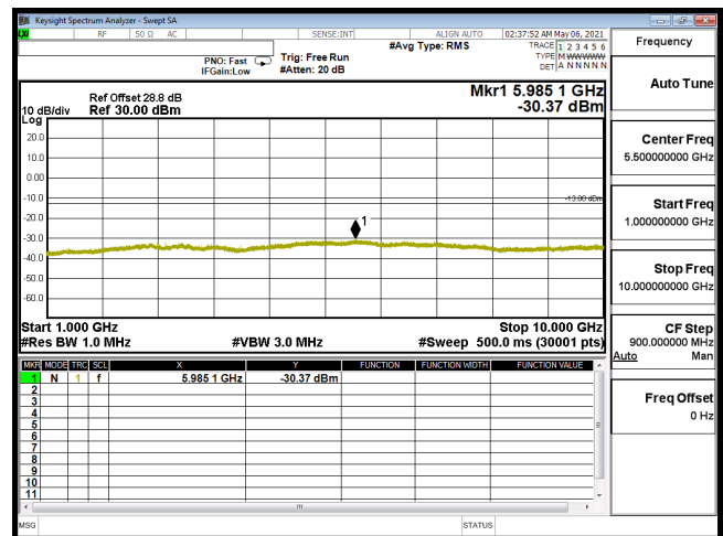
CSE-B12_3M-CH23165-16QAM(1,7)-1G-10G
