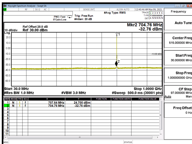
CSE-B12_5M-CH23095-64QAM(1,12)-30M-1G
