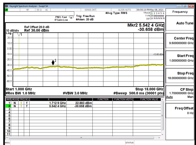
CSE-B66_3M-CH131987-16QAM(1,14)-1G-18G
