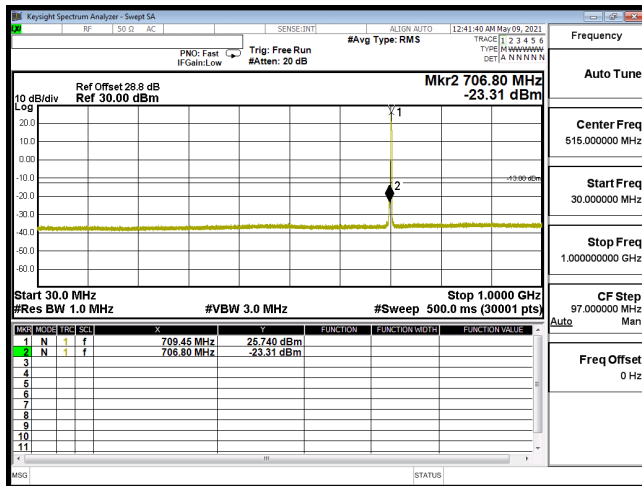
CSE-B12_5M-CH23095-QPSK(1,24)-30M-1G
