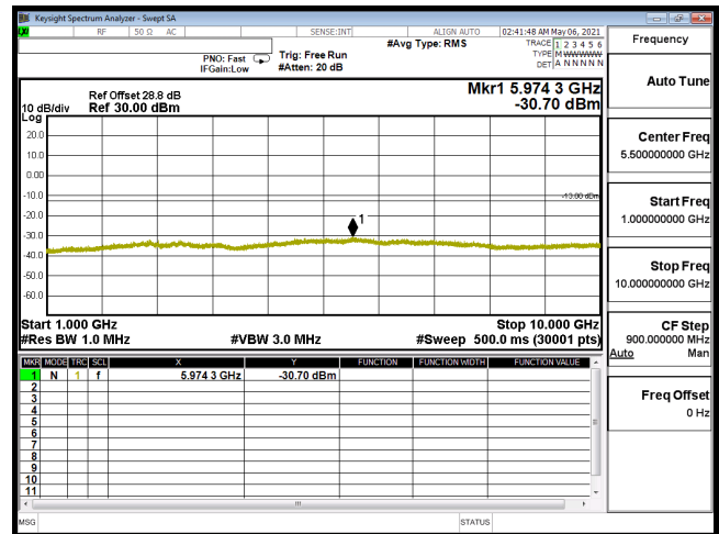
CSE-B12_5M-CH23035-QPSK(1,0)-1G-10G
