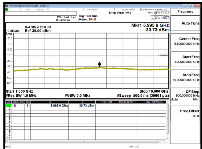
CSE-B12_5M-CH23095-16QAM(1,24)-1G-10G
