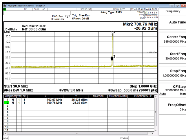
CSE-B12_5M-CH23035-64QAM(1,24)-30M-1G
