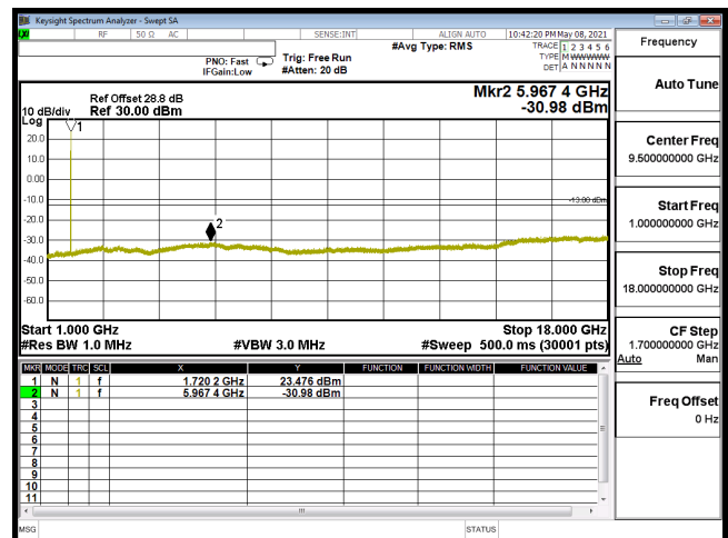
CSE-B66_20M-CH132072-16QAM(1,50)-1G-18G
