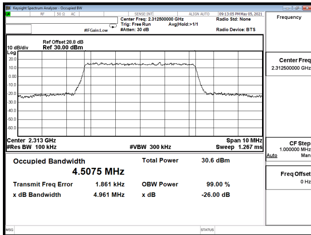
OCC-B30_5M-CH27735-QPSK
