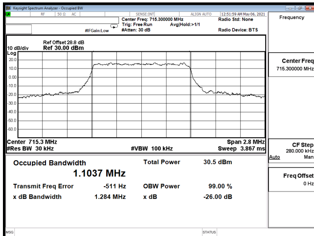
OCC-B12_1.4M-CH23173-QPSK
