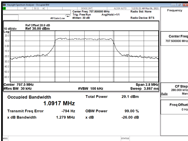
OCC-B12_1.4M-CH23095-16QAM
