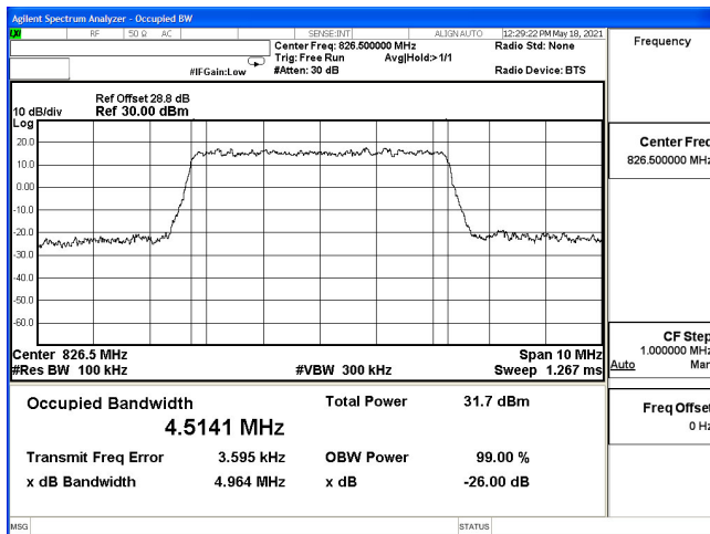
OCC-B5_5M-CH20425-QPSK
