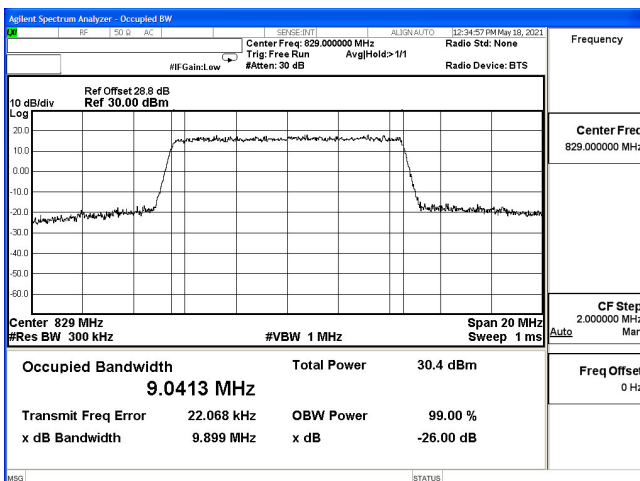
OCC-B5_10M-CH20450-16QAM
