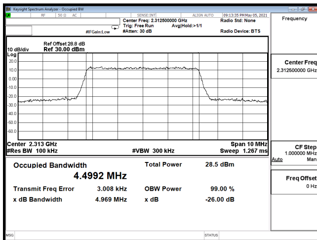
OCC-B30_5M-CH27735-64QAM
