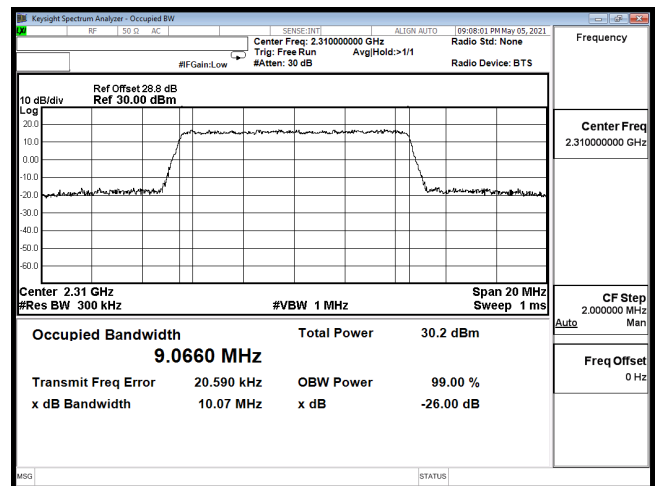
OCC-B30_10M-CH27710-QPSK
