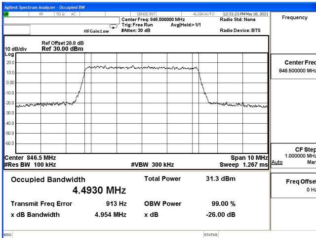
OCC-B5_5M-CH20625-QPSK
