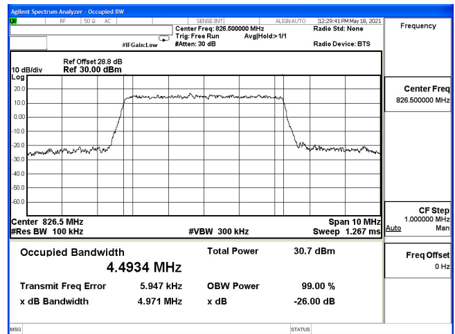
OCC-B5_5M-CH20425-16QAM
