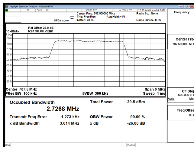
OCC-B12_3M-CH23095-16QAM
