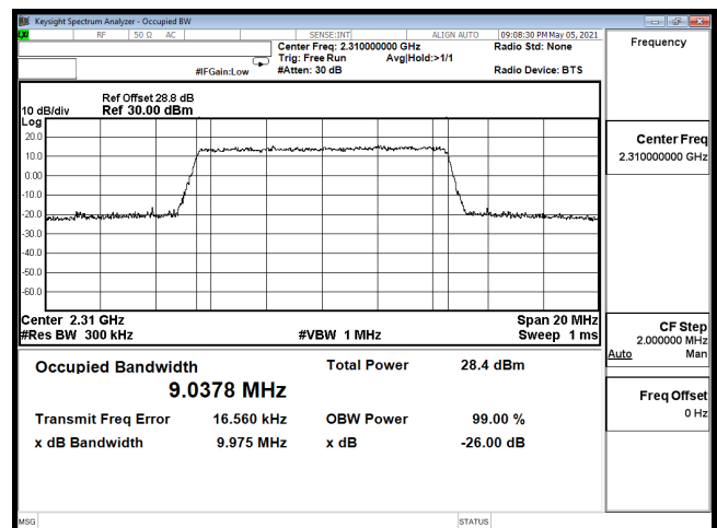
OCC-B30_10M-CH27710-64QAM
