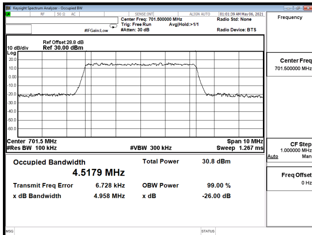
OCC-B12_5M-CH23035-QPSK
