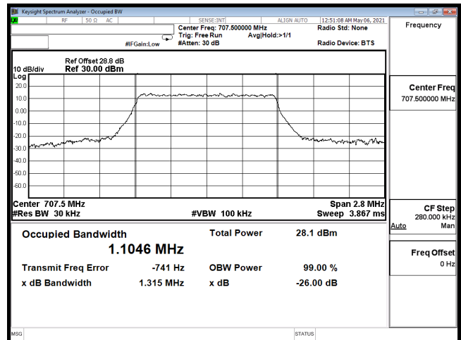
OCC-B12_1.4M-CH23095-64QAM
