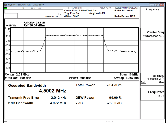
OCC-B30_5M-CH27710-64QAM
