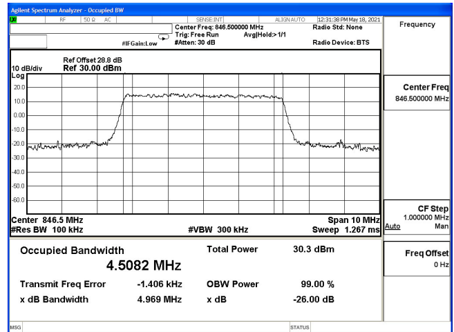
OCC-B5_5M-CH20625-16QAM
