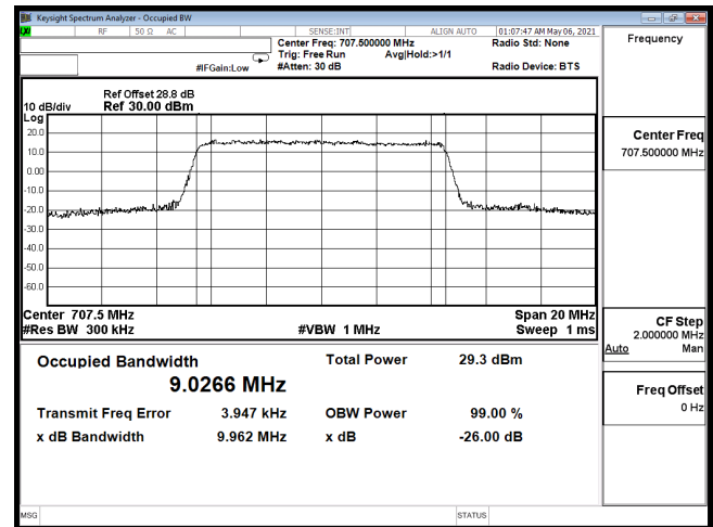
OCC-B12_10M-CH23095-16QAM
