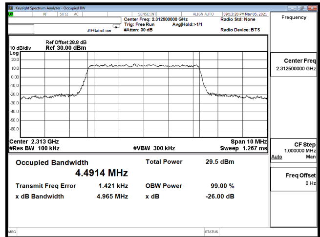
OCC-B30_5M-CH27735-16QAM
