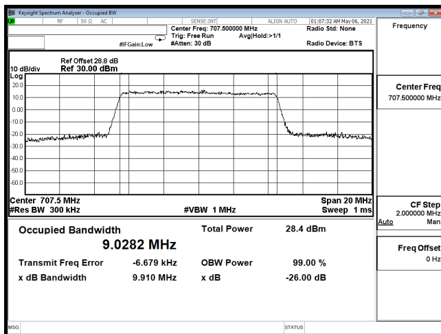
OCC-B12_10M-CH23095-64QAM
