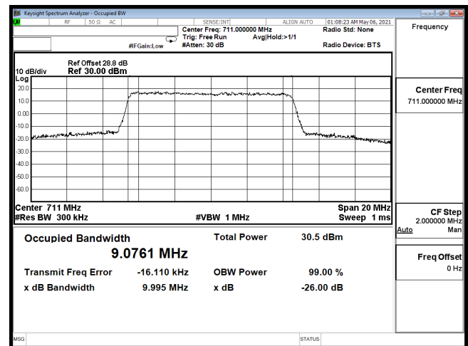
OCC-B12_10M-CH23130-16QAM
