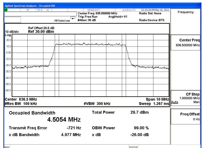
OCC-B5_5M-CH20525-64QAM
