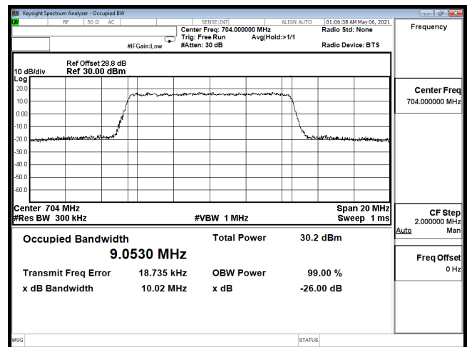
OCC-B12_10M-CH23060-QPSK
