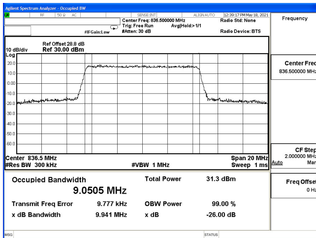
OCC-B5_10M-CH20525-QPSK
