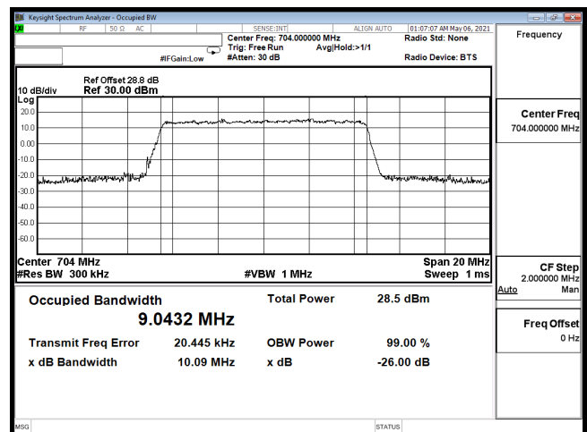
OCC-B12_10M-CH23060-64QAM
