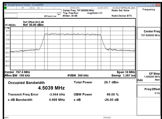
OCC-B12_5M-CH23095-64QAM
