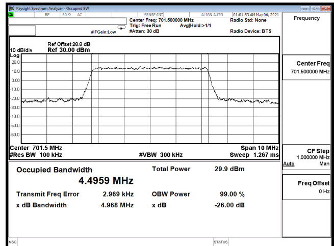
OCC-B12_5M-CH23035-16QAM
