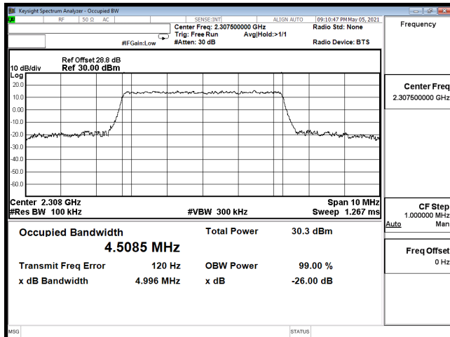
OCC-B30_5M-CH27685-QPSK
