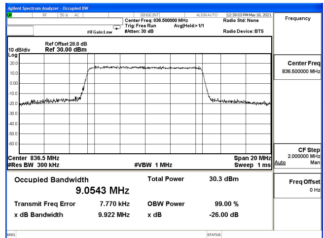
OCC-B5_10M-CH20525-16QAM
