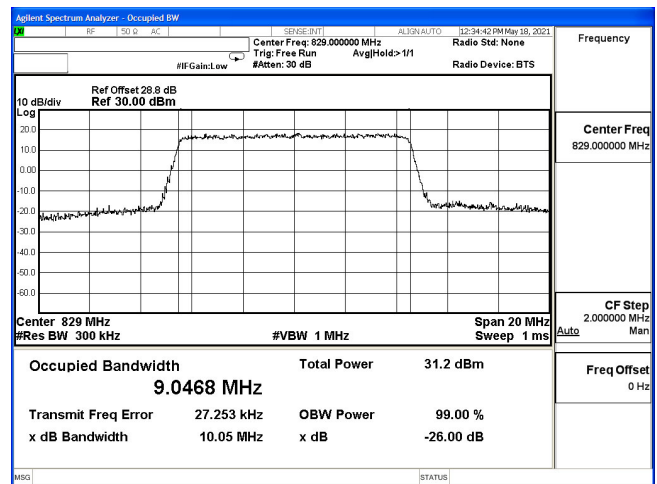
OCC-B5_10M-CH20450-QPSK
