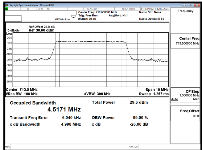
OCC-B12_5M-CH23155-16QAM
