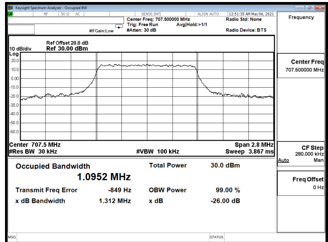
OCC-B12_1.4M-CH23095-QPSK
