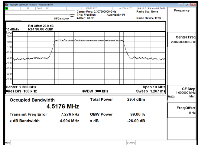
OCC-B30_5M-CH27685-16QAM
