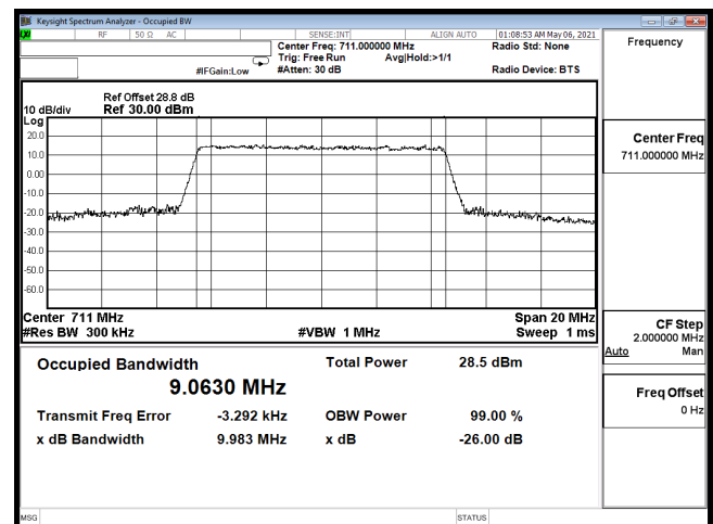
OCC-B12_10M-CH23130-64QAM
