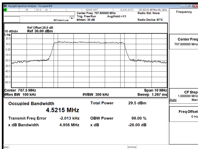
OCC-B12_5M-CH23095-16QAM
