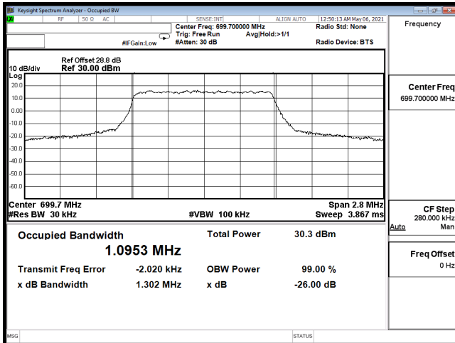
OCC-B12_1.4M-CH23017-QPSK
