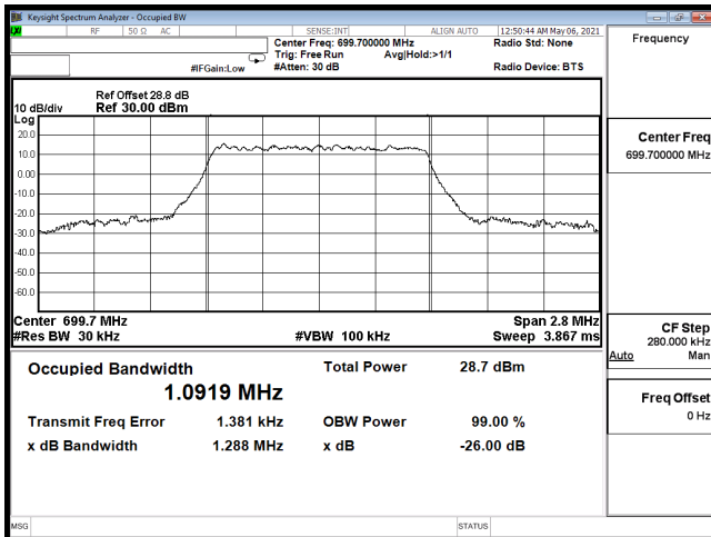
OCC-B12_1.4M-CH23017-64QAM
