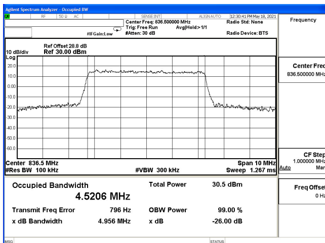
OCC-B5_5M-CH20525-16QAM
