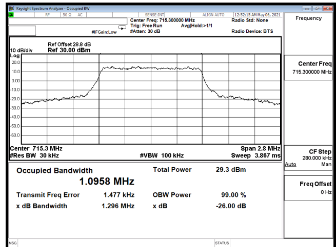
OCC-B12_1.4M-CH23173-16QAM
