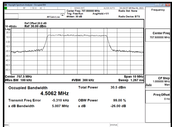
OCC-B12_5M-CH23095-QPSK
