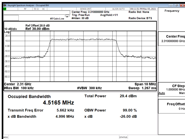
OCC-B30_5M-CH27710-16QAM
