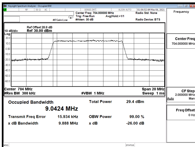
OCC-B12_10M-CH23060-16QAM
