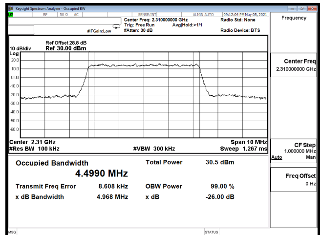
OCC-B30_5M-CH27710-QPSK
