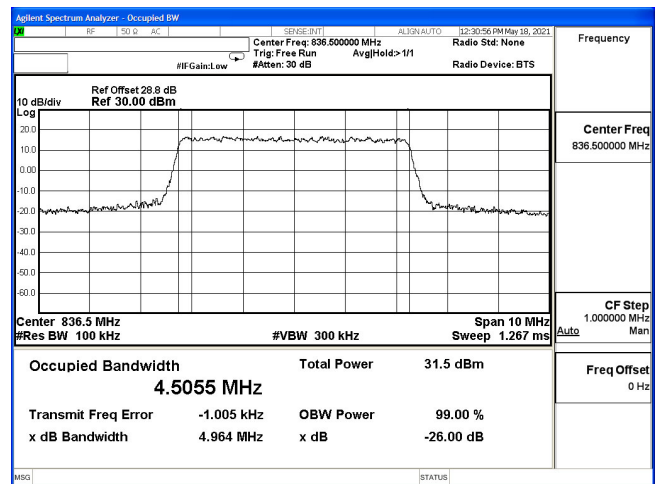
OCC-B5_5M-CH20525-QPSK
