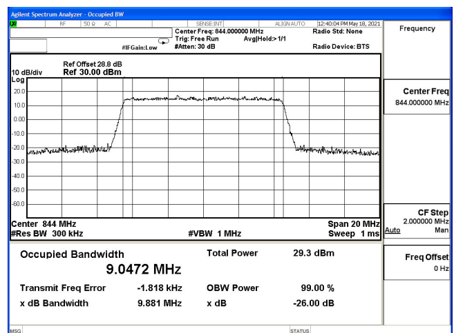
OCC-B5_10M-CH20600-64QAM
