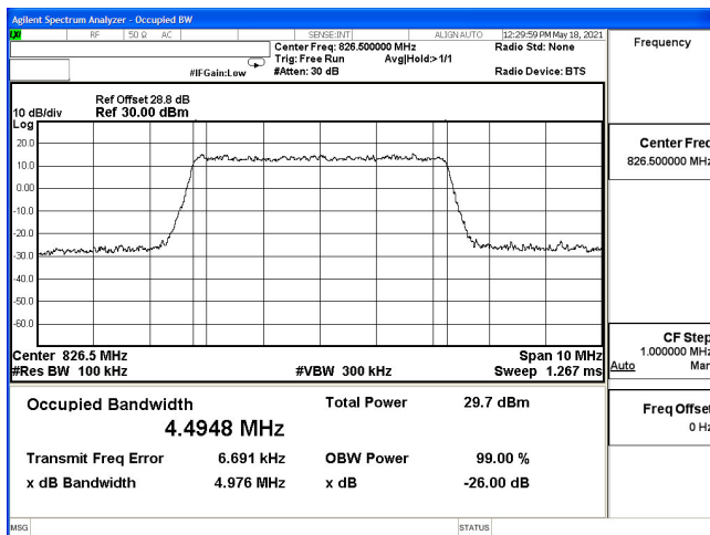
OCC-B5_5M-CH20425-64QAM
