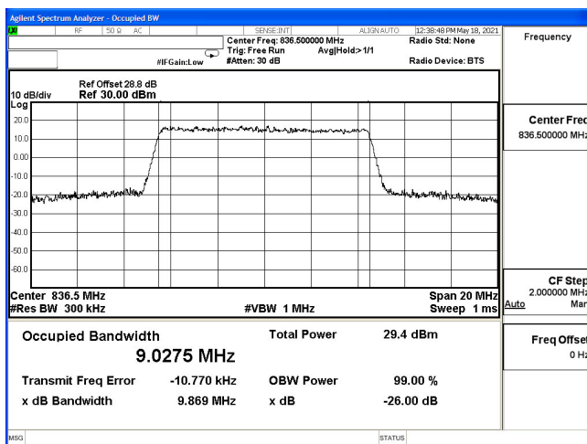
OCC-B5_10M-CH20525-64QAM
