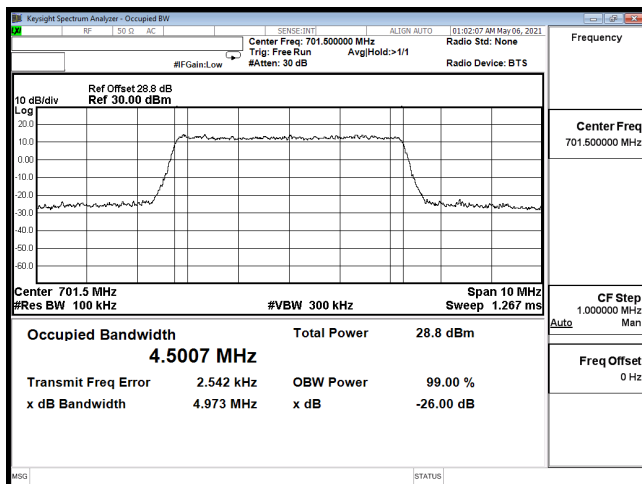
OCC-B12_5M-CH23035-64QAM
