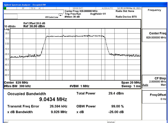
OCC-B5_10M-CH20450-64QAM
