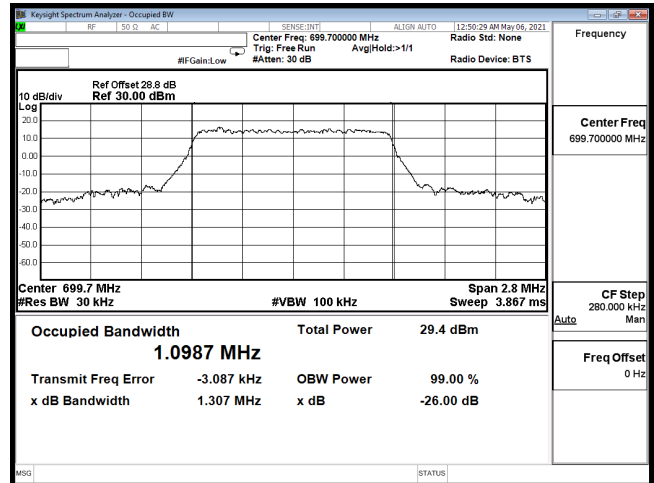
OCC-B12_1.4M-CH23017-16QAM
