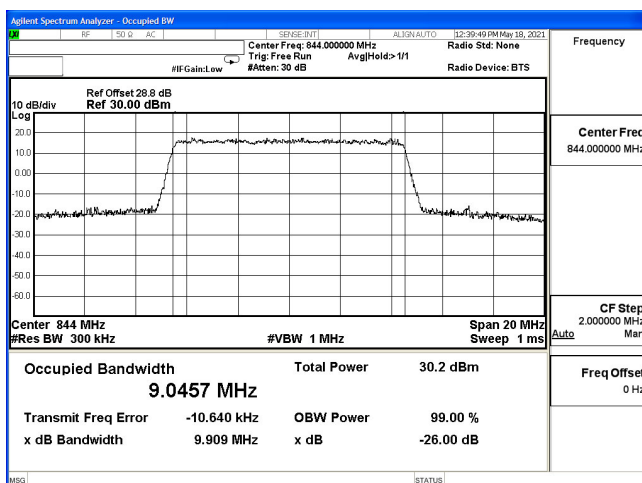
OCC-B5_10M-CH20600-16QAM
