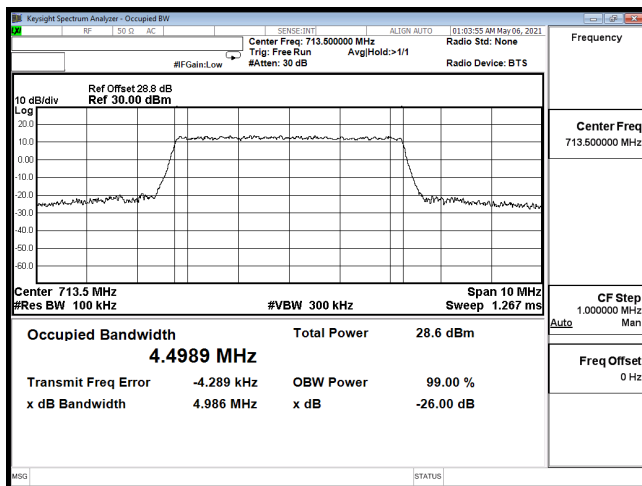
OCC-B12_5M-CH23155-64QAM
