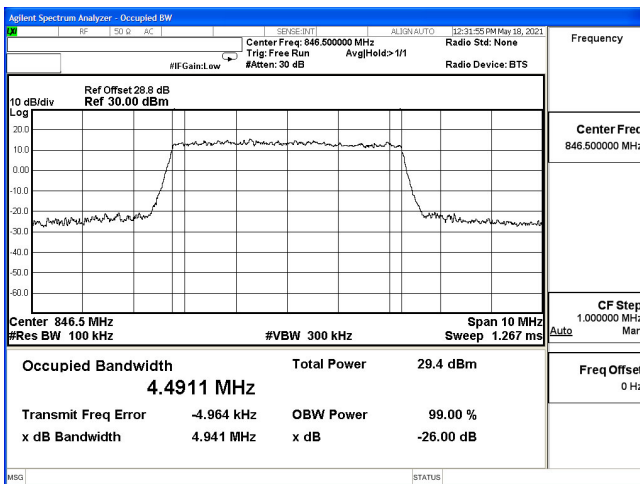
OCC-B5_5M-CH20625-64QAM
