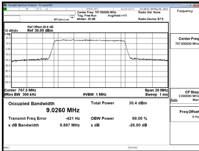
OCC-B12_10M-CH23095-QPSK
