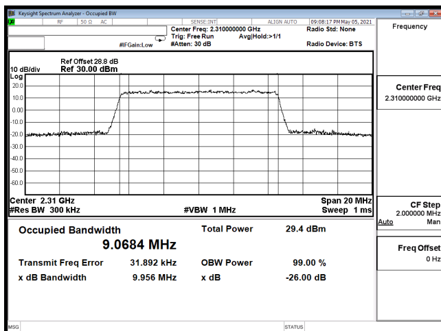
OCC-B30_10M-CH27710-16QAM
