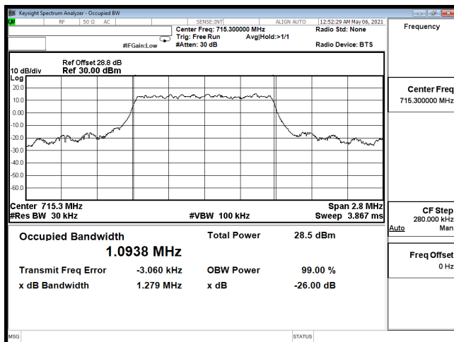
OCC-B12_1.4M-CH23173-64QAM
