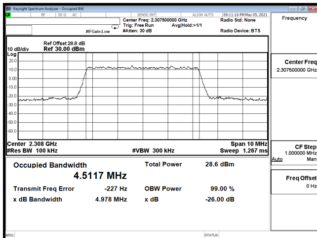
OCC-B30_5M-CH27685-64QAM
