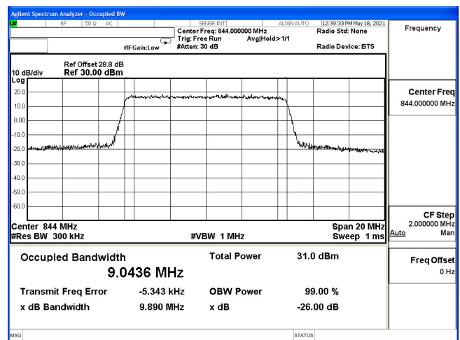
OCC-B5_10M-CH20600-QPSK
