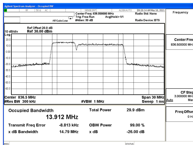
OCC(5M+10M)-2ULCA_5B-QPSK_831.8(25,0)+839(50,0)
