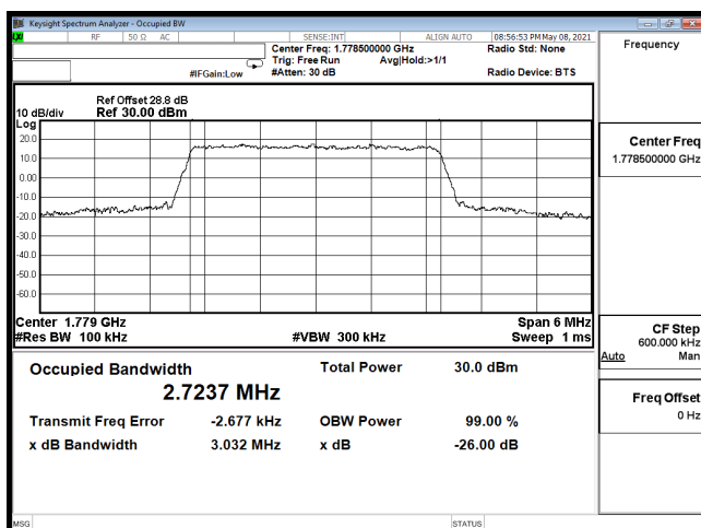
OCC-B66_3M-CH132657-16QAM
