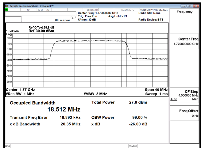
OCC-B66_20M-CH132572-64QAM
