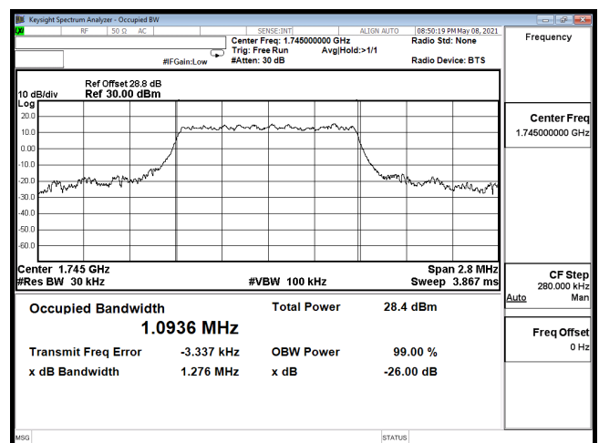
OCC-B66_1.4M-CH132322-64QAM
