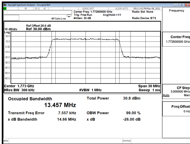
OCC-B66_15M-CH132597-QPSK
