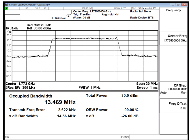
OCC-B66_15M-CH132597-16QAM
