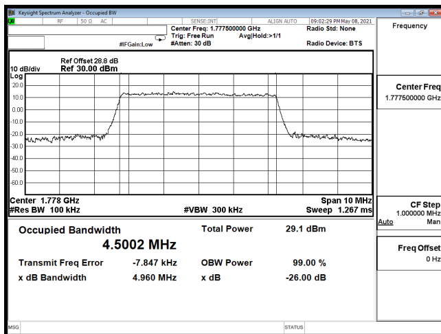
OCC-B66_5M-CH132647-64QAM
