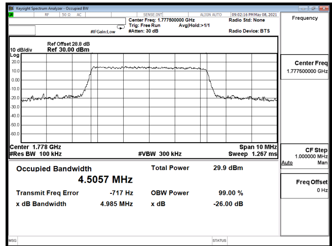
OCC-B66_5M-CH132647-16QAM
