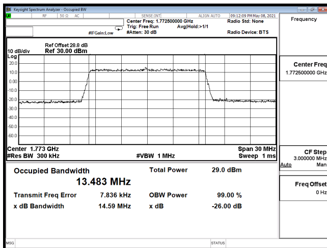
OCC-B66_15M-CH132597-64QAM
