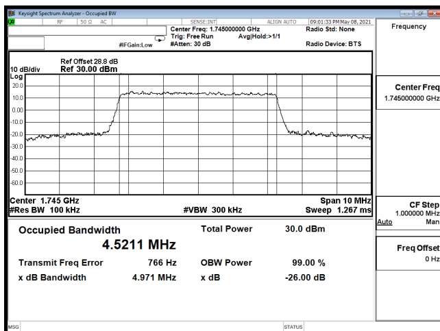
OCC-B66_5M-CH132322-16QAM
