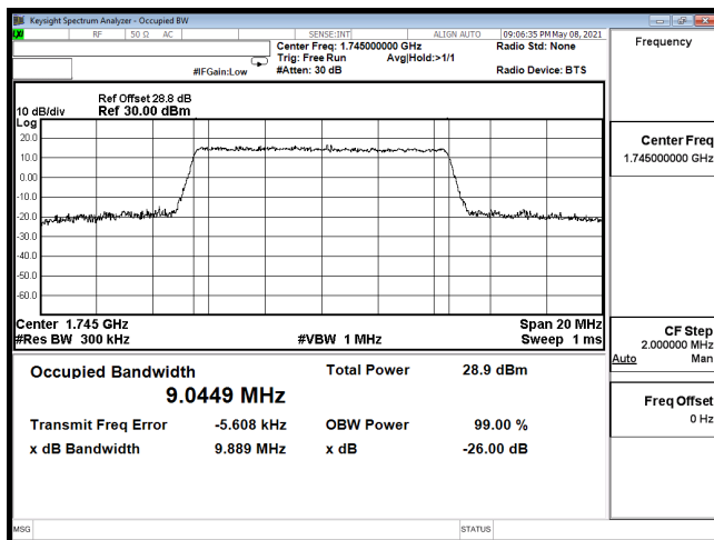
OCC-B66_10M-CH132322-64QAM
