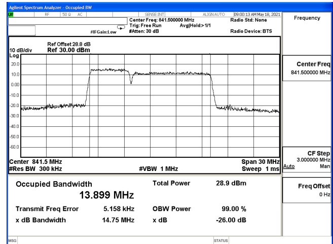
OCC(5M+10M)-2ULCA_5B-16QAM_836.8(25,0)+844(50,0)
