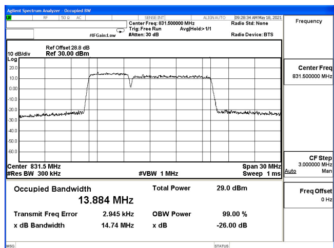
OCC(5M+10M)-2ULCA_5B-64QAM_826.8(25,0)+834(50,0)
