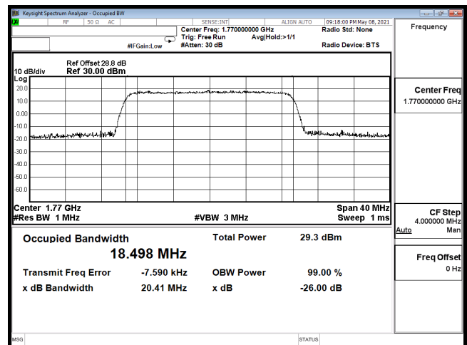
OCC-B66_20M-CH132572-QPSK
