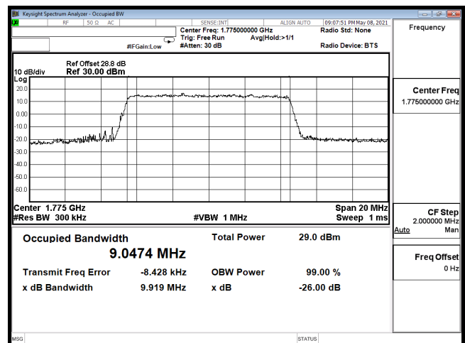
OCC-B66_10M-CH132622-64QAM
