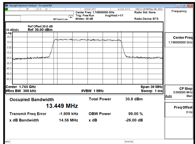
OCC-B66_15M-CH132322-QPSK
