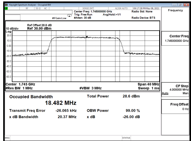
OCC-B66_20M-CH132322-16QAM
