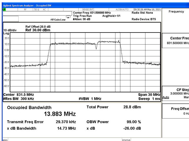
OCC(10M+5M)-2ULCA_5B-16QAM_829(50,0)+836.2(25,0)
