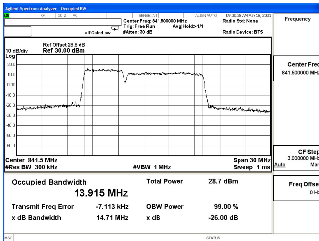
OCC(5M+10M)-2ULCA_5B-64QAM_836.8(25,0)+844(50,0)
