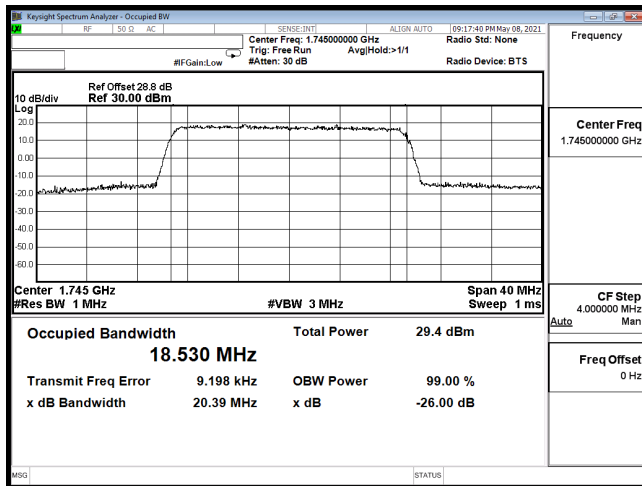
OCC-B66_20M-CH132322-QPSK
