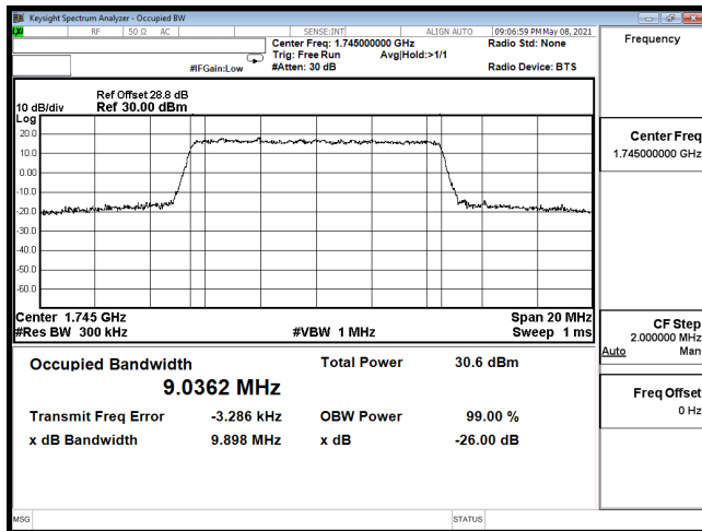
OCC-B66_10M-CH132322-QPSK
