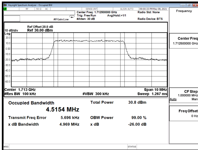
OCC-B66_5M-CH131997-QPSK
