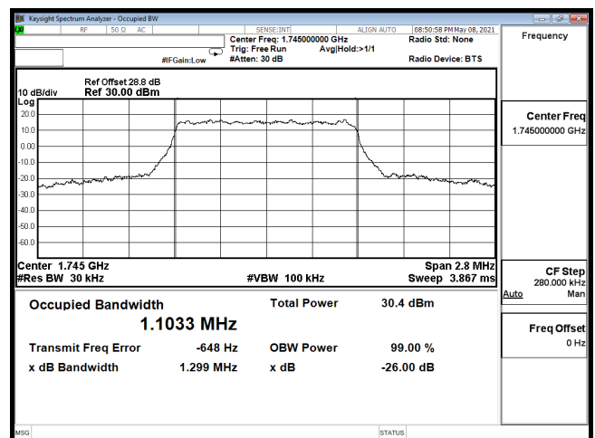
OCC-B66_1.4M-CH132322-QPSK
