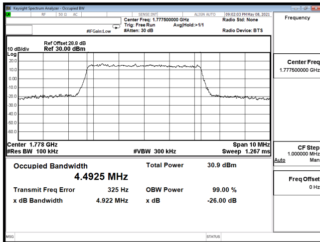
OCC-B66_5M-CH132647-QPSK
