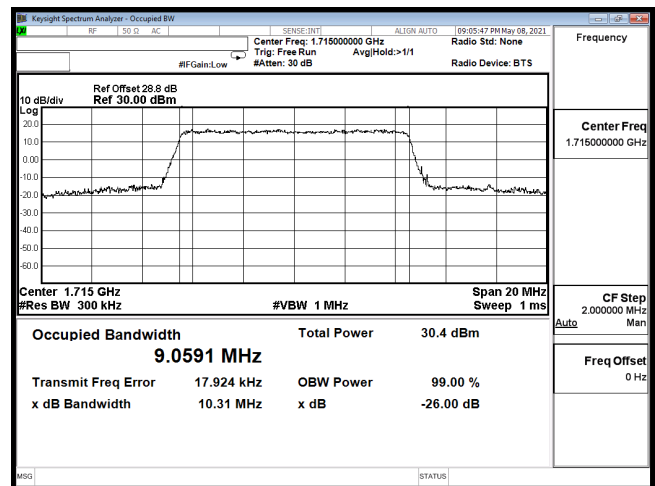
OCC-B66_10M-CH132022-QPSK
