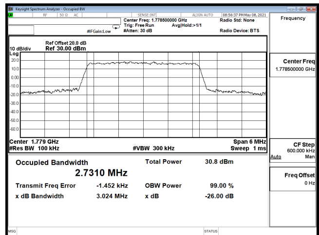
OCC-B66_3M-CH132657-QPSK
