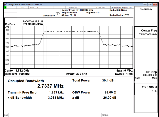
OCC-B66_3M-CH131987-QPSK
