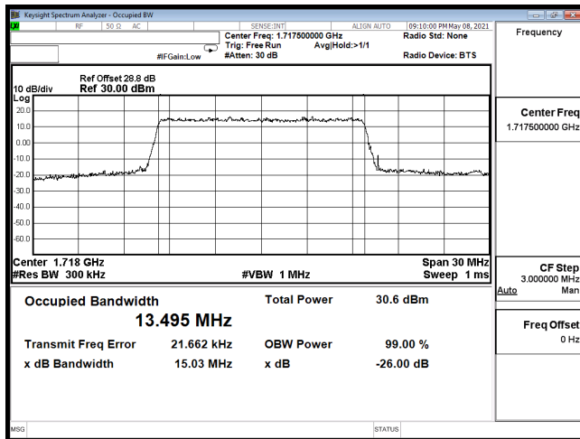
OCC-B66_15M-CH132047-QPSK
