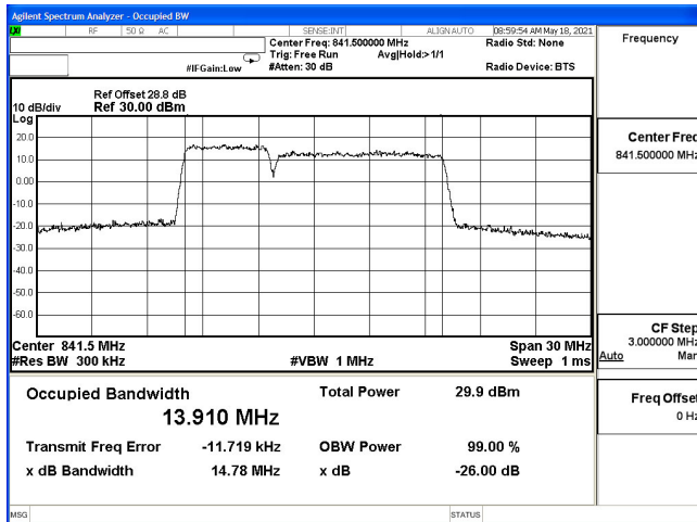
OCC(5M+10M)-2ULCA_5B-QPSK_836.8(25,0)+844(50,0)
