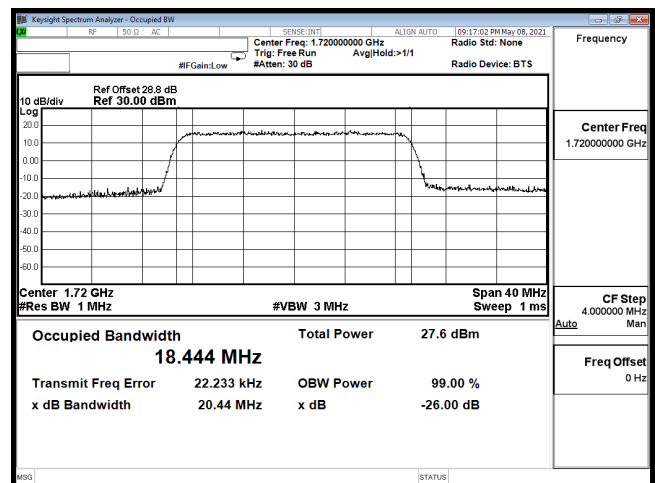
OCC-B66_20M-CH132072-64QAM
