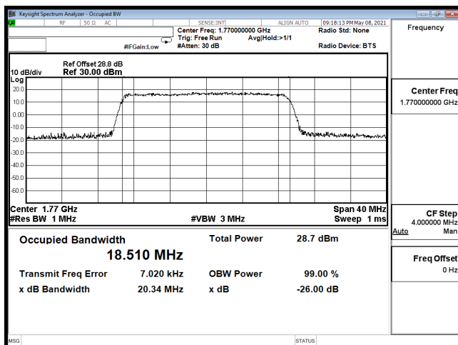
OCC-B66_20M-CH132572-16QAM
