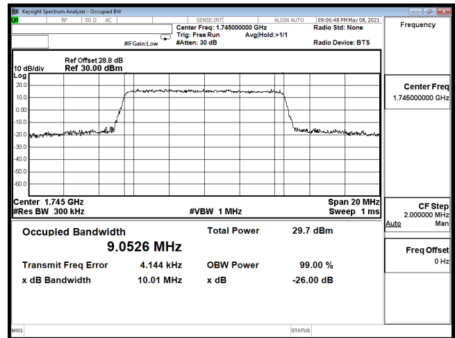
OCC-B66_10M-CH132322-16QAM
