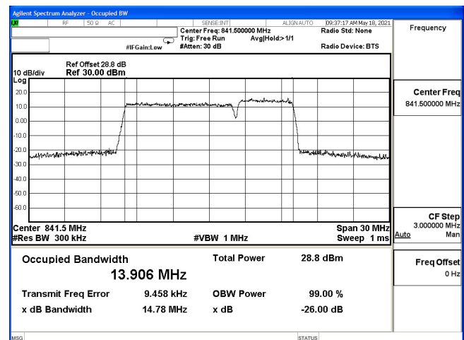
OCC(10M+5M)-2ULCA_5B-64QAM_839(50,0)+846.2(25,0)
