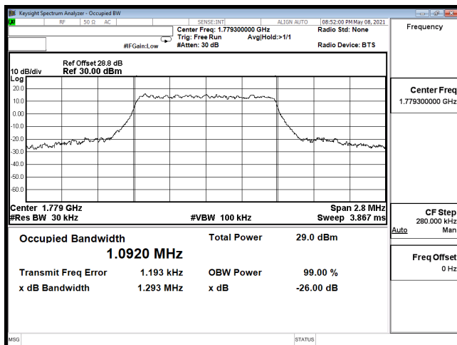
OCC-B66_1.4M-CH132665-64QAM
