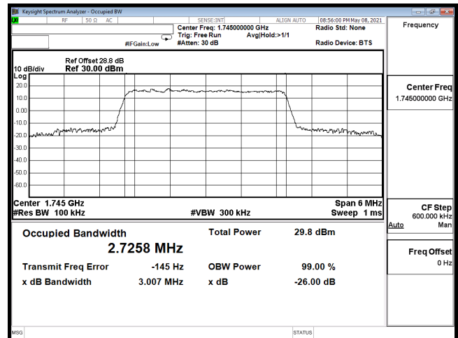
OCC-B66_3M-CH132322-16QAM
