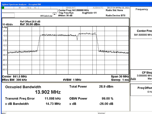
OCC(10M+5M)-2ULCA_5B-16QAM_839(50,0)+846.2(25,0)
