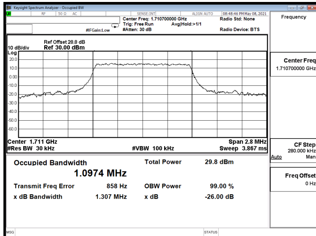
OCC-B66_1.4M-CH131979-QPSK
