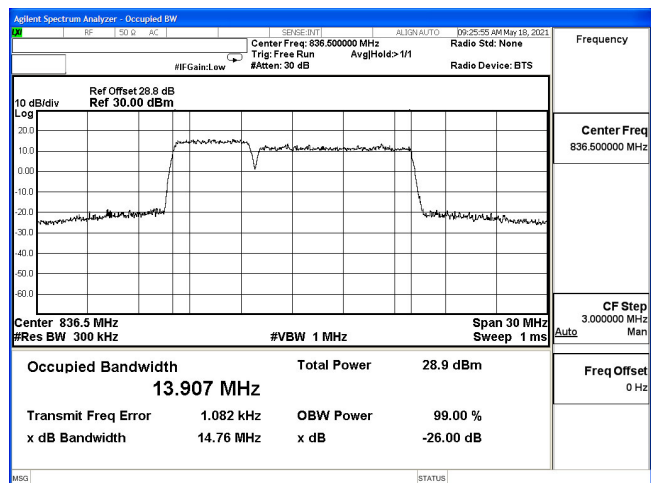
OCC(5M+10M)-2ULCA_5B-16QAM_831.8(25,0)+839(50,0)
