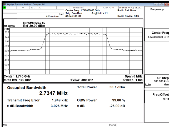
OCC-B66_3M-CH132322-QPSK
