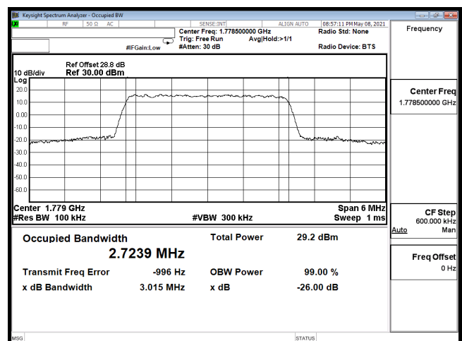
OCC-B66_3M-CH132657-64QAM
