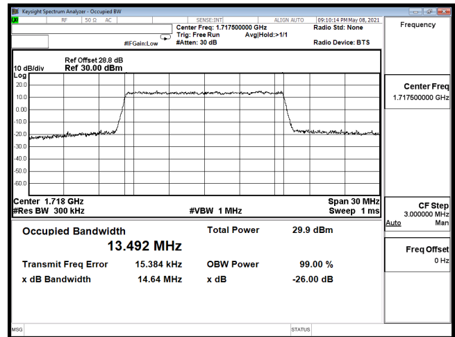
OCC-B66_15M-CH132047-16QAM
