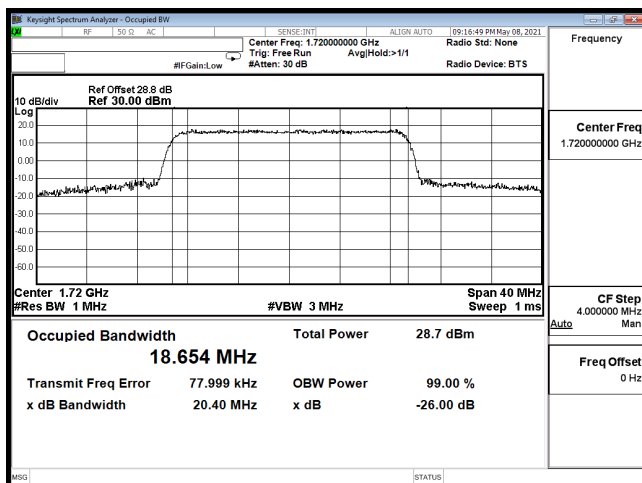
OCC-B66_20M-CH132072-16QAM
