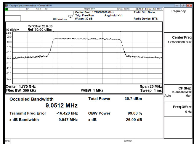
OCC-B66_10M-CH132622-QPSK
