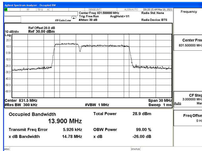
OCC(5M+10M)-2ULCA_5B-16QAM_826.8(25,0)+834(50,0)
