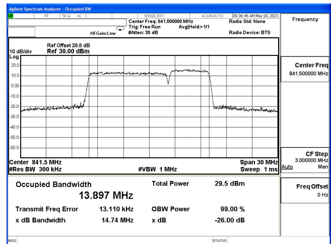
OCC(10M+5M)-2ULCA_5B-QPSK_839(50,0)+846.2(25,0)
