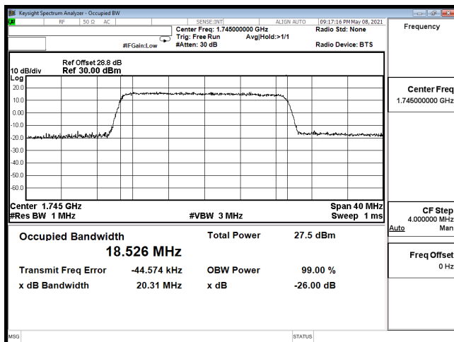
OCC-B66_20M-CH132322-64QAM
