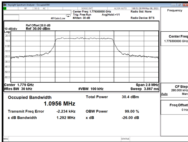
OCC-B66_1.4M-CH132665-QPSK
