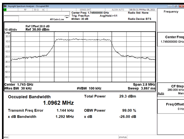
OCC-B66_1.4M-CH132322-16QAM
