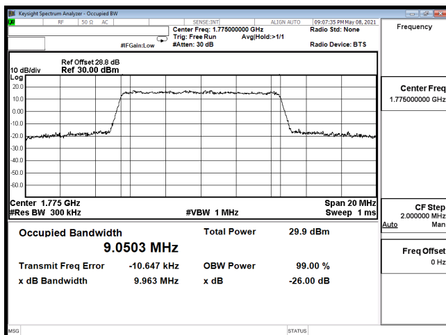
OCC-B66_10M-CH132622-16QAM
