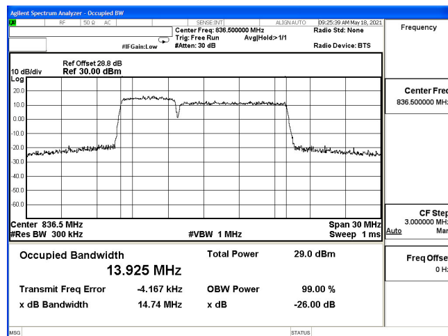
OCC(5M+10M)-2ULCA_5B-64QAM_831.8(25,0)+839(50,0)
