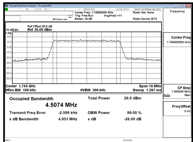
OCC-B66_5M-CH132322-64QAM
