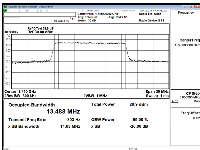
OCC-B66_15M-CH132322-16QAM
