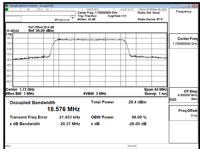
OCC-B66_20M-CH132072-QPSK
