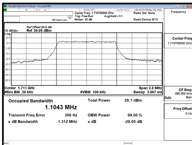
OCC-B66_1.4M-CH131979-64QAM
