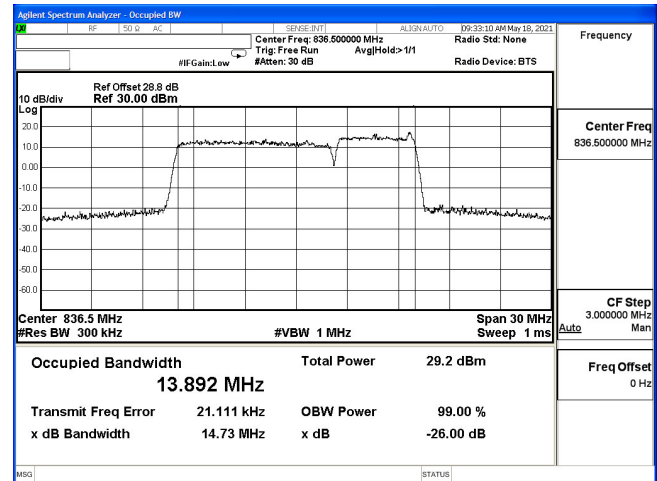
OCC(10M+5M)-2ULCA_5B-16QAM_834(50,0)+841.2(25,0)
