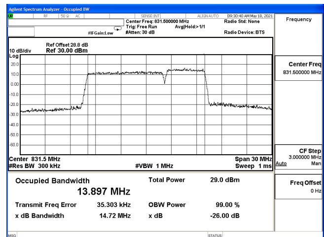
OCC(10M+5M)-2ULCA_5B-64QAM_829(50,0)+836.2(25,0)
