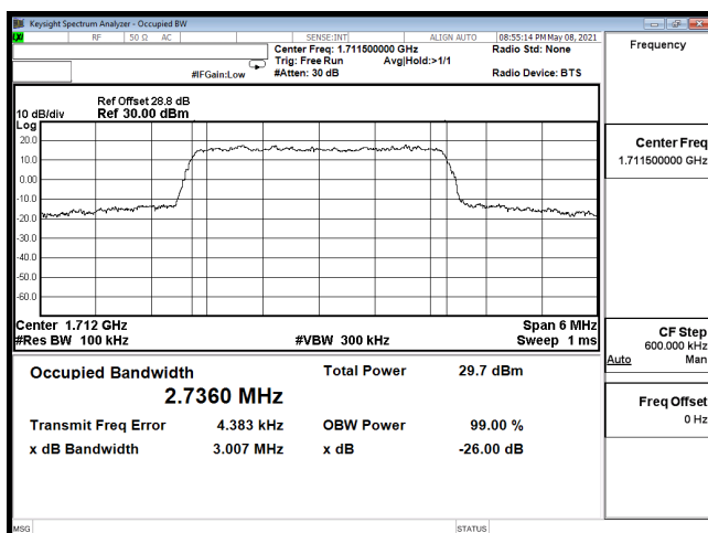
OCC-B66_3M-CH131987-16QAM
