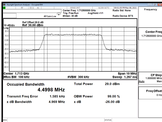
OCC-B66_5M-CH131997-64QAM
