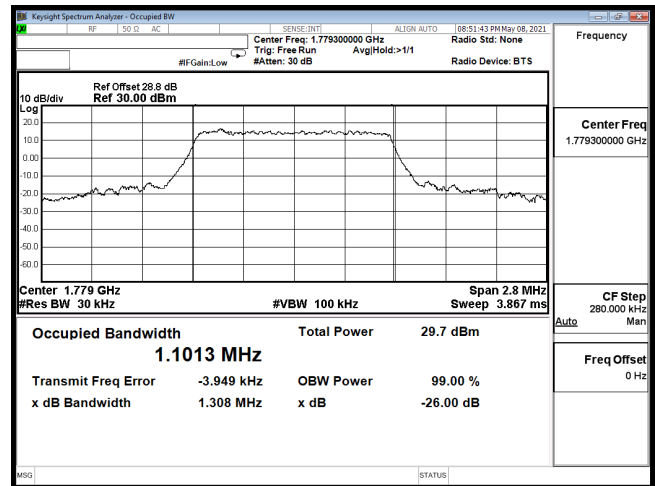
OCC-B66_1.4M-CH132665-16QAM
