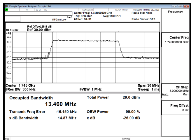
OCC-B66_15M-CH132322-64QAM
