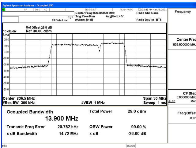
OCC(10M+5M)-2ULCA_5B-64QAM_834(50,0)+841.2(25,0)
