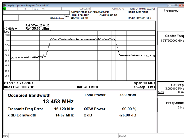
OCC-B66_15M-CH132047-64QAM
