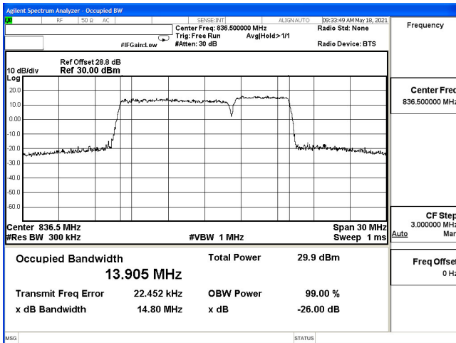
OCC(10M+5M)-2ULCA_5B-QPSK_834(50,0)+841.2(25,0)
