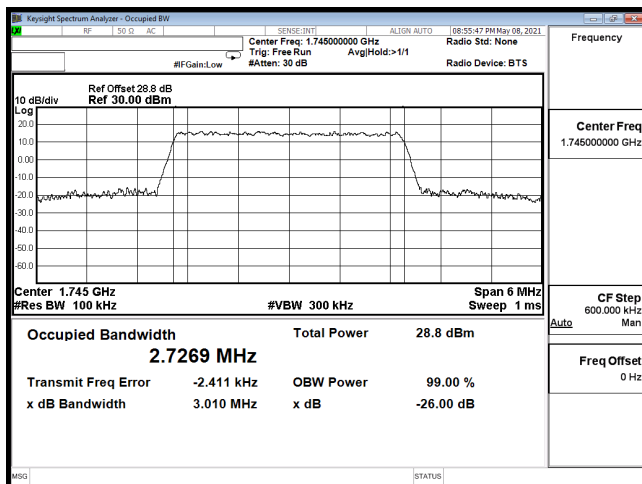
OCC-B66_3M-CH132322-64QAM
