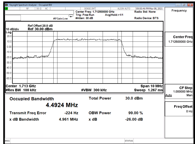
OCC-B66_5M-CH131997-16QAM
