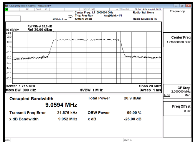
OCC-B66_10M-CH132022-64QAM
