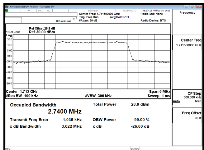
OCC-B66_3M-CH131987-64QAM
