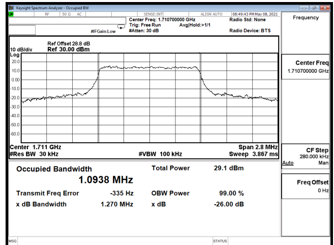
OCC-B66_1.4M-CH131979-16QAM
