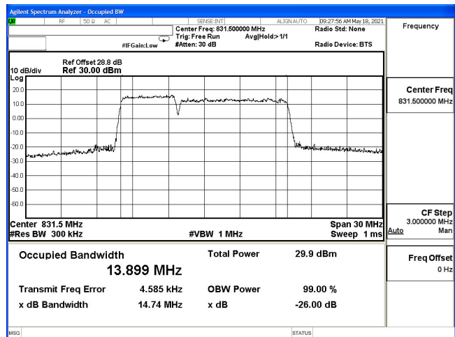
OCC(5M+10M)-2ULCA_5B-QPSK_826.8(25,0)+834(50,0)
