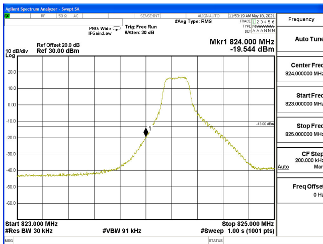
EDGE-B5_3M-CH20415-16QAM(1,0)
