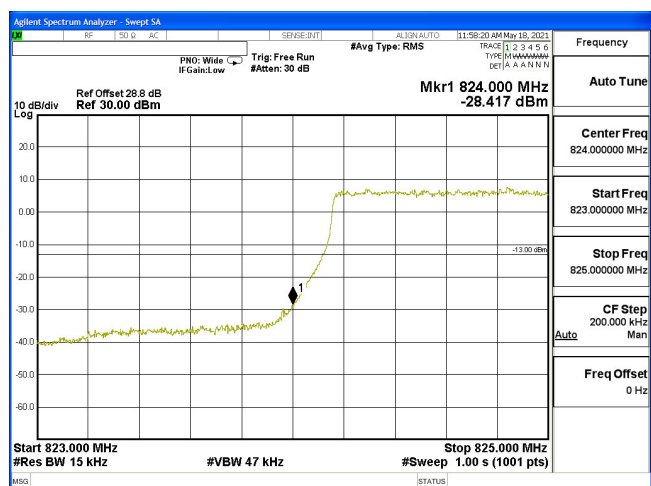
EDGE-B5_1.4M-CH20407-QPSK(6,0)
