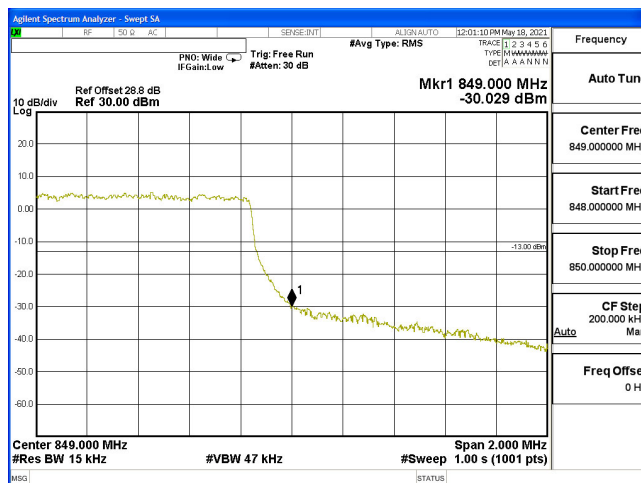
EDGE-B5_1.4M-CH20643-64QAM(6,0)
