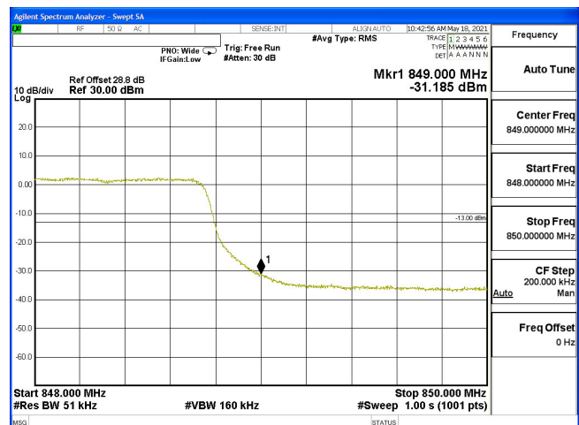
EDGE-B5_5M-CH20625-64QAM(25,0)
