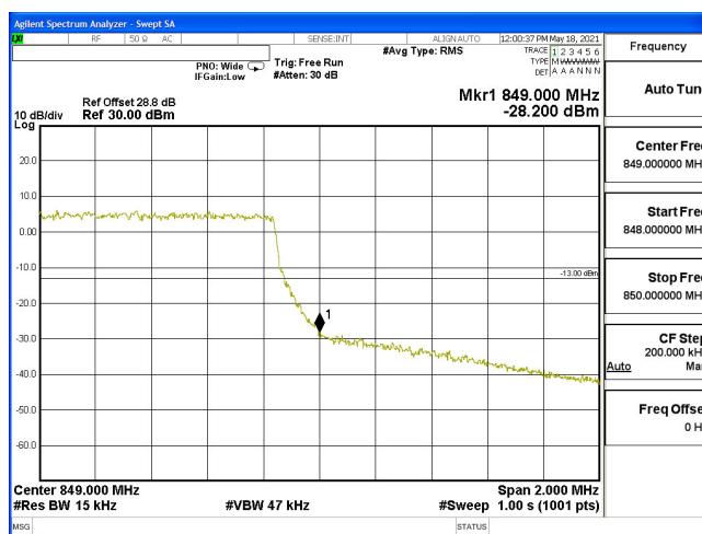
EDGE-B5_1.4M-CH20643-16QAM(6,0)
