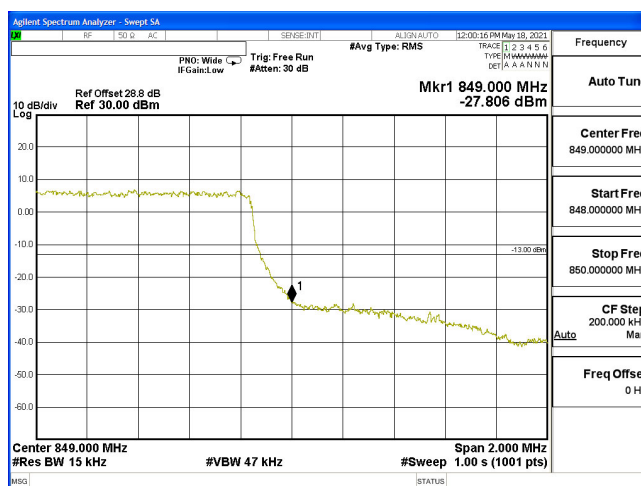
EDGE-B5_1.4M-CH20643-QPSK(6,0)
