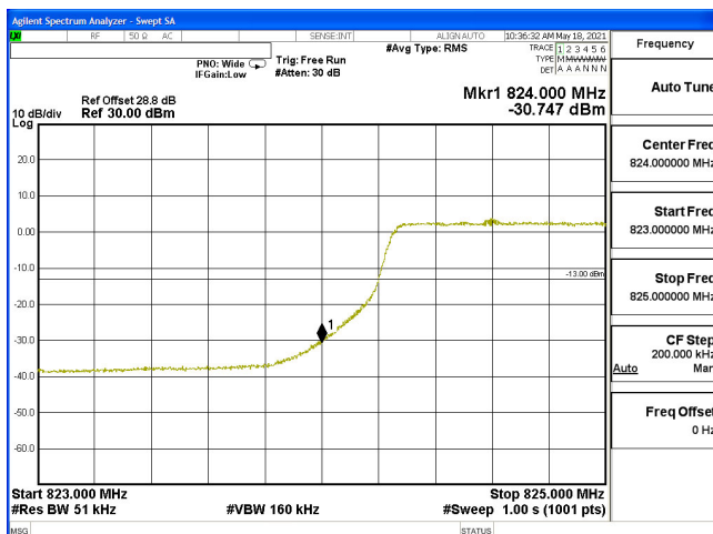
EDGE-B5_5M-CH20425-64QAM(25,0)
