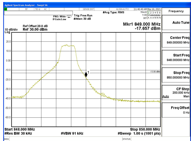
EDGE-B5_3M-CH20635-16QAM(1,14)
