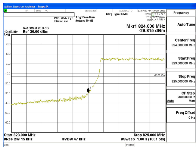
EDGE-B5_1.4M-CH20407-16QAM(6,0)
