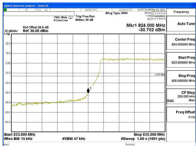
EDGE-B5_1.4M-CH20407-64QAM(6,0)
