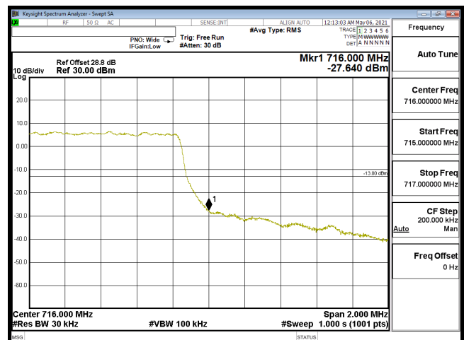
EDGE-B12_1.4M-CH23173-64QAM(6,0)
