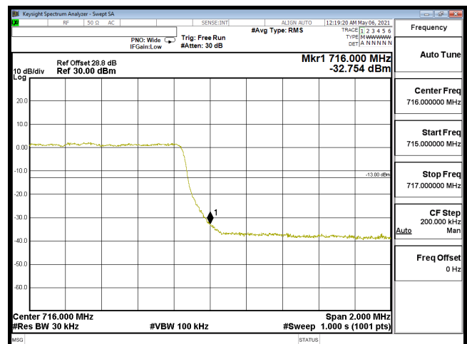
EDGE-B12_3M-CH23165-64QAM(15,0)
