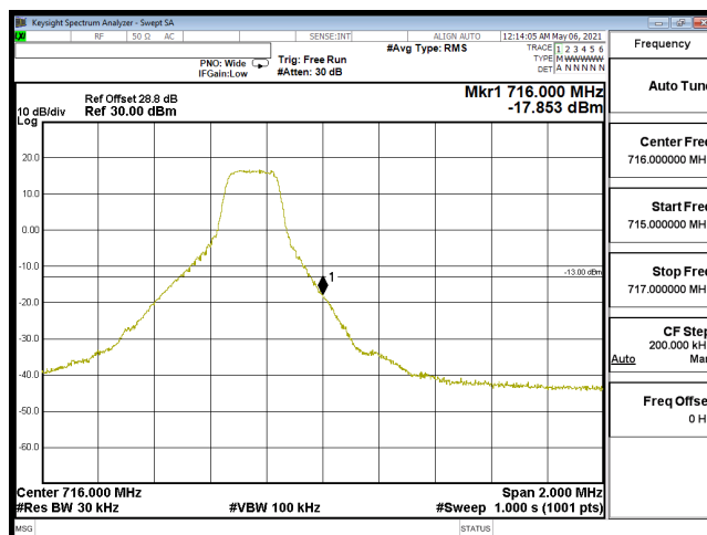
EDGE-B12_1.4M-CH23173-QPSK(1,5)
