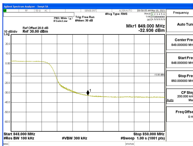
EDGE-B5_10M-CH20600-16QAM(50,0)
