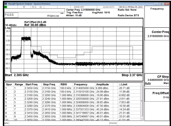
EDGE-B30_5M-CH27735-QPSK(25,0)
