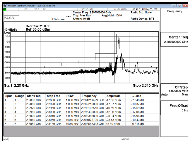
EDGE-B30_10M-CH27710-64QAM(1,0)
