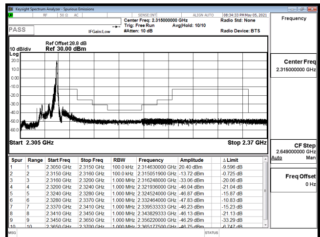
EDGE-B30_5M-CH27735-16QAM(1,24)
