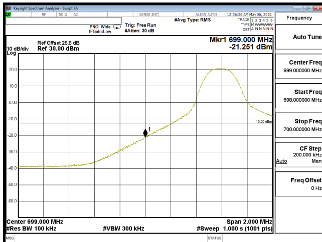
EDGE-B12_10M-CH23060-QPSK(1,0)
