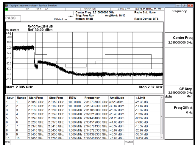
EDGE-B30_10M-CH27710-16QAM(50,0)
