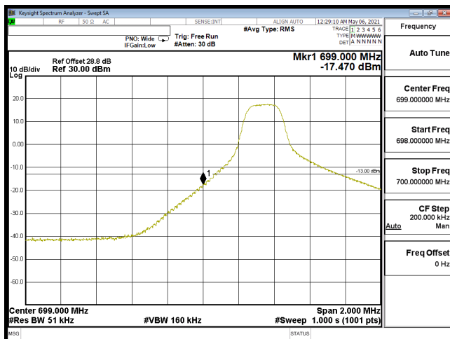
EDGE-B12_5M-CH23035-16QAM(1,0)
