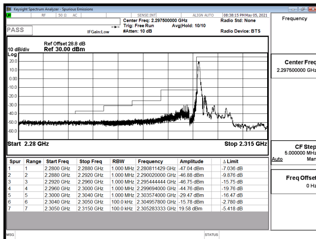
EDGE-B30_5M-CH27685-16QAM(1,0)
