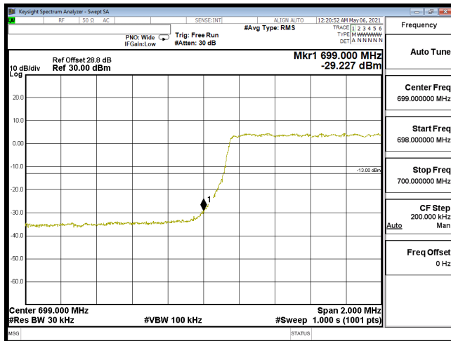
EDGE-B12_3M-CH23025-QPSK(15,0)
