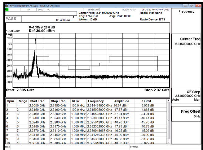
EDGE-B30_10M-CH27710-16QAM(1,49)
