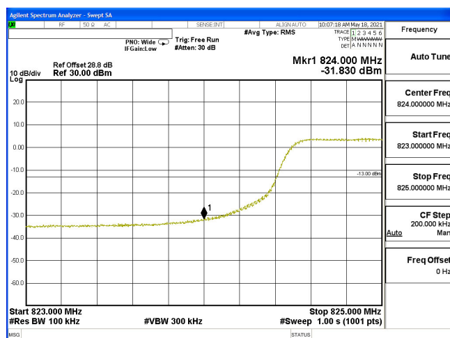
EDGE-B5_10M-CH20450-QPSK(50,0)
