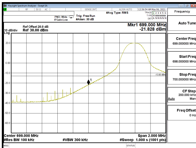
EDGE-B12_10M-CH23060-16QAM(1,0)
