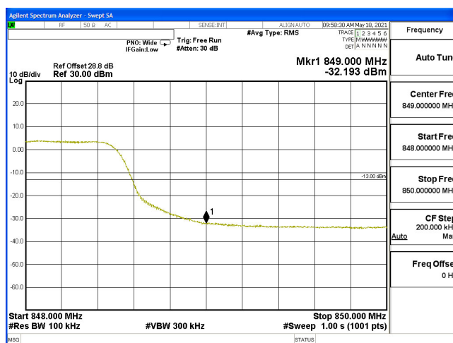
EDGE-B5_10M-CH20600-QPSK(50,0)
