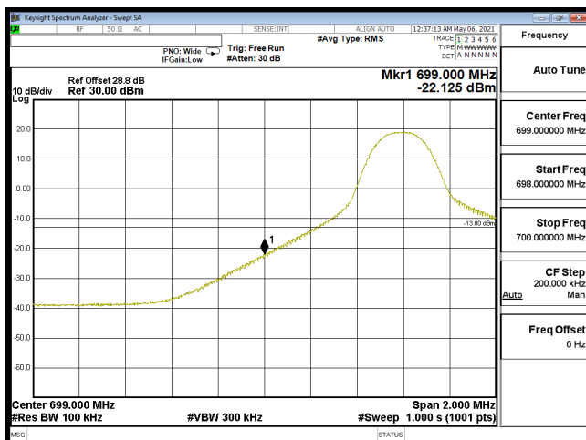
EDGE-B12_10M-CH23060-64QAM(1,0)
