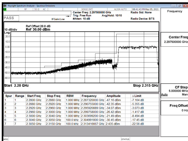
EDGE-B30_10M-CH27710-64QAM(50,0)
