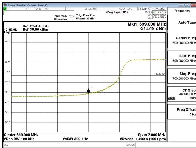
EDGE-B12_10M-CH23060-QPSK(50,0)
