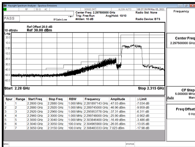
EDGE-B30_5M-CH27685-16QAM(25,0)
