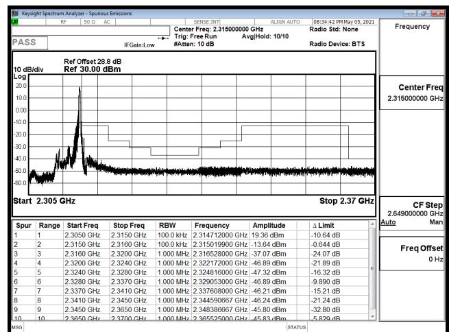
EDGE-B30_5M-CH27735-64QAM(1,24)
