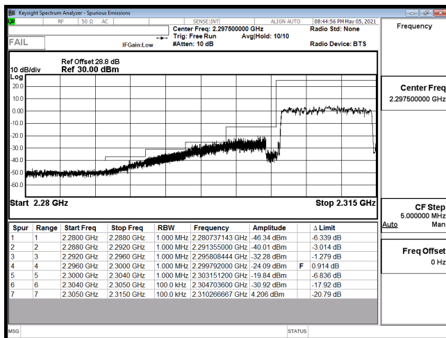
EDGE-B30_10M-CH27710-16QAM(50,0)
