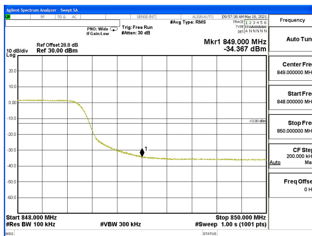
EDGE-B5_10M-CH20600-64QAM(50,0)
