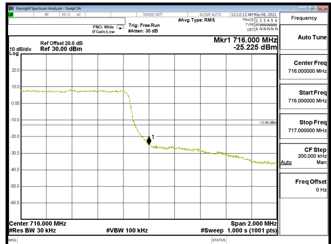
EDGE-B12_1.4M-CH23173-QPSK(6,0)
