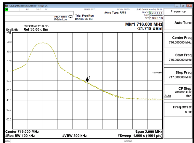
EDGE-B12_10M-CH23130-64QAM(1,49)
