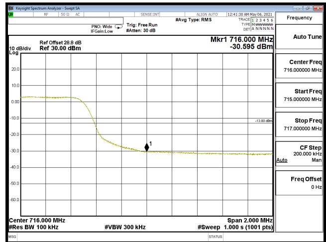
EDGE-B12_10M-CH23130-QPSK(50,0)
