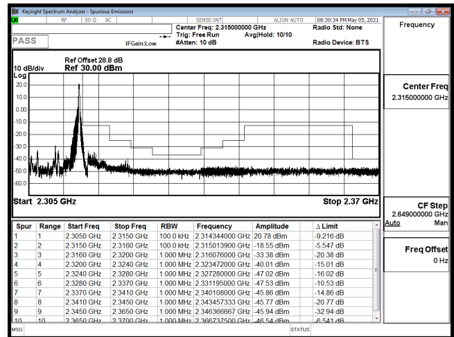
EDGE-B30_10M-CH27710-QPSK(1,49)
