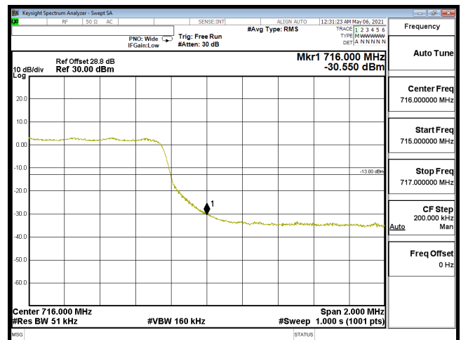
EDGE-B12_5M-CH23155-16QAM(25,0)
