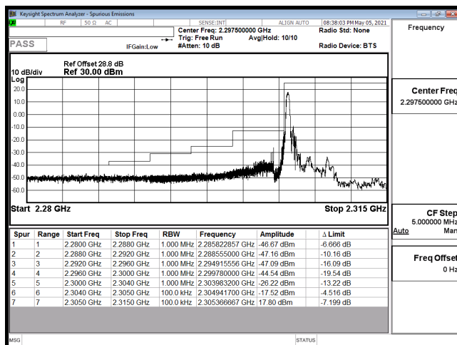
EDGE-B30_5M-CH27685-64QAM(1,0)
