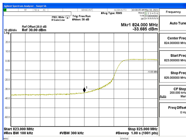
EDGE-B5_10M-CH20450-64QAM(50,0)
