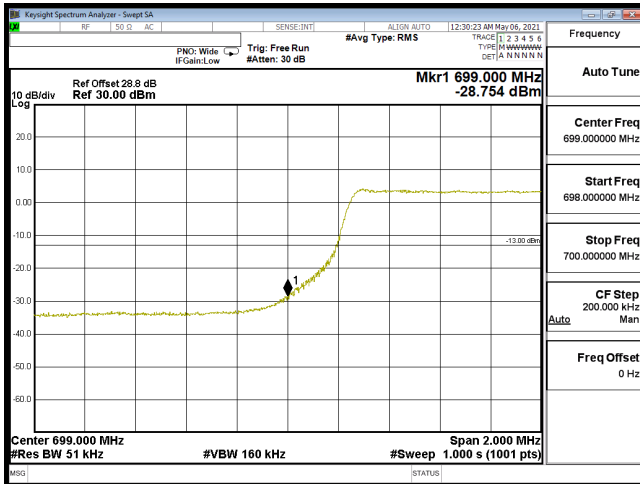
EDGE-B12_5M-CH23035-QPSK(25,0)
