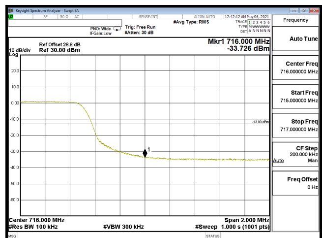
EDGE-B12_10M-CH23130-64QAM(50,0)
