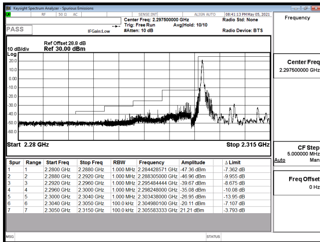
EDGE-B30_10M-CH27710-QPSK(1,0)
