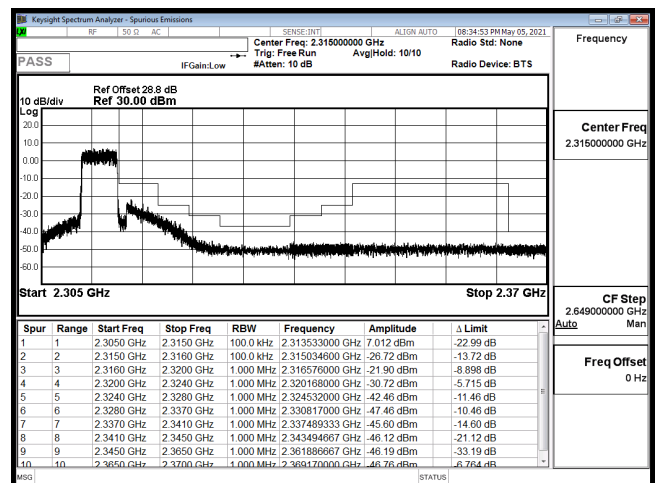
EDGE-B30_5M-CH27735-64QAM(25,0)
