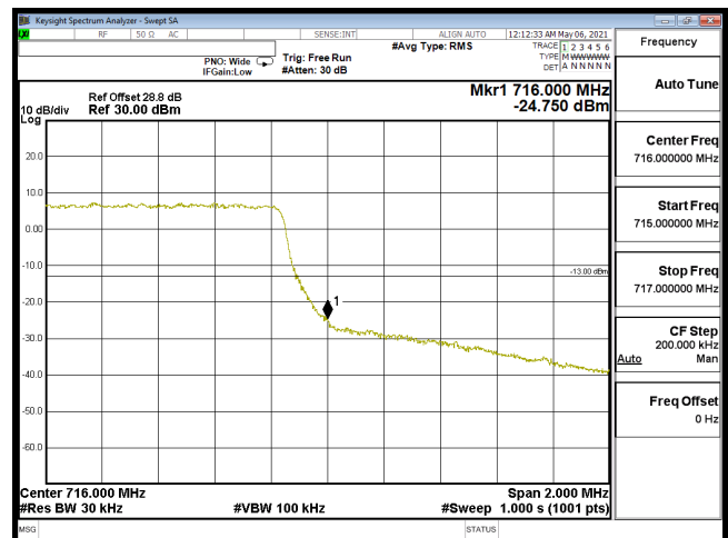
EDGE-B12_1.4M-CH23173-16QAM(6,0)
