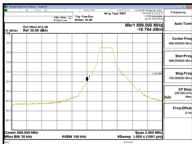
EDGE-B12_1.4M-CH23017-16QAM(1,0)
