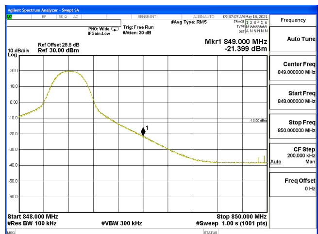
EDGE-B5_10M-CH20600-64QAM(1,49)
