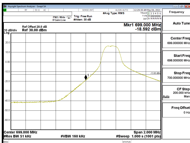
EDGE-B12_5M-CH23035-64QAM(1,0)
