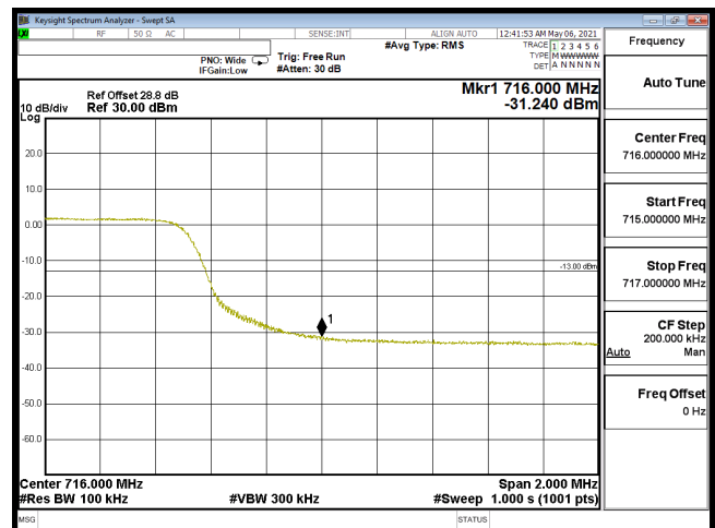
EDGE-B12_10M-CH23130-16QAM(50,0)
