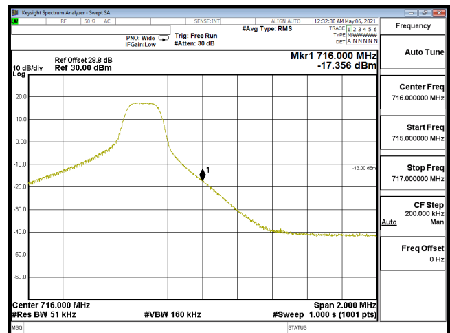
EDGE-B12_5M-CH23155-16QAM(1,24)
