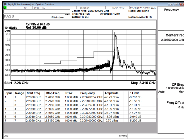
EDGE-B30_5M-CH27685-QPSK(1,0)
