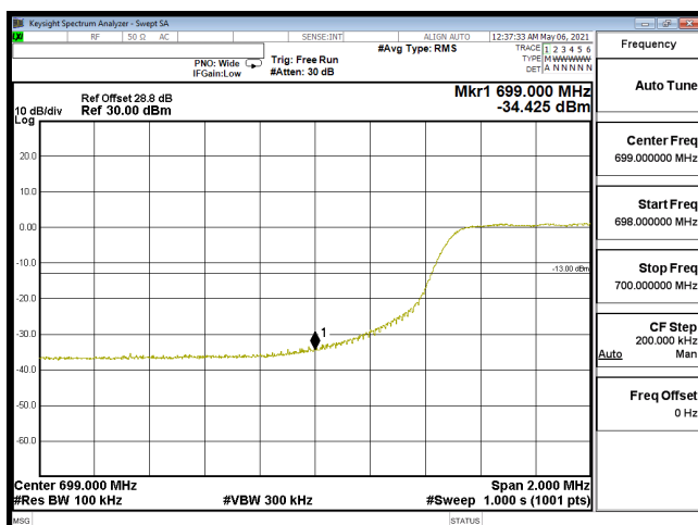
EDGE-B12_10M-CH23060-64QAM(50,0)
