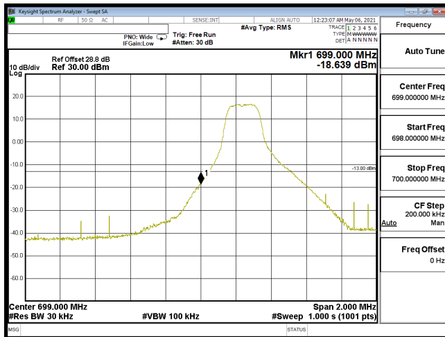
EDGE-B12_3M-CH23025-QPSK(1,0)
