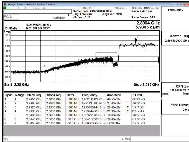
EDGE-B30_10M-CH27710-QPSK(50,0)
