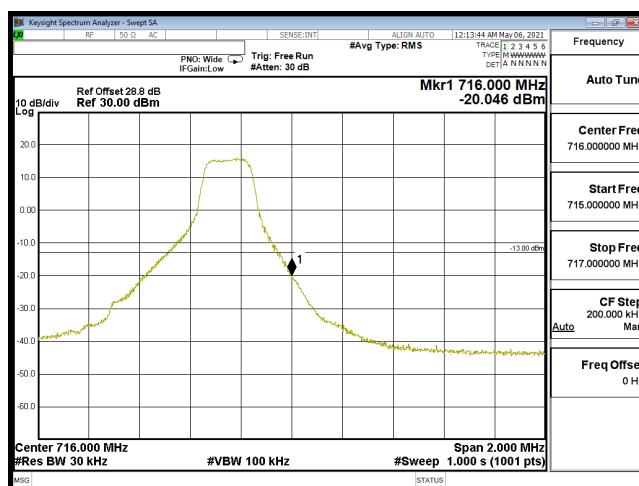
EDGE-B12_1.4M-CH23173-16QAM(1,5)
