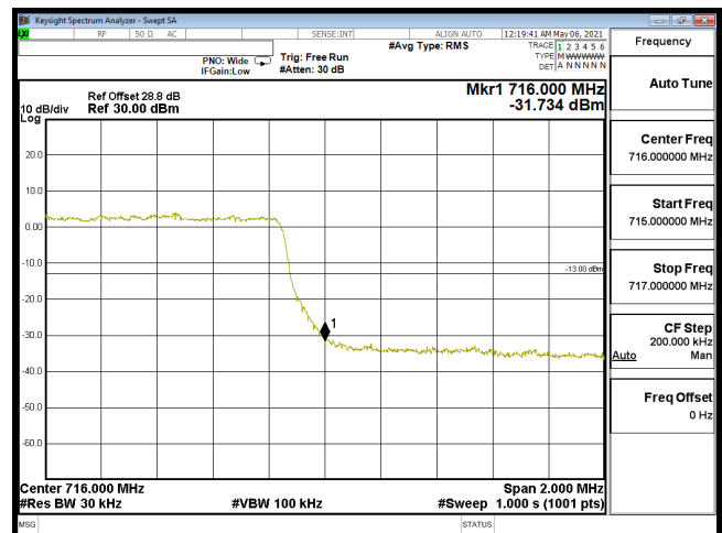
EDGE-B12_3M-CH23165-16QAM(15,0)
