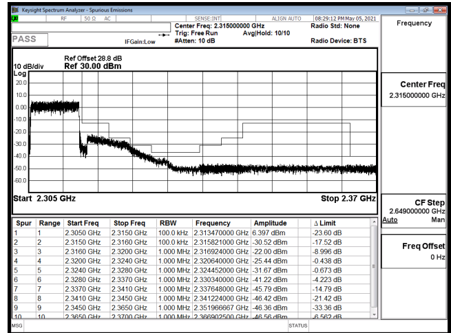
EDGE-B30_10M-CH27710-QPSK(50,0)
