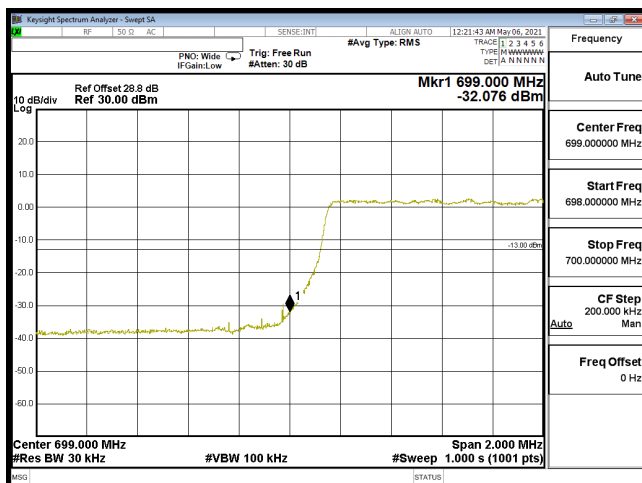
EDGE-B12_3M-CH23025-64QAM(15,0)
