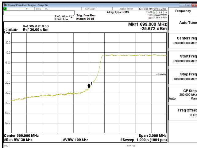
EDGE-B12_1.4M-CH23017-QPSK(6,0)
