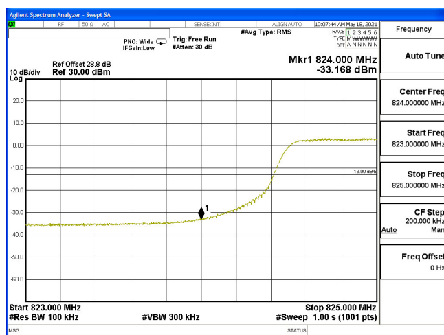
EDGE-B5_10M-CH20450-16QAM(50,0)
