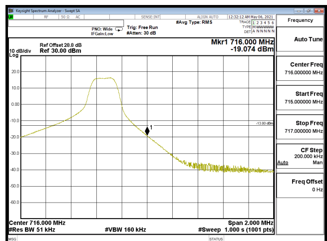
EDGE-B12_5M-CH23155-64QAM(1,24)
