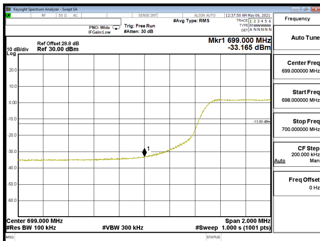
EDGE-B12_10M-CH23060-16QAM(50,0)
