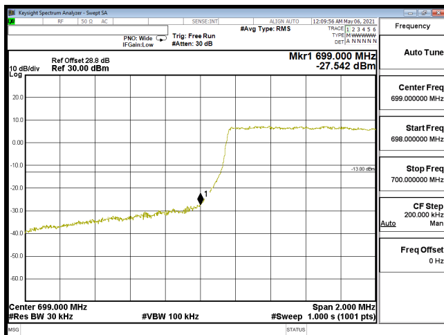
EDGE-B12_1.4M-CH23017-16QAM(6,0)
