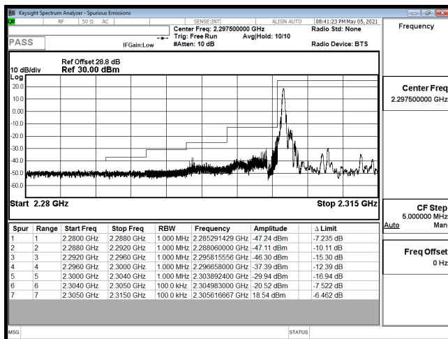
EDGE-B30_10M-CH27710-16QAM(1,0)
