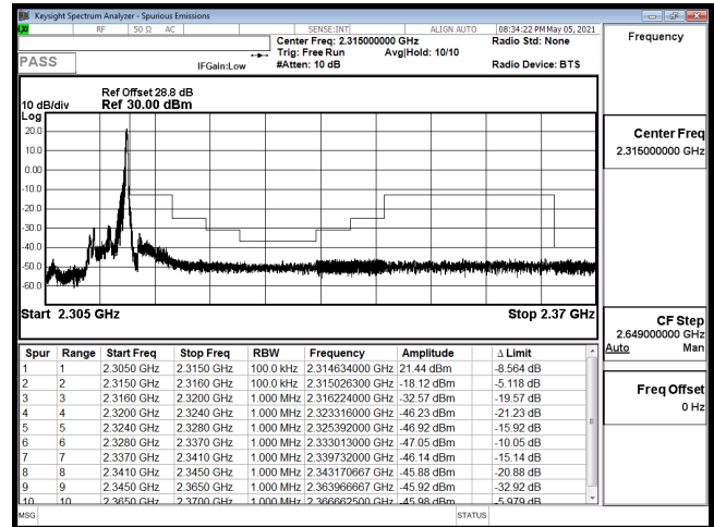
EDGE-B30_5M-CH27735-QPSK(1,24)
