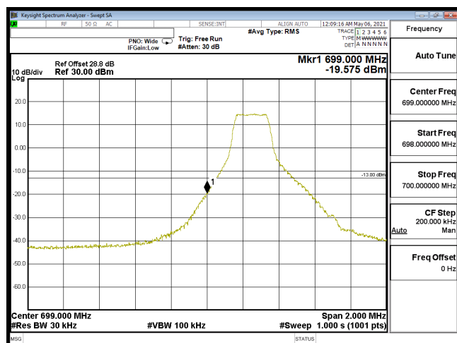
EDGE-B12_1.4M-CH23017-64QAM(1,0)
