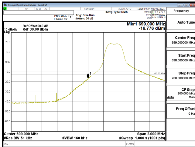
EDGE-B12_5M-CH23035-QPSK(1,0)
