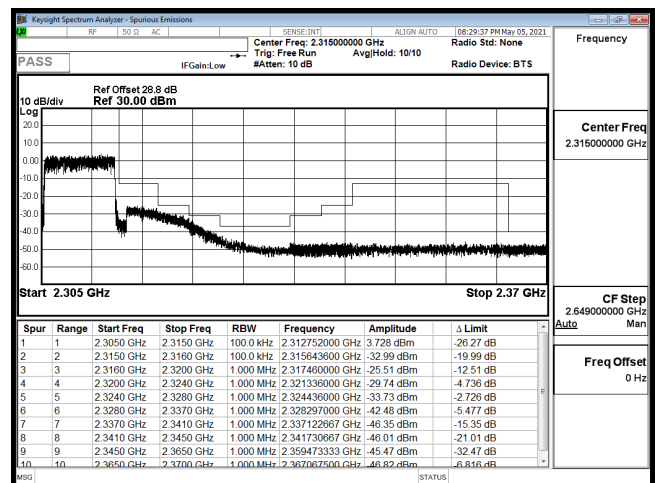
EDGE-B30_10M-CH27710-64QAM(50,0)
