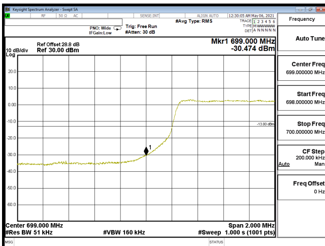
EDGE-B12_5M-CH23035-16QAM(25,0)
