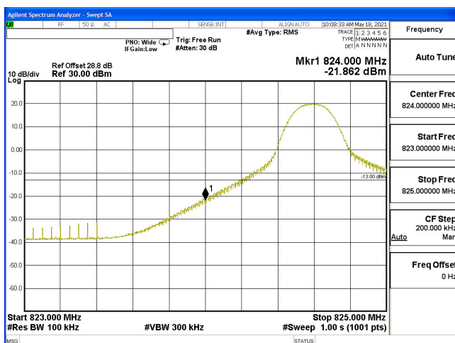
EDGE-B5_10M-CH20450-64QAM(1,0)
