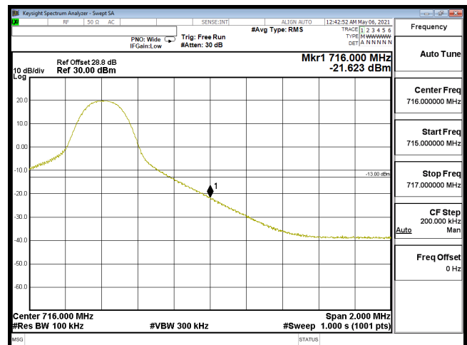
EDGE-B12_10M-CH23130-16QAM(1,49)
