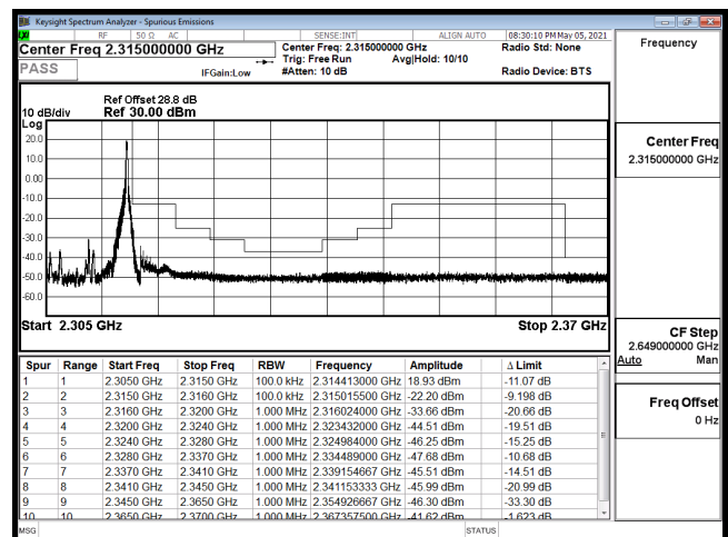
EDGE-B30_10M-CH27710-64QAM(1,49)
