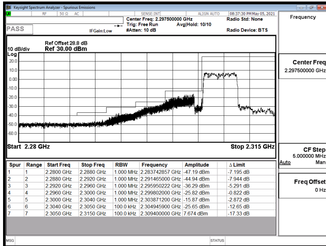
EDGE-B30_5M-CH27685-QPSK(25,0)
