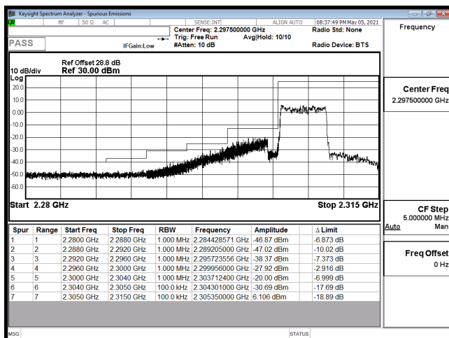
EDGE-B30_5M-CH27685-64QAM(25,0)
