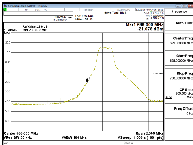
EDGE-B12_3M-CH23025-64QAM(1,0)
