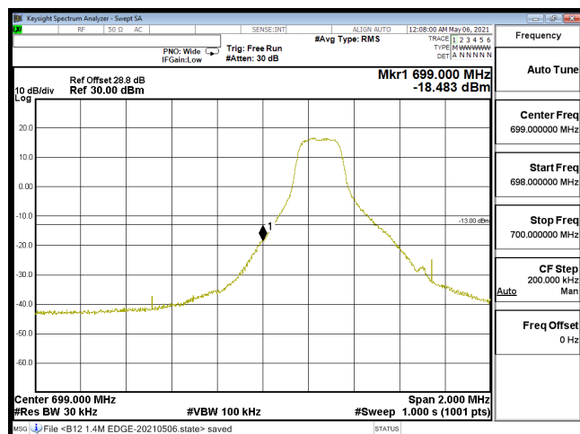
EDGE-B12_1.4M-CH23017-QPSK(1,0)
