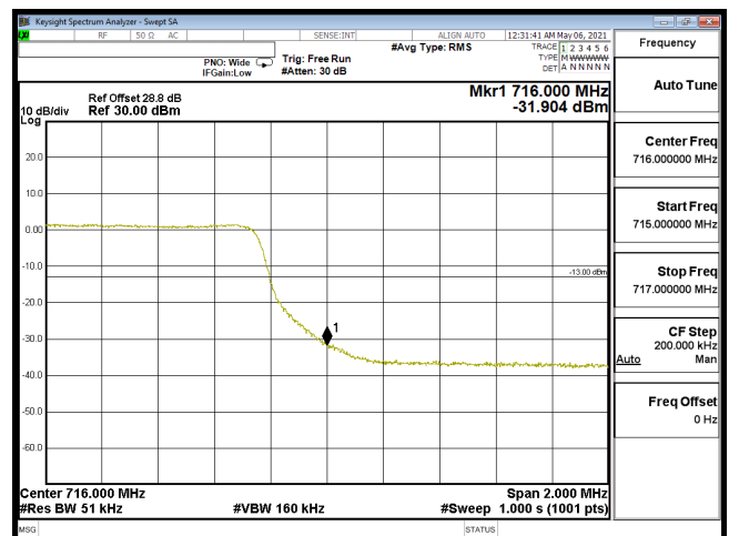
EDGE-B12_5M-CH23155-64QAM(25,0)
