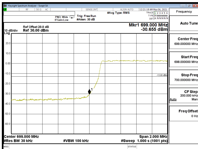
EDGE-B12_3M-CH23025-16QAM(15,0)
