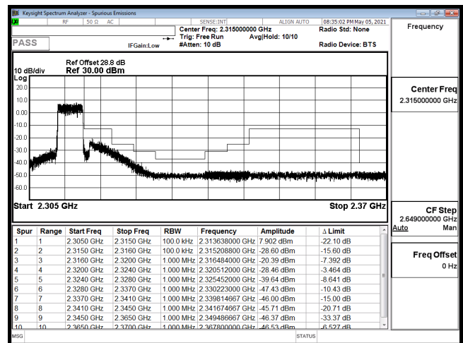
EDGE-B30_5M-CH27735-16QAM(25,0)
