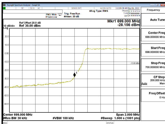
EDGE-B12_1.4M-CH23017-64QAM(6,0)
