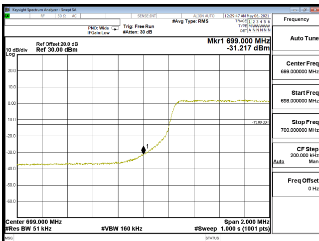
EDGE-B12_5M-CH23035-64QAM(25,0)
