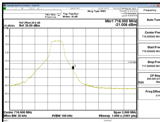
EDGE-B12_1.4M-CH23173-64QAM(1,5)
