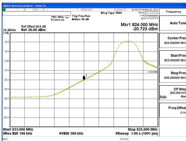
EDGE-B5_10M-CH20450-16QAM(1,0)
