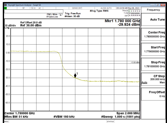
EDGE-B66_5M-CH132647-64QAM(25,0)
