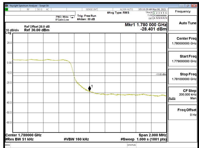
EDGE-B66_5M-CH132647-16QAM(25,0)
