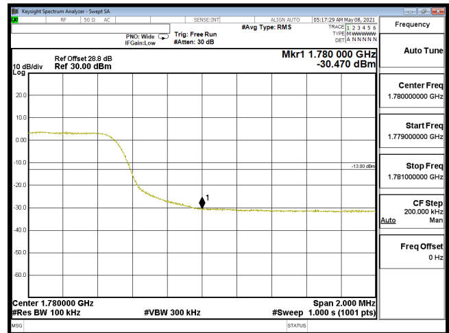
EDGE-B66_10M-CH132622-QPSK(50,0)
