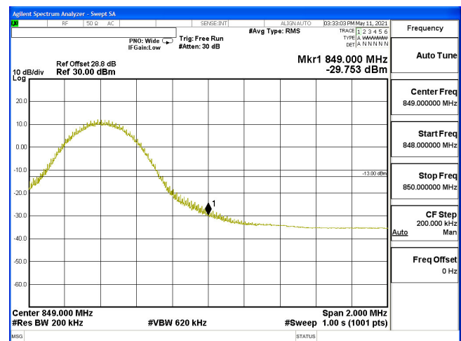
EDGE(10M+10M)-2ULCA_5B-16QAM_834.1(1,0)+844(1,49)
