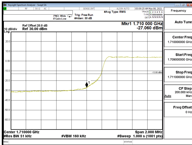
EDGE-B66_5M-CH131997-QPSK(25,0)
