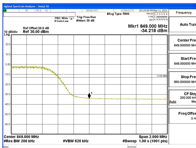
EDGE(10M+10M)-2ULCA_5B-16QAM_834.1(50,0)+844(50,0)
