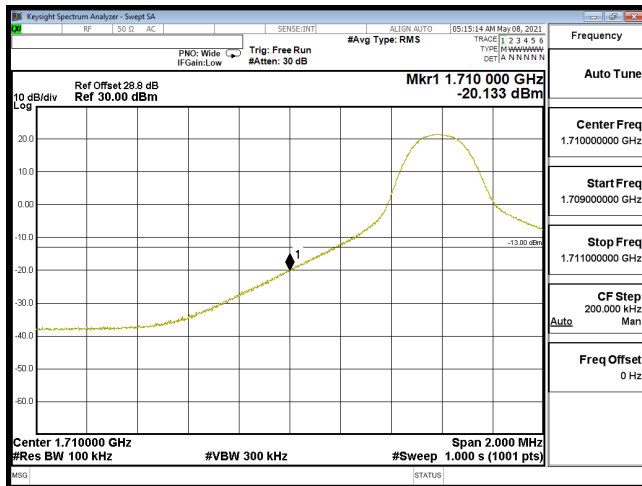
EDGE-B66_10M-CH132022-QPSK(1,0)
