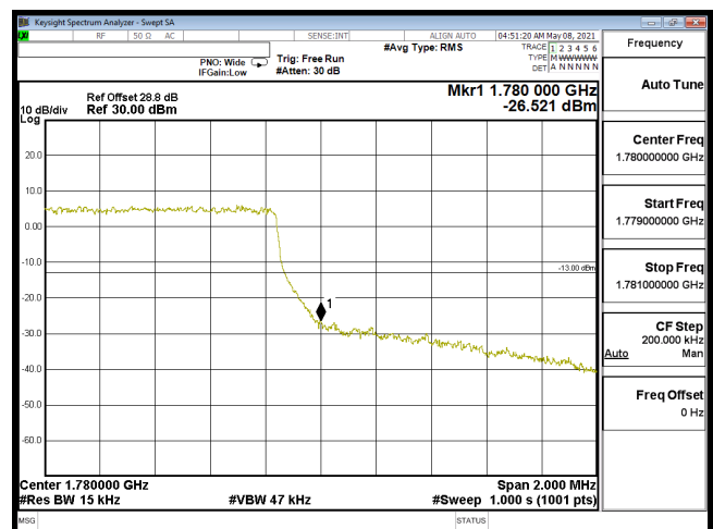
EDGE-B66_1.4M-CH132665-16QAM(6,0)
