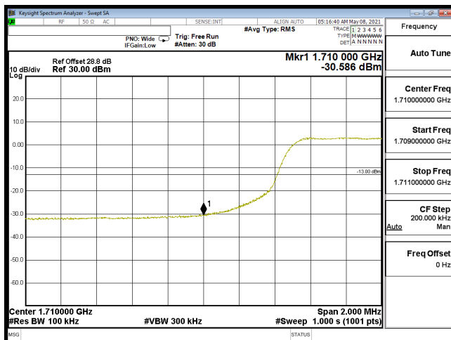
EDGE-B66_10M-CH132022-16QAM(50,0)
