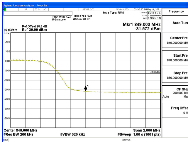
EDGE(10M+10M)-2ULCA_5B-QPSK_834.1(50,0)+844(50,0)
