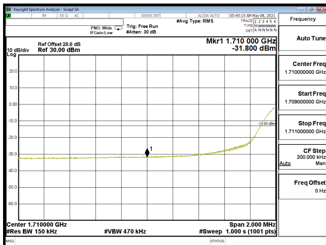
EDGE-B66_20M-CH132072-16QAM(100,0)
