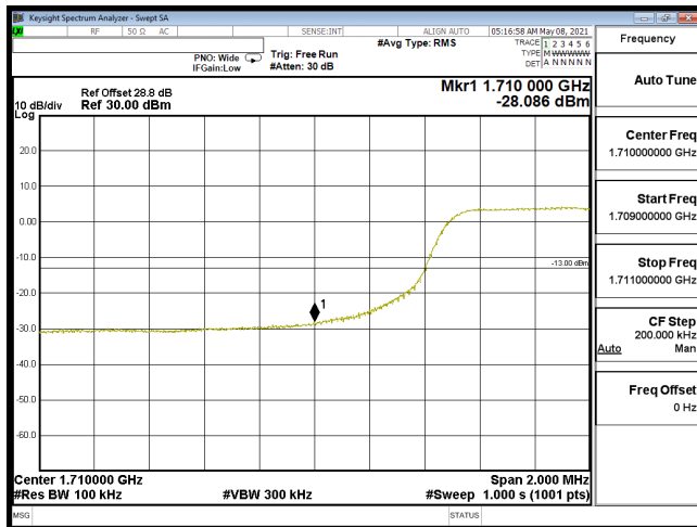
EDGE-B66_10M-CH132022-QPSK(50,0)
