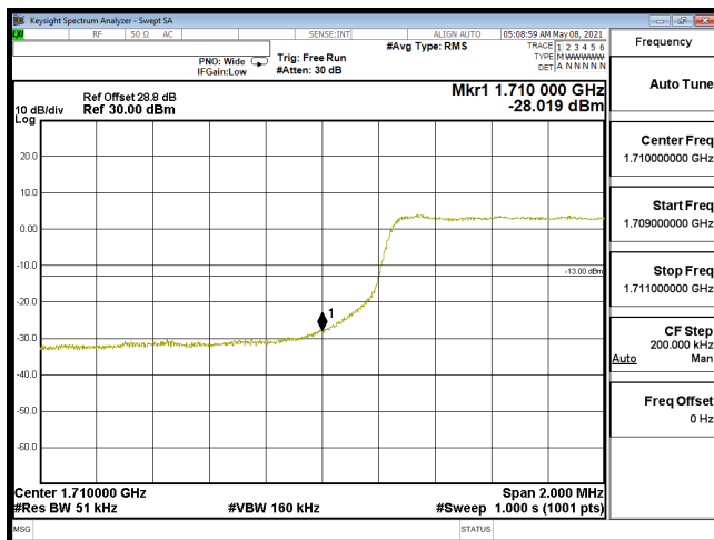
EDGE-B66_5M-CH131997-16QAM(25,0)
