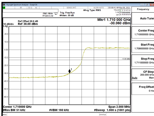
EDGE-B66_5M-CH131997-64QAM(25,0)
