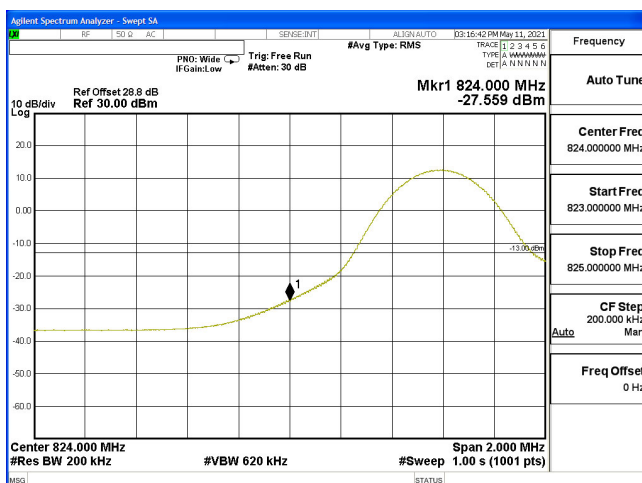
EDGE(10M+10M)-2ULCA_5B-64QAM_829(1,0)+838.9(1,49)
