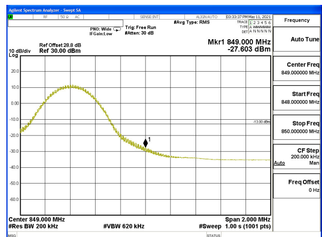
EDGE(10M+10M)-2ULCA_5B-64QAM_834.1(1,0)+844(1,49)
