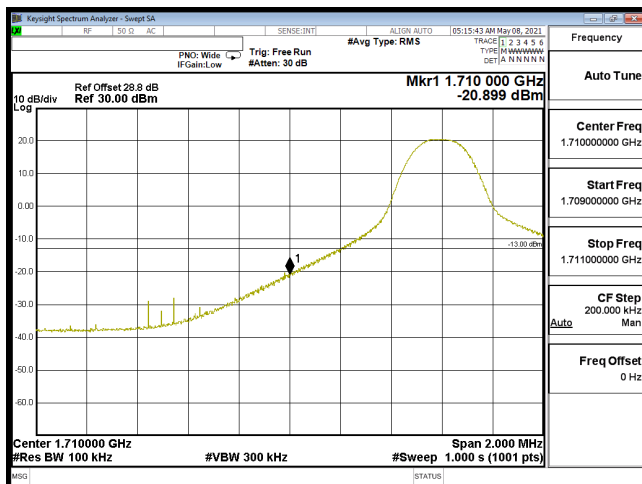
EDGE-B66_10M-CH132022-16QAM(1,0)
