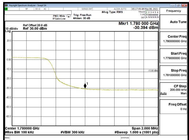
EDGE-B66_10M-CH132622-16QAM(50,0)
