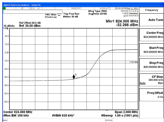
EDGE(10M+10M)-2ULCA_5B-64QAM_829(50,0)+838.9(50,0)
