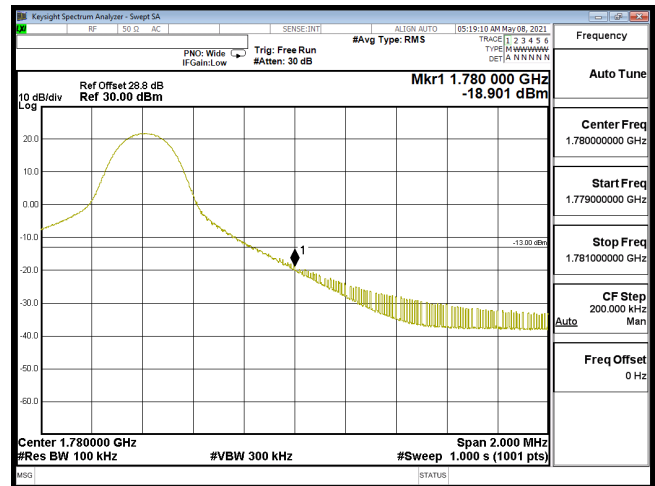
EDGE-B66_10M-CH132622-QPSK(1,49)
