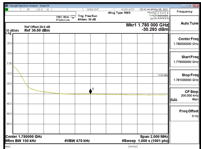
EDGE-B66_20M-CH132572-16QAM(100,0)
