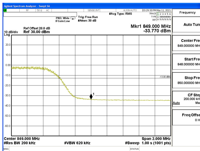
EDGE(10M+10M)-2ULCA_5B-64QAM_834.1(50,0)+844(50,0)
