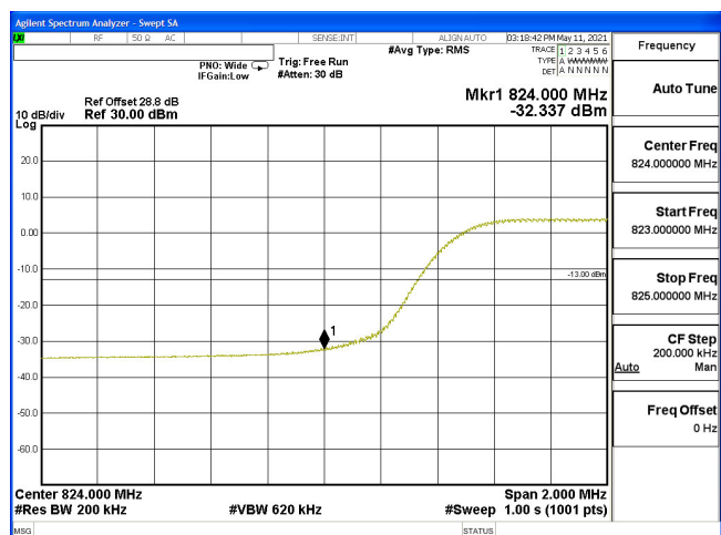
EDGE(10M+10M)-2ULCA_5B-16QAM_829(50,0)+838.9(50,0)
