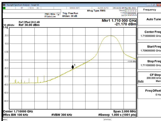
EDGE-B66_10M-CH132022-64QAM(1,0)
