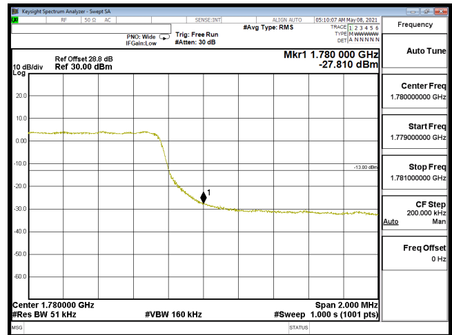
EDGE-B66_5M-CH132647-QPSK(25,0)
