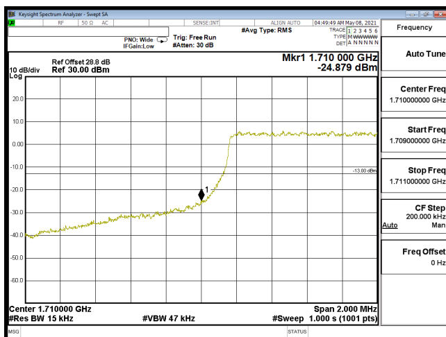
EDGE-B66_1.4M-CH131979-16QAM(6,0)
