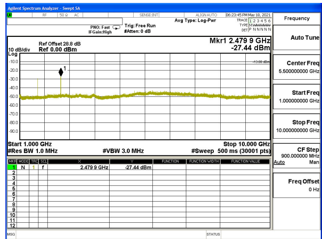
CSE-B5_5M-CH20425-QPSK(1,12)-1G-10G
