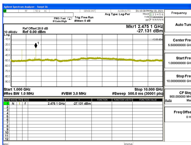
CSE-B5_1.4M-CH20407-16QAM(1,5)-1G-10G
