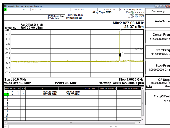
CSE-B5_1.4M-CH20407-16QAM(1,5)-30M-1G
