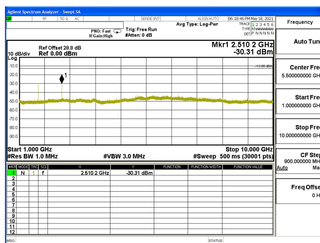
CSE-B5 3M-CH20525-QPSK(1,7)-1G-10G
