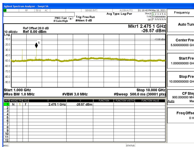
CSE-B5_1.4M-CH20407-QPSK(3,3)-1G-10G
