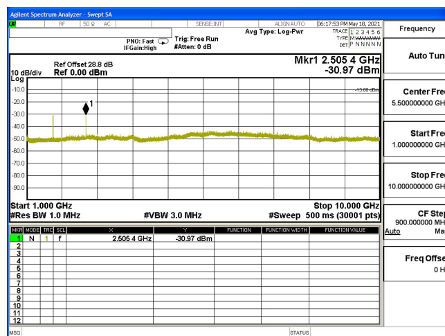
CSE-B5_3M-CH20525-64QAM(1,0)-1G-10G
