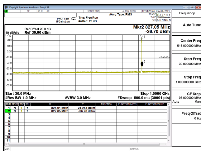
CSE-B5_1.4M-CH20407-64QAM(3,3)-30M-1G
