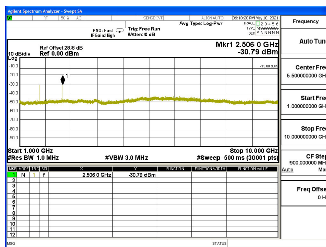
CSE-B5_3M-CH20525-16QAM(1,0)-1G-10G
