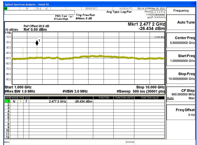
CSE-B5_3M-CH20415-QPSK(1,7)-1G-10G
