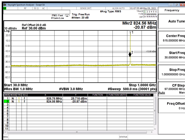
CSE-B5_5M-CH20425-QPSK(1,12)-30M-1G
