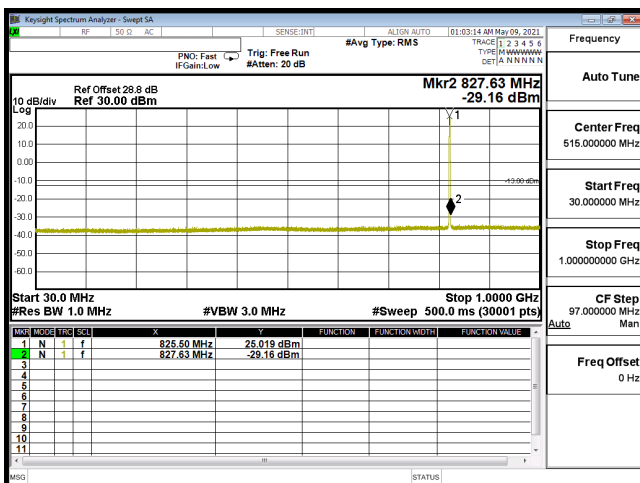
CSE-B5_3M-CH20415-64QAM(1,7)-30M-1G
