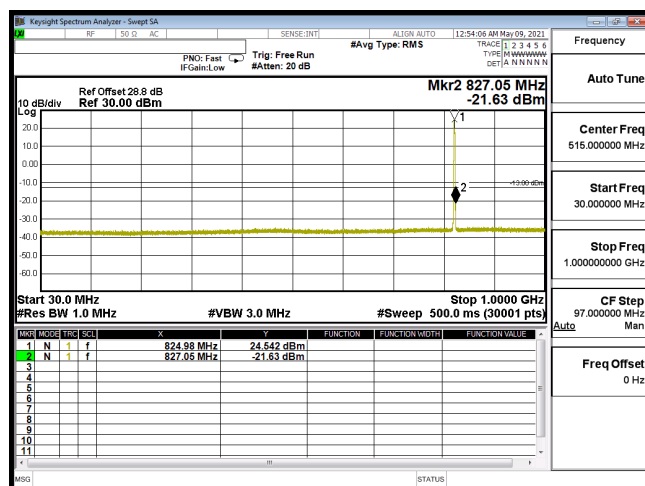
CSE-B5_1.4M-CH20407-QPSK(3,3)-30M-1G
