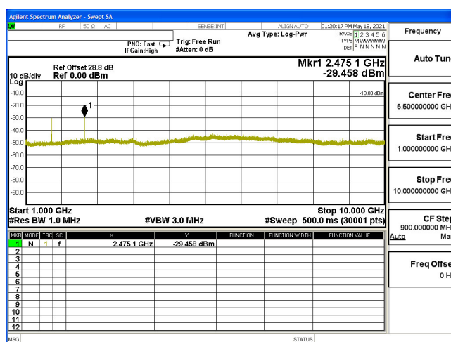
CSE-B5_1.4M-CH20407-64QAM(3,3)-1G-10G
