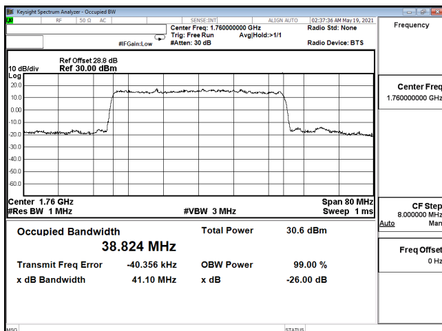
OCC-ENDC_12A_n66-PI2-BPSK_40M_CH352000_1760(216,0)
