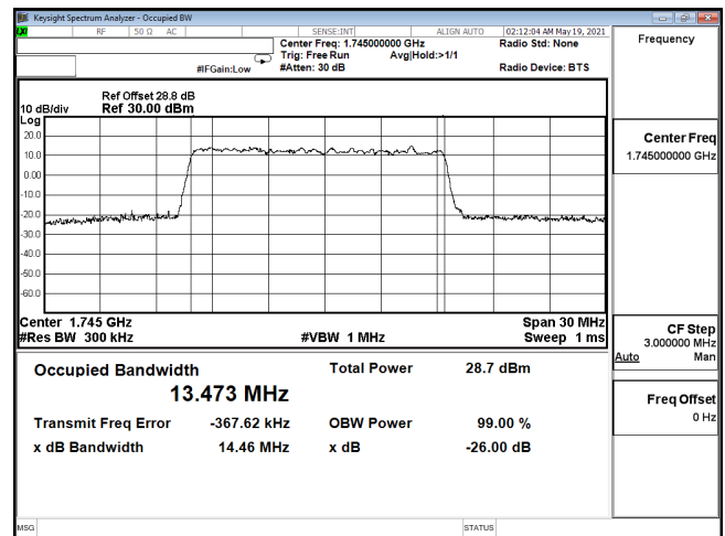
OCC-ENDC_12A_n66-16QAM_15M_CH349000_1745(75,0)
