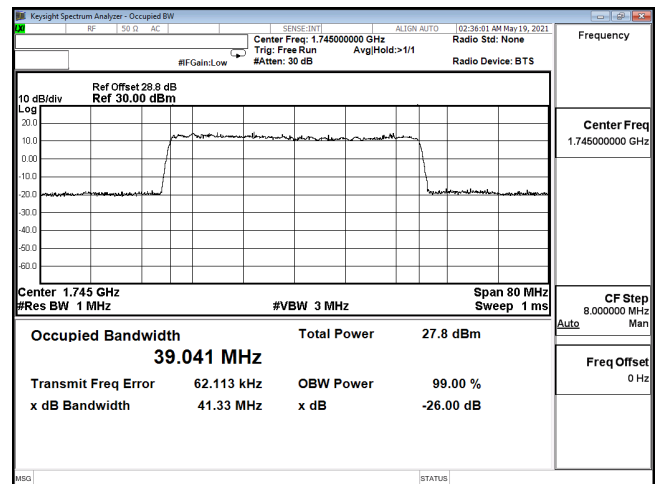
OCC-ENDC_12A_n66-256QAM_40M_CH349000_1745(216,0)
