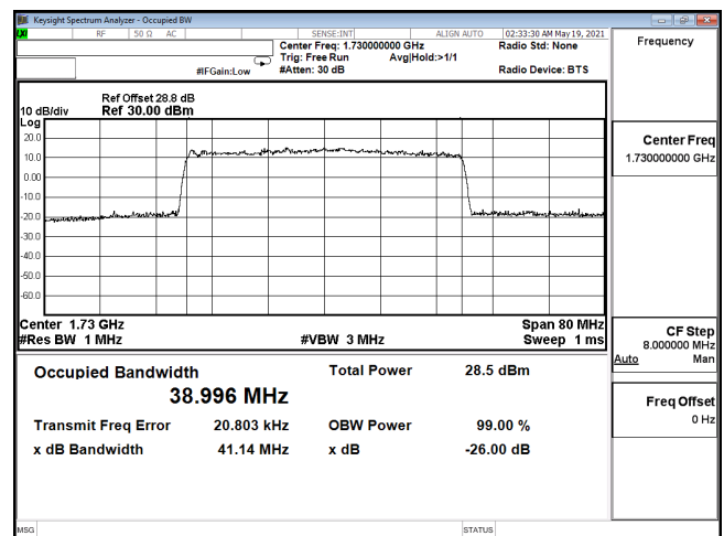
OCC-ENDC_12A_n66-64QAM_40M_CH346000_1730(216,0)
