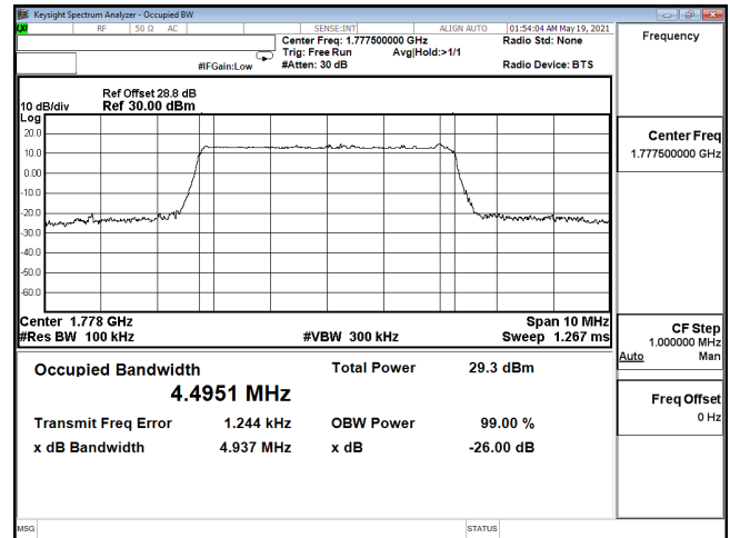
OCC-ENDC_12A_n66-64QAM_5M_CH355500_1777.5(25,0)
