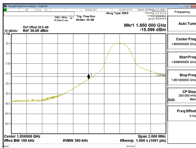
EDGE-ENDC_5A_n2-PI2-BPSK_10M_CH371000_1855(1,0)_SCS15KHz
