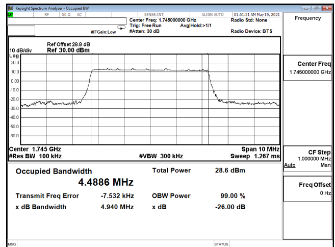
OCC-ENDC_12A_n66-256QAM_5M_CH349000_1745(25,0)
