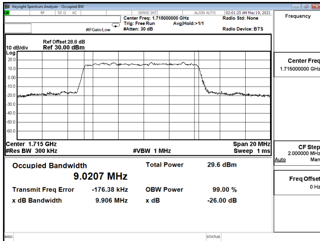
OCC-ENDC_12A_n66-64QAM_10M_CH343000_1715(50,0)
