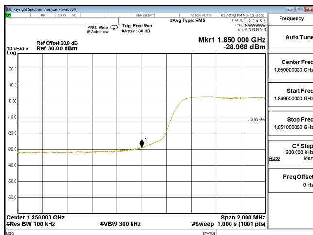
EDGE-ENDC_5A_n2-16QAM_10M_CH371000_1855(50,0)_SCS15KHz
