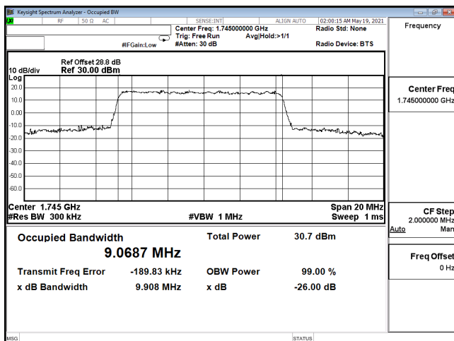
OCC-ENDC_12A_n66-16QAM_10M_CH349000_1745(50,0)
