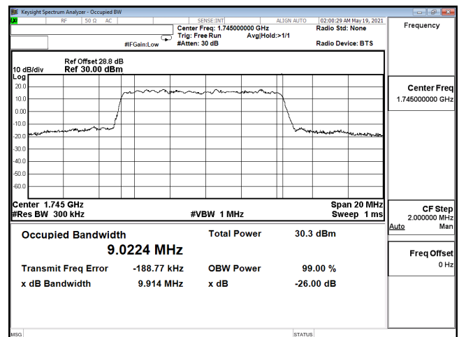
OCC-ENDC_12A_n66-64QAM_10M_CH349000_1745(50,0)
