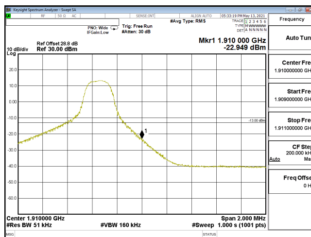
EDGE-ENDC_5A_n2-256QAM_5M_CH381500_1907.5(1,24)_SCS15KHz
