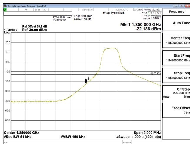
EDGE-ENDC_5A_n2-256QAM_5M_CH370500_1852.5(1,0)_SCS15KHz
