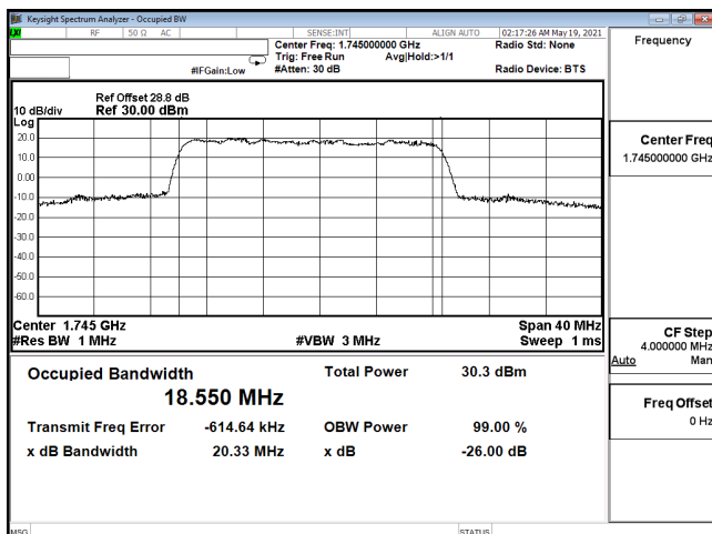
OCC-ENDC_12A_n66-16QAM_20M_CH349000_1745(100,0)
