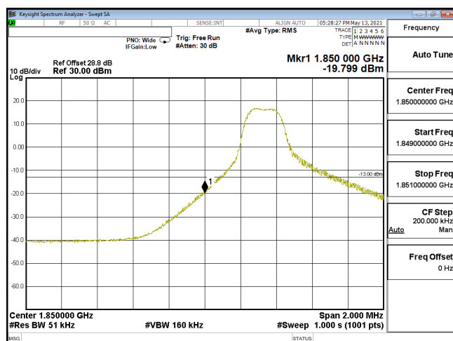
EDGE-ENDC_5A_n2-64QAM_5M_CH370500_1852.5(1,0)_SCS15KHz
