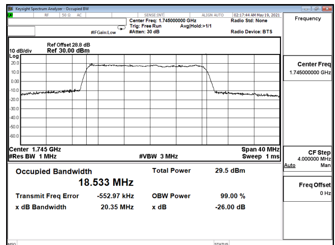
OCC-ENDC_12A_n66-64QAM_20M_CH349000_1745(100,0)
