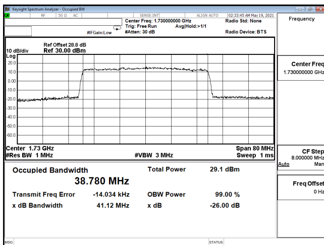
OCC-ENDC_12A_n66-16QAM_40M_CH346000_1730(216,0)
