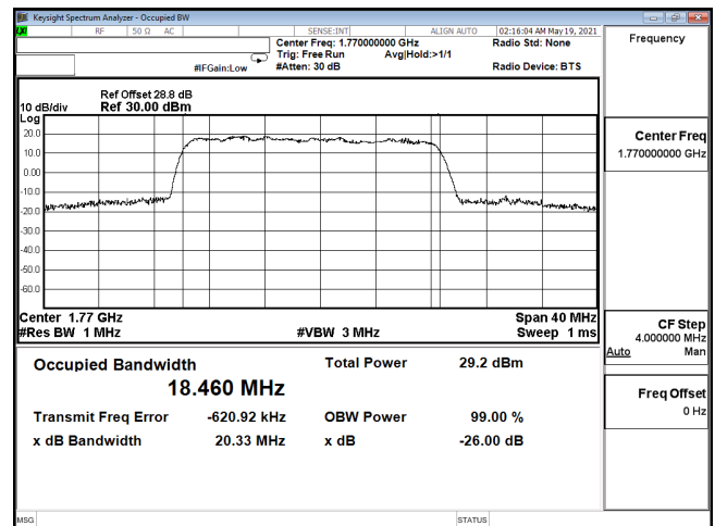
OCC-ENDC_12A_n66-16QAM_20M_CH354000_1770(100,0)
