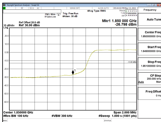
EDGE-ENDC_5A_n2-QPSK_10M_CH371000_1855(50,0)_SCS15KHz
