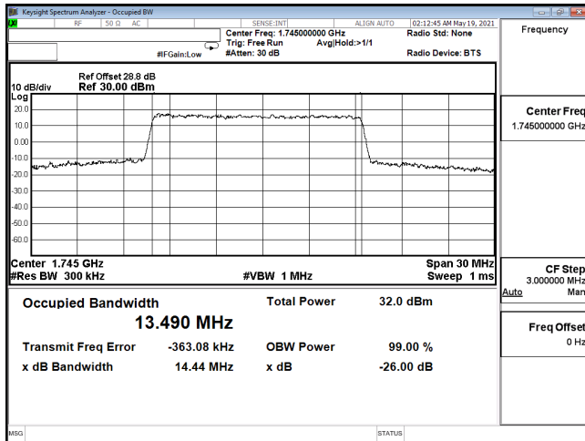
OCC-ENDC_12A_n66-QPSK_15M_CH349000_1745(75,0)
