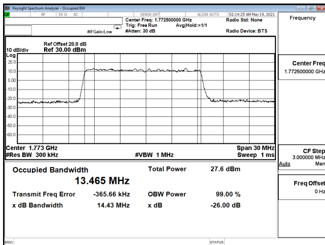
OCC-ENDC_12A_n66-256QAM_15M_CH354500_1772.5(75,0)
