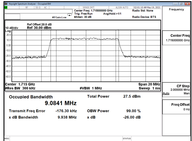
OCC-ENDC_12A_n66-256QAM_10M_CH343000_1715(50,0)
