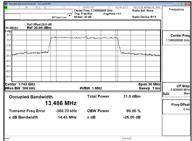
OCC-ENDC_12A_n66-16QAM_15M_CH349000_1745(75,0)
