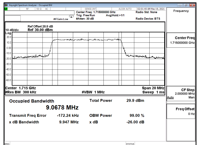
OCC-ENDC_12A_n66-16QAM_10M_CH343000_1715(50,0)
