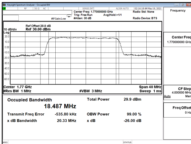
OCC-ENDC_12A_n66-QPSK_20M_CH354000_1770(100,0)
