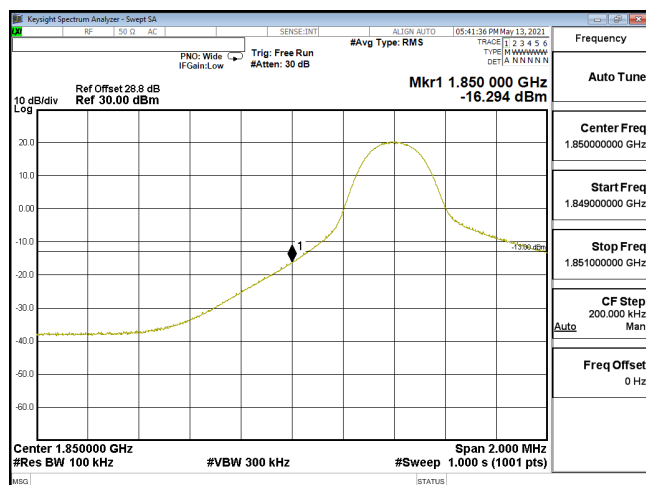
EDGE-ENDC_5A_n2-QPSK_10M_CH371000_1855(1,0)_SCS15KHz
