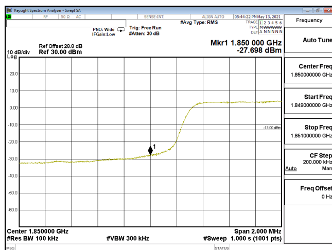
EDGE-ENDC_5A_n2-PI2-BPSK_10M_CH371000_1855(50,0)_SCS15KHz
