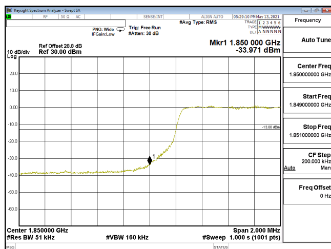
EDGE-ENDC_5A_n2-256QAM_5M_CH370500_1852.5(25,0)_SCS15KHz
