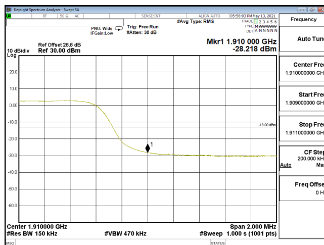
EDGE-ENDC_5A_n2-QPSK_15M_CH380500_1902.5(75,4)_SCS15KHz
