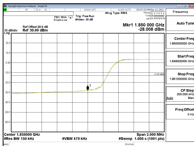
EDGE-ENDC_5A_n2-PI2-BPSK_15M_CH371500_1857.5(75,0)_SCS15KHz
