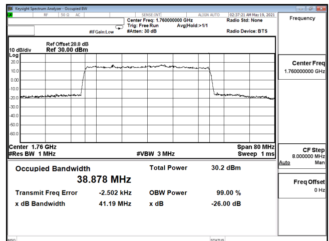
OCC-ENDC_12A_n66-QPSK_40M_CH352000_1760(216,0)
