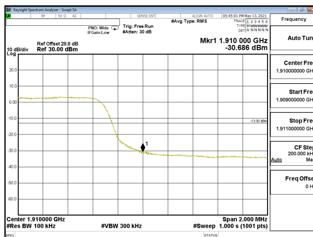
EDGE-ENDC_5A_n2-PI2-BPSK_10M_CH381000_1855(50,2)_SCS15KHz
