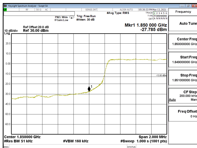
EDGE-ENDC_5A_n2-PI2-BPSK_5M_CH370500_1852.5(25,0)_SCS15KHz
