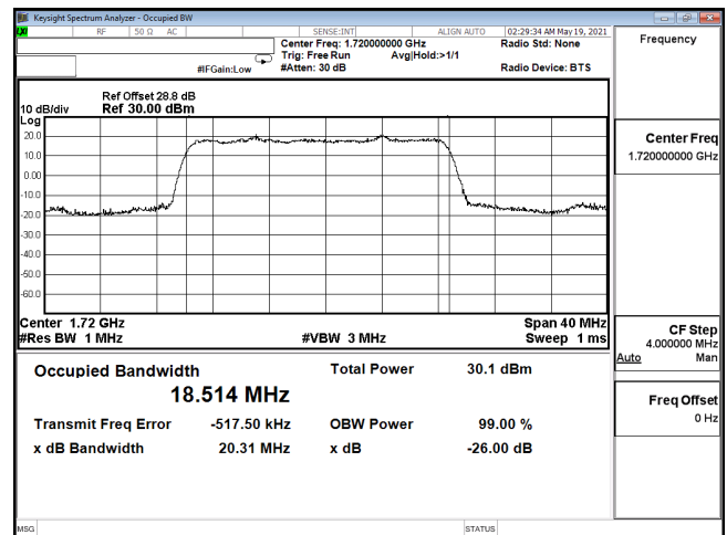
OCC-ENDC_12A_n66-PI2-BPSK_20M_CH344000_1720(100,0)
