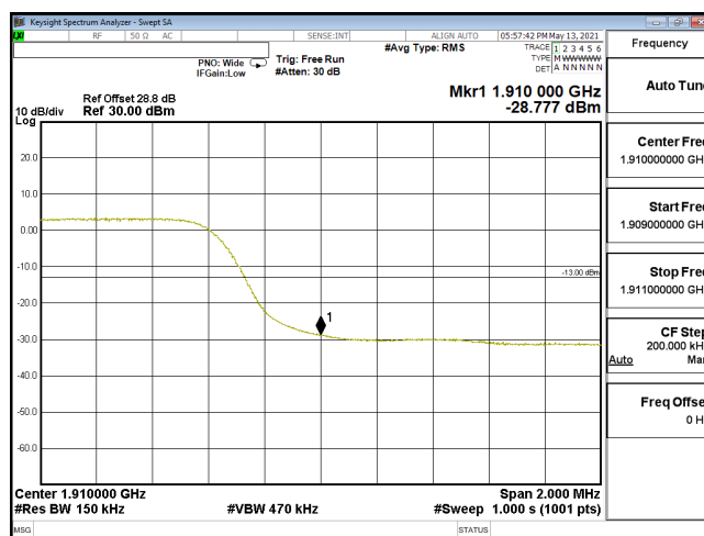
EDGE-ENDC_5A_n2-PI2-BPSK_15M_CH380500_1902.5(75,4)_SCS15KHz
