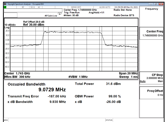
OCC-ENDC_12A_n66-QPSK_10M_CH349000_1745(50,0)
