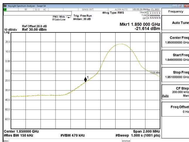
EDGE-ENDC_5A_n2-256QAM_15M_CH371500_1857.5(1,0)_SCS15KHz
