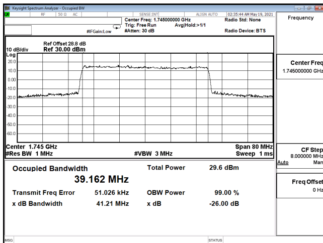
OCC-ENDC_12A_n66-64QAM_40M_CH349000_1745(216,0)
