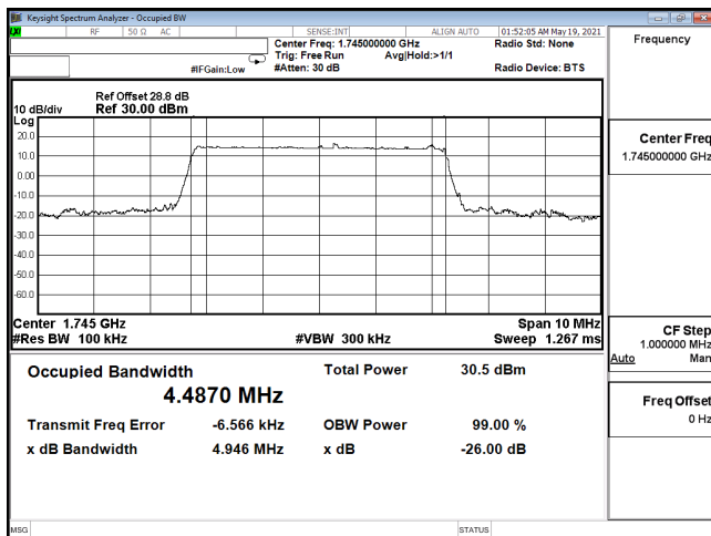
OCC-ENDC_12A_n66-64QAM_5M_CH349000_1745(25,0)
