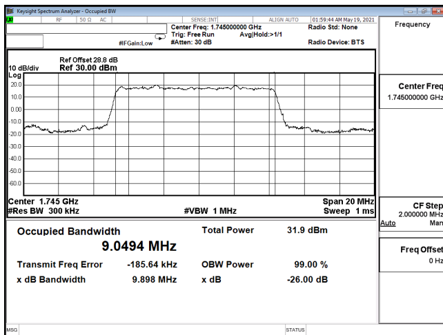
OCC-ENDC_12A_n66-PI2-BPSK_10M_CH349000_1745(50,0)
