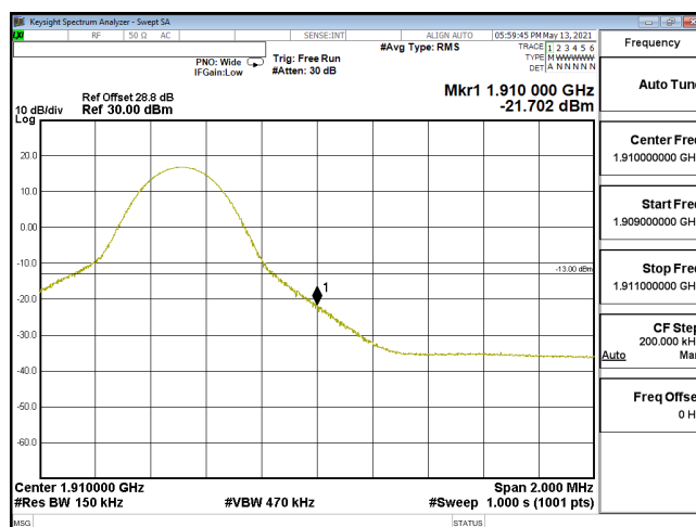
EDGE-ENDC_5A_n2-256QAM_15M_CH380500_1902.5(1,78)_SCS15KHz
