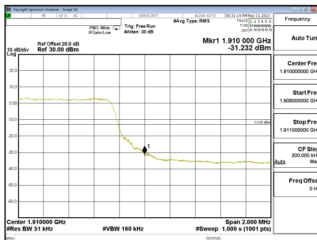
EDGE-ENDC_5A_n2-PI2-BPSK_5M_CH381500_1907.5(25,0)_SCS15KHz
