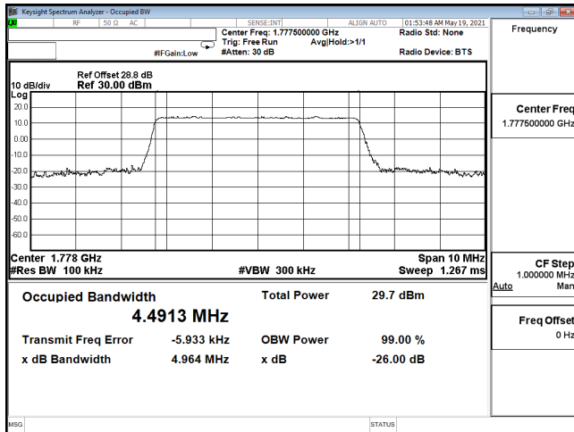
OCC-ENDC_12A_n66-16QAM_5M_CH355500_1777.5(25,0)
