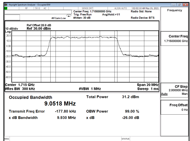
OCC-ENDC_12A_n66-PI2-BPSK_10M_CH343000_1715(50,0)
